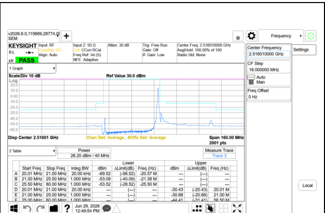
5G NR n41 40MHz BPSK Low Channel RB1-105 Ant14+Ant1
