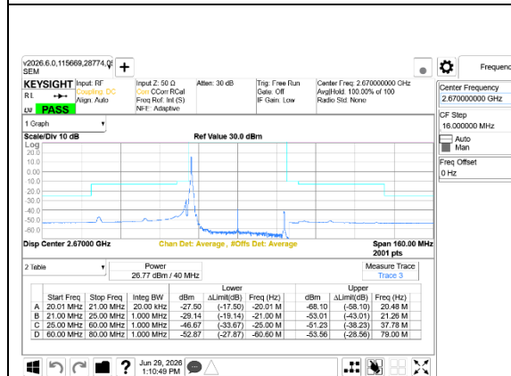
5G NR n41 40MHz BPSK High Channel RB1-0 Ant14+Ant1
