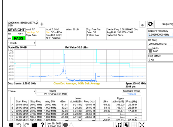
5G NR n41 50MHz BPSK Middle Channel RB1-0 Ant14+Ant1
