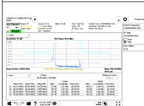
5G NR n41 50MHz BPSK High Channel RB1-0 Ant14+Ant1
