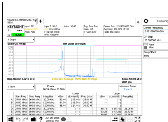
5G NR n41 50MHz BPSK Low Channel RB1-0 Ant14+Ant1
