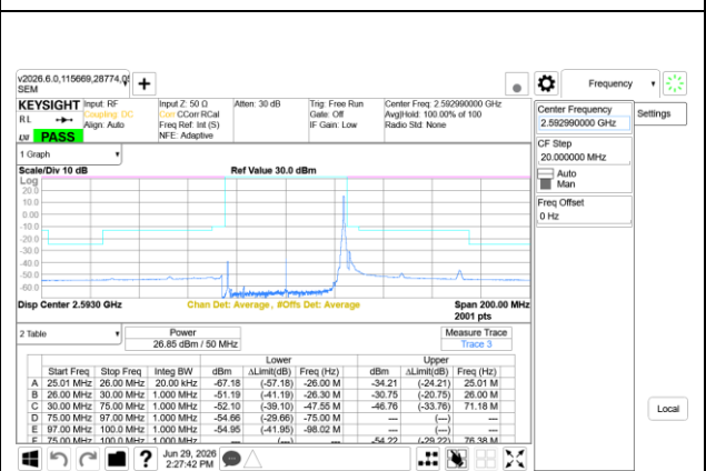
5G NR n41 50MHz BPSK Middle Channel RB1-132 Ant14+Ant1
