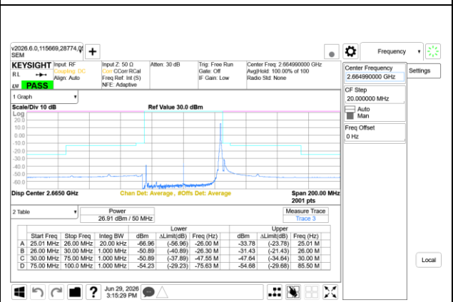
5G NR n41 50MHz BPSK High Channel RB1-132 Ant14+Ant1
