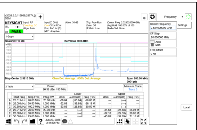
5G NR n41 50MHz BPSK Low Channel RB1-132 Ant14+Ant1
