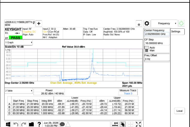
5G NR n41 40MHz BPSK Middle Channel RB1-105 Ant14+Ant1
