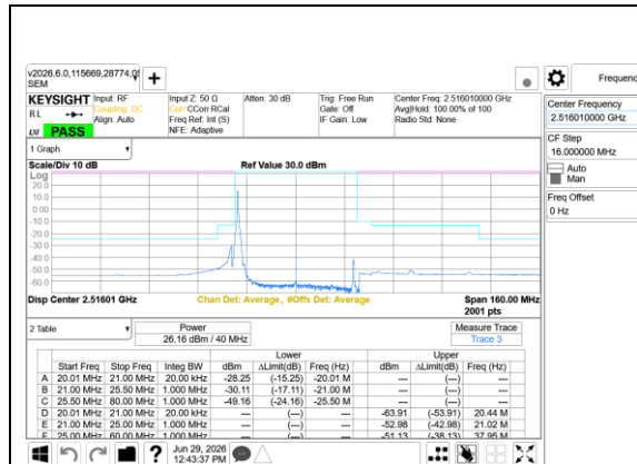
5G NR n41 40MHz BPSK Low Channel RB1-0 Ant14+Ant1
