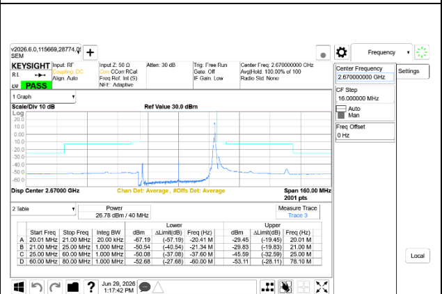
5G NR n41 40MHz BPSK High Channel RB1-105 Ant14+Ant1
