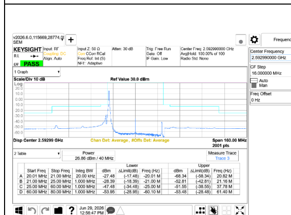
5G NR n41 40MHz BPSK Middle Channel RB1-0 Ant14+Ant1
