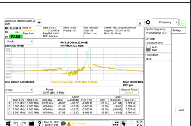
LTE B41 5MHz QPSK Middle Channel RB1-24
