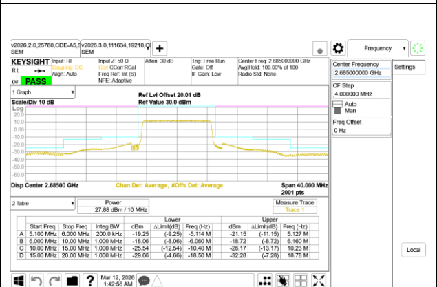
LTE B41 10MHz QPSK High Channel RB50-0
