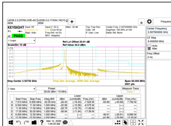
LTE B41 15MHz QPSK Low Channel RB1-0
