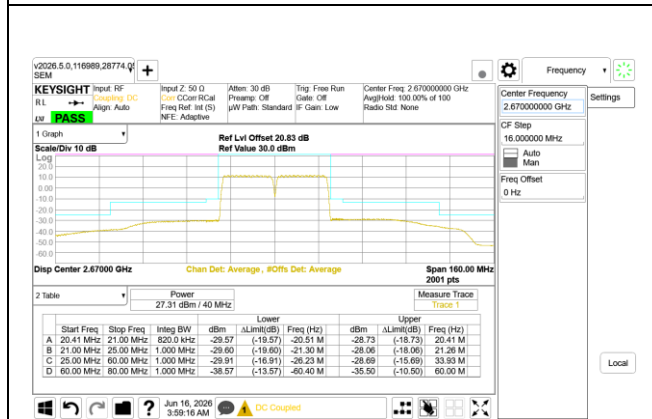
ULCA LTE B41 20MHz + 20MHz QPSK High Ch RB100-0 + RB100-0
