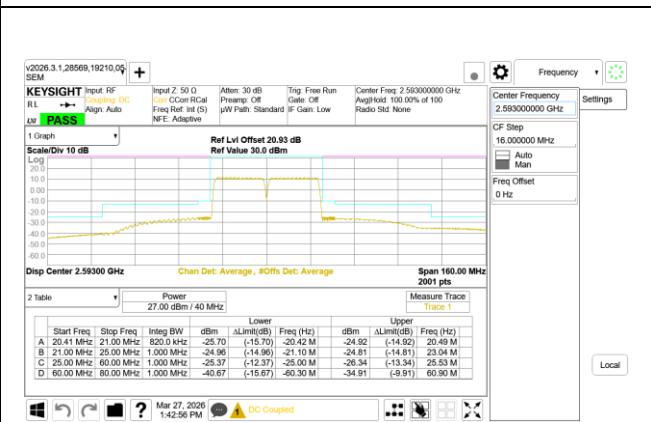
ULCA LTE B41 20MHz + 20MHz 16QAM Mid Ch RB100-0 + RB100-0
