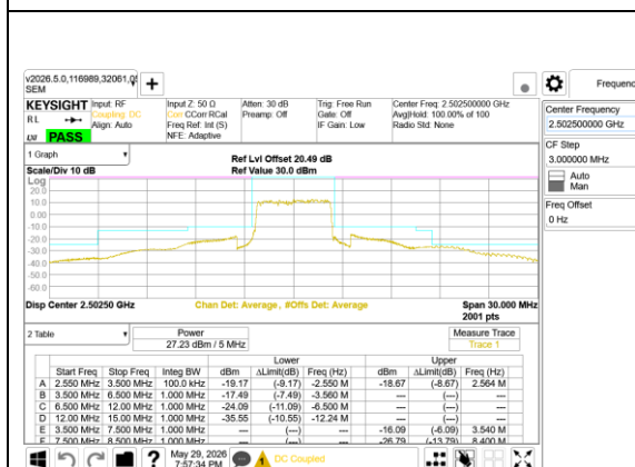
LTE B41 5MHz QPSK Low Channel RB25-0
