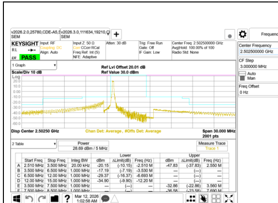
LTE B41 5MHz QPSK Low Channel RB1-0
