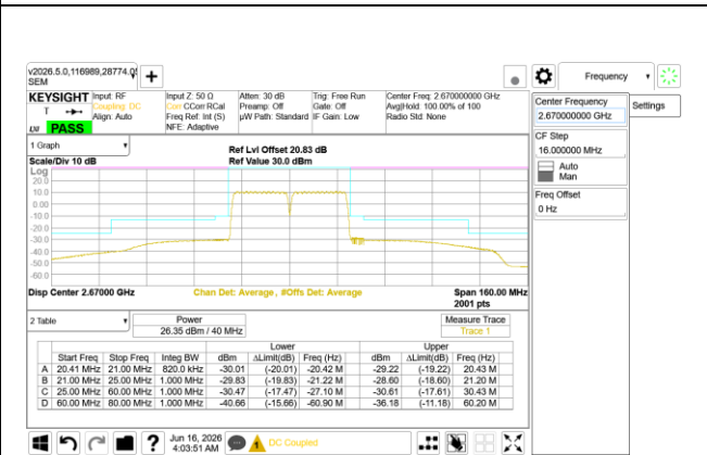
ULCA LTE B41 20MHz + 20MHz 16QAM High Ch RB100-0 + RB100-0
