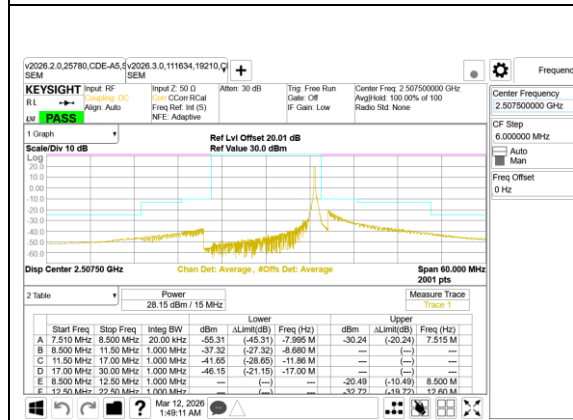
LTE B41 15MHz QPSK Low Channel RB1-74
