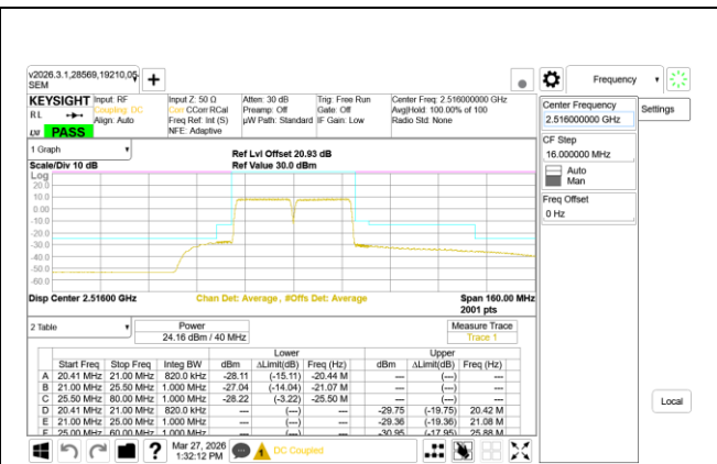
ULCA LTE B41 20MHz + 20MHz 16QAM Low Ch RB100-0 + RB100-0
