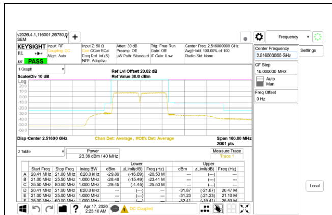
ULCA LTE B41 20MHz + 20MHz QPSK Low Ch RB100-0 + RB100-0
