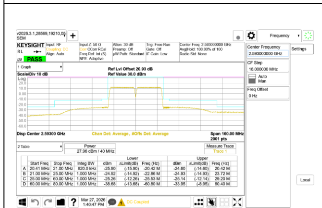
ULCA LTE B41 20MHz + 20MHz QPSK Mid Ch RB100-0 + RB100-0
