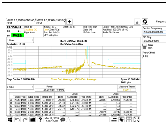
LTE B41 5MHz QPSK Low Channel RB1-24
