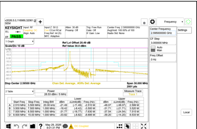
LTE B41 5MHz QPSK Middle Channel RB1-0
