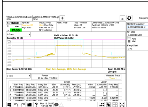
LTE B41 15MHz QPSK Low Channel RB75-0
