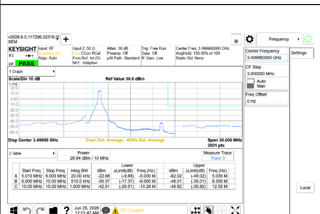
5G NR n77 10MHz BPSK Mid Channel RB1-0, Ant9+Ant8
