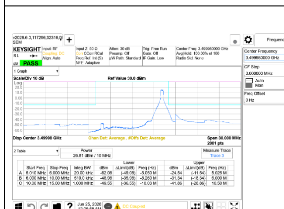
5G NR n77 10MHz BPSK Mid Channel RB1-23, Ant9+Ant8
