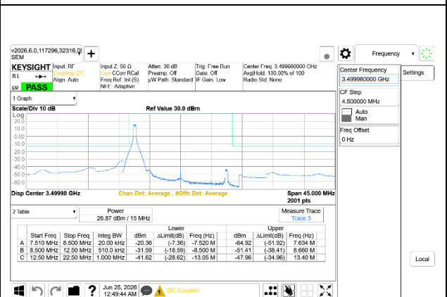
5G NR n77 15MHz BPSK Mid Channel RB1-0, Ant9+Ant8
