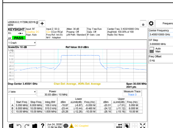
5G NR n77 10MHz BPSK Low Channel RB24-0, Ant9+Ant8
