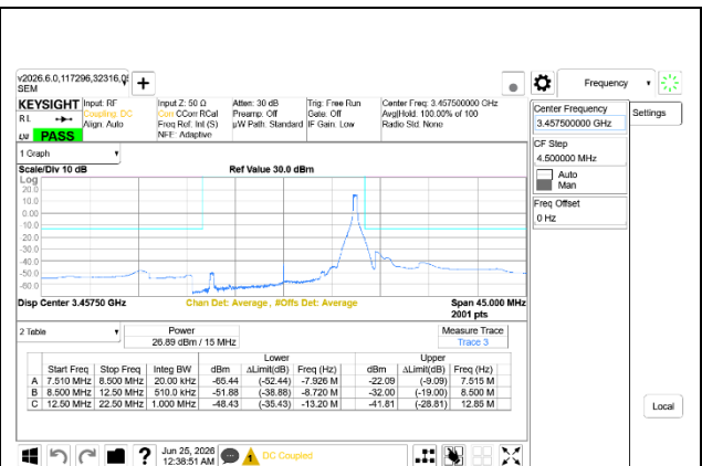
5G NR n77 15MHz BPSK Low Channel RB1-37, Ant9+Ant8
