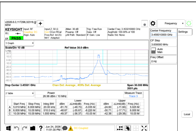
5G NR n77 10MHz BPSK Low Channel RB1-23, Ant9+Ant8
