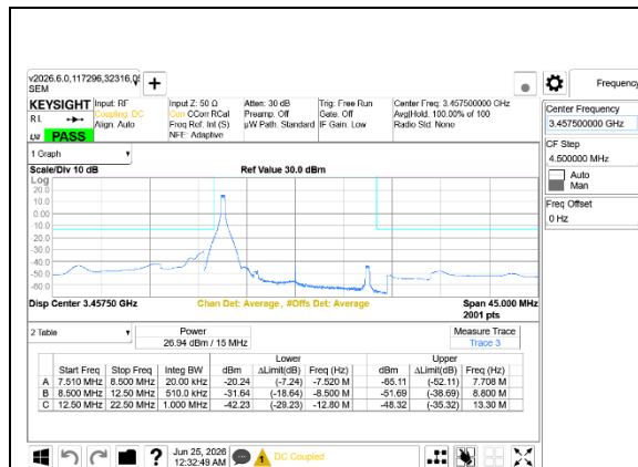
5G NR n77 15MHz BPSK Low Channel RB1-0, Ant9+Ant8
