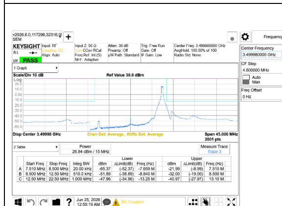
5G NR n77 15MHz BPSK Mid Channel RB1-37, Ant9+Ant8
