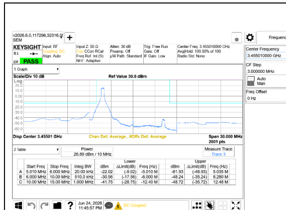
5G NR n77 10MHz BPSK Low Channel RB1-0, Ant9+Ant8
