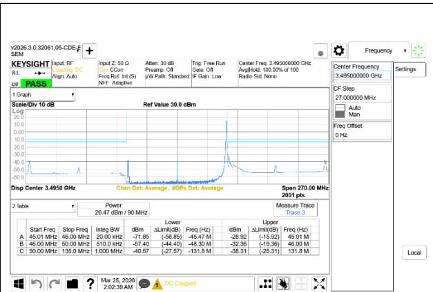
5G NR n77 90MHz BPSK Low Channel RB1-244, Ant9+Ant8
