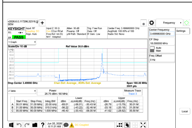
5G NR n77 60MHz BPSK Mid Channel RB1-161, Ant9+Ant8
