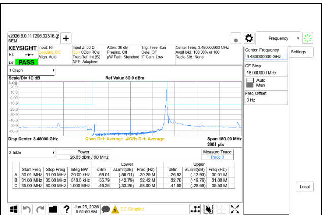
5G NR n77 60MHz BPSK Low Channel RB1-161, Ant9+Ant8
