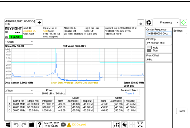
5G NR n77 90MHz BPSK Mid Channel RB1-0, Ant9+Ant8
