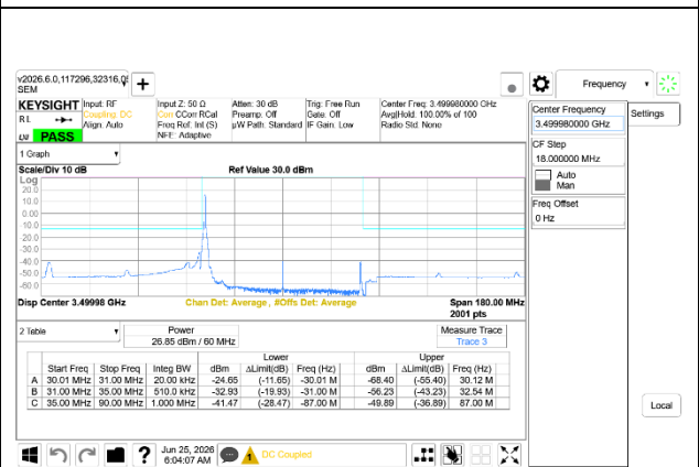
5G NR n77 60MHz BPSK Mid Channel RB1-0, Ant9+Ant8
