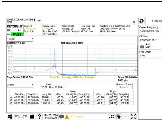
5G NR n77 90MHz BPSK Low Channel RB1-0, Ant9+Ant8
