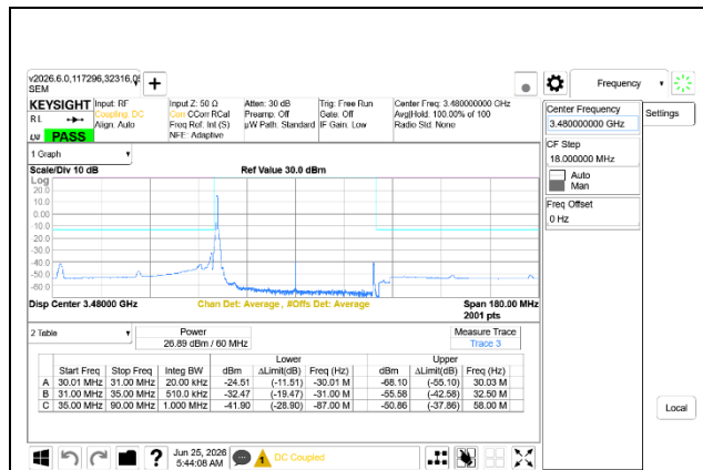
5G NR n77 60MHz BPSK Low Channel RB1-0, Ant9+Ant8
