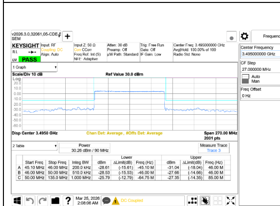
5G NR n77 90MHz BPSK Low Channel RB243-0, Ant9+Ant8
