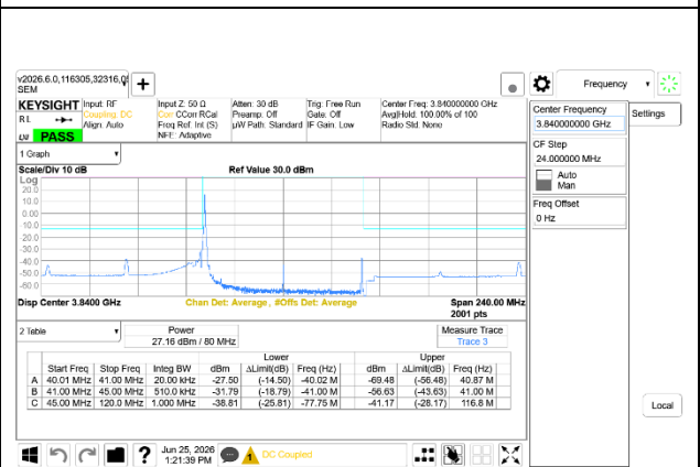
5G NR n77 80MHz BPSK Mid Channel RB1-0, Ant9+Ant8
