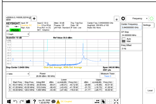
5G NR n77 80MHz BPSK Mid Channel RB1-216, Ant9+Ant8
