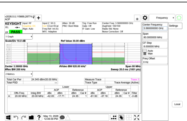
5G NR n48 20MHz QPSK Low Channel RB1-0, Ant9+Ant8
