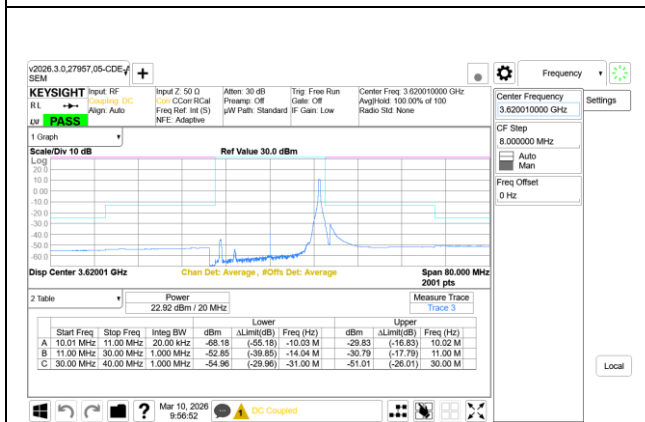
5G NR n48 20MHz QPSK Middle ChannelRB1-50, Ant9+Ant8
