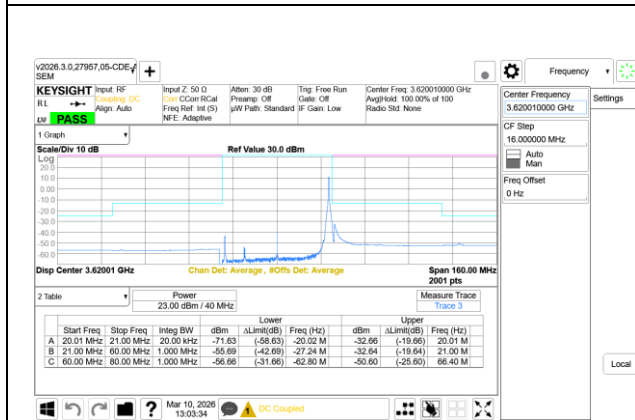
5G NR n48 40MHz QPSK Middle ChannelRB1-105, Ant9+Ant8
