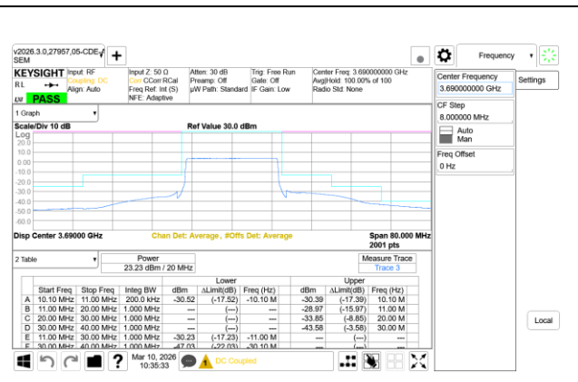
5G NR n48 20MHz QPSK High Channel RB51-0, Ant9+Ant8
