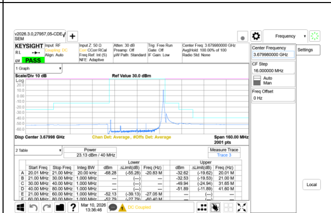
5G NR n48 40MHz QPSK High Channel RB1-105, Ant9+Ant8
