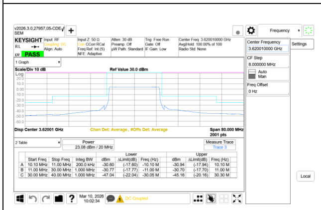
5G NR n48 20MHz QPSK Middle ChannelRB51-0, Ant9+Ant8
