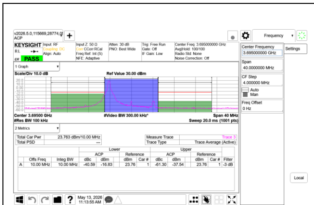
5G NR n48 10MHz QPSK High Channel RB1-0, Ant9+Ant8
