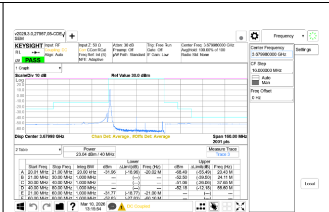
5G NR n48 40MHz QPSK High Channel RB1-0, Ant9+Ant8
