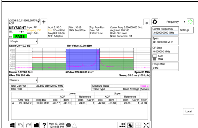
5G NR n48 20MHz QPSK Middle Channel RB1-50, Ant9+Ant8
