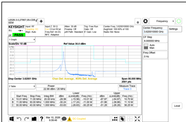
5G NR n48 20MHz QPSK Middle ChannelRB1-0, Ant9+Ant8
