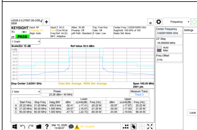
5G NR n48 40MHz QPSK Middle ChannelRB106-0, Ant9+Ant8
