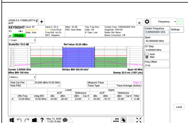
5G NR n48 10MHz QPSK High Channel RB24-0, Ant9+Ant8
