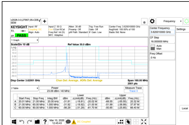
5G NR n48 40MHz QPSK Middle ChannelRB1-0, Ant9+Ant8
