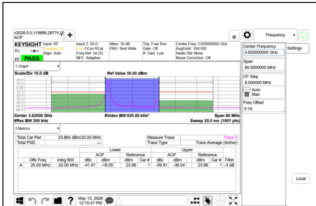
5G NR n48 20MHz QPSK Middle Channel RB1-0, Ant9+Ant8
