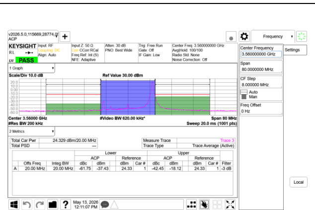
5G NR n48 20MHz QPSK Low Channel RB1-50, Ant9+Ant8
