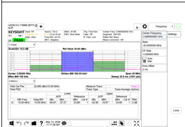
5G NR n48 10MHz QPSK High Channel RB1-23, Ant9+Ant8
