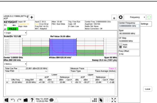
5G NR n48 20MHz QPSK High Channel RB1-0, Ant9+Ant8
