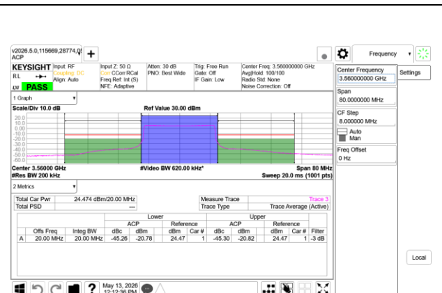
5G NR n48 20MHz QPSK Low Channel RB51-0, Ant9+Ant8
