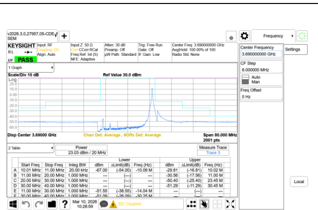
5G NR n48 20MHz QPSK High Channel RB1-50, Ant9+Ant8
