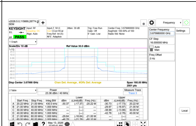
5G NR n48 40MHz QPSK High Channel RB106-0, Ant9+Ant8
