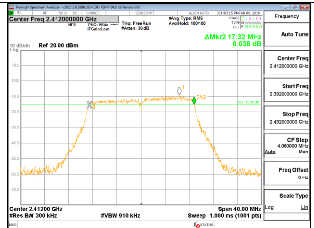
HT20-mode – 2412 Channel – ANT 4 SISO
