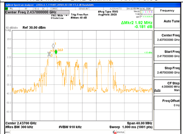
EHT20-mode – 2437 Channel – Partial RU0 – ANT 4 MIMO
