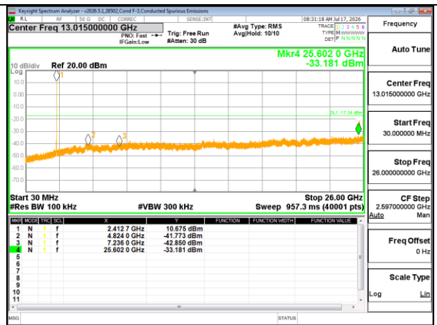
LOW CHANNEL 1, OUT-OF-BAND
