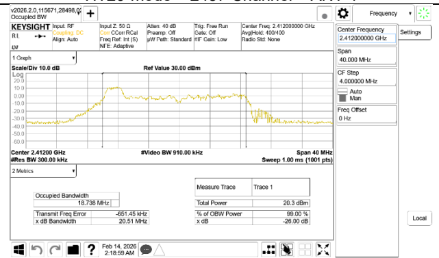
EHT20-mode - 2412 Channel - Partial RU0 - ANT 4
