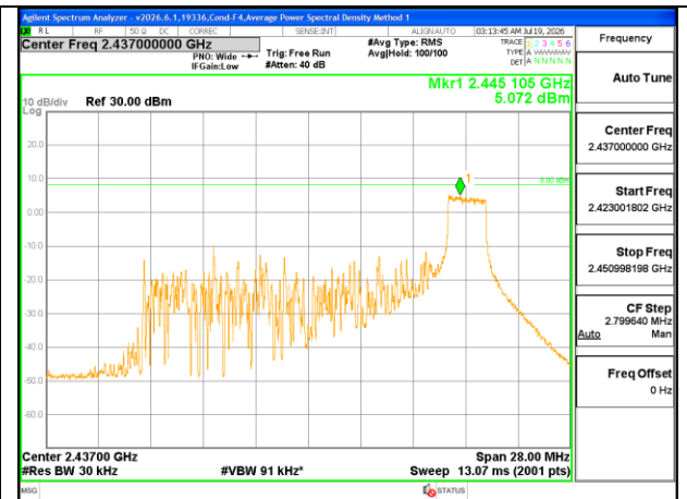
Worst Case Plot Channel 6 26-Tone Index 8 [ANT 3]
