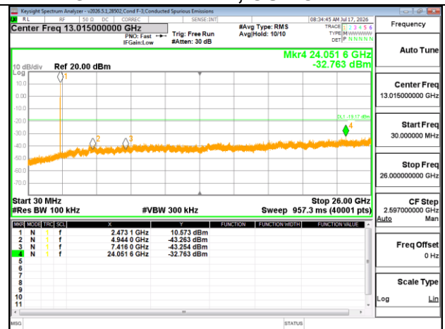
HIGH CHANNEL 13, OUT-OF-BAND
