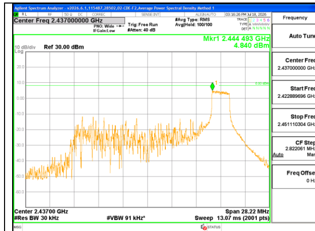
Worst Case Plot Channel 6 26-Tone Index 8 [ANT 4]
