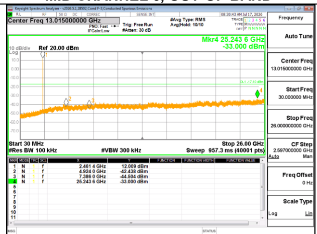
HIGH CHANNEL 11, OUT-OF-BAND
