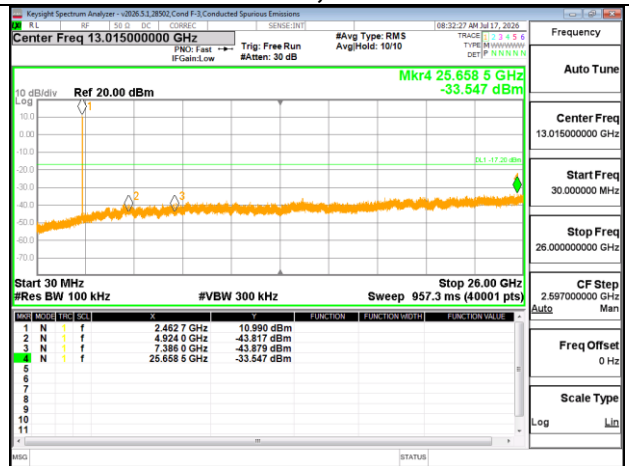
HIGH CHANNEL 11, OUT-OF-BAND
