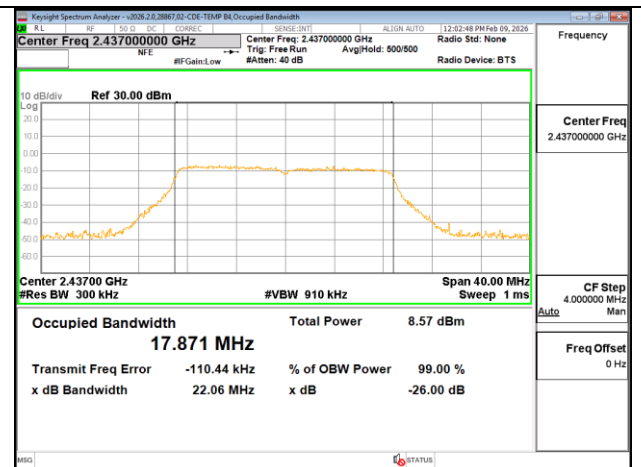
HT20-mode - 2437 Channel - ANT 4
