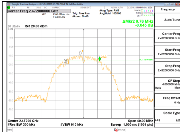
b-mode – 2472 Channel – ANT 4 SISO
