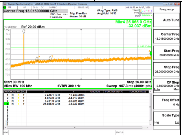
MID CHANNEL 6, OUT-OF-BAND
