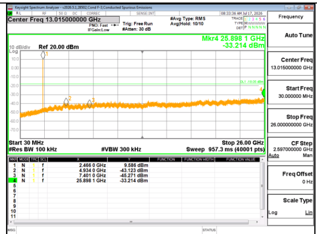
HIGH CHANNEL 12, OUT-OF-BAND
