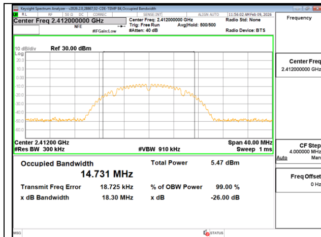
b-mode - 2412 Channel - ANT 3
