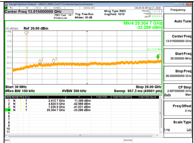
LOW CHANNEL 1, OUT-OF-BAND
