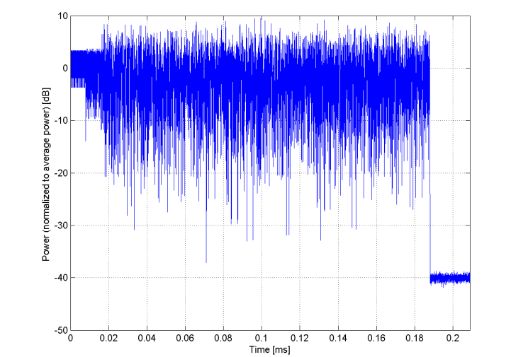
Time Domain
