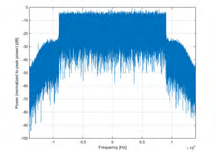
Frequency Domain
