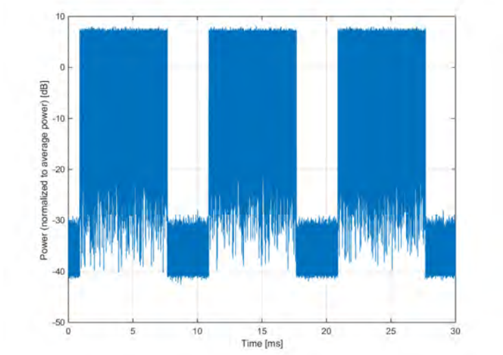
Time Domain
