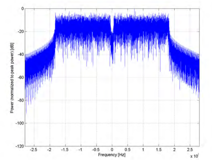
Frequency Domain
