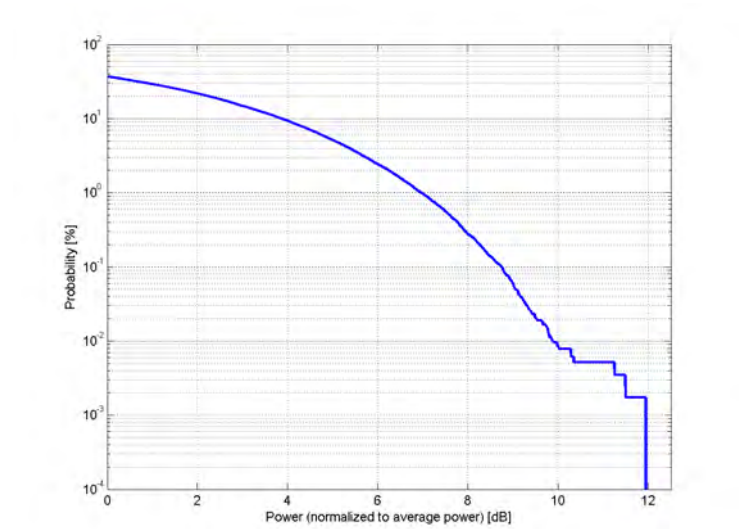
Complementary Cumulative Distribution Function (CCDF)
