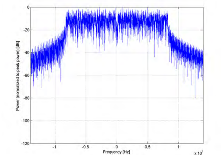
Frequency Domain
