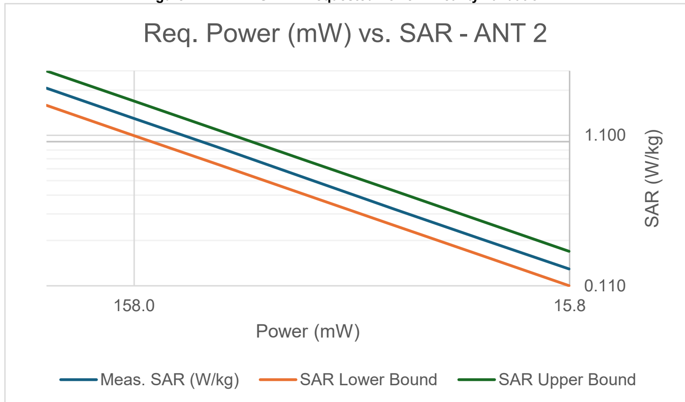
Figure 4-2: ANT 2 SAR v. Requested Power Linearity Validation
