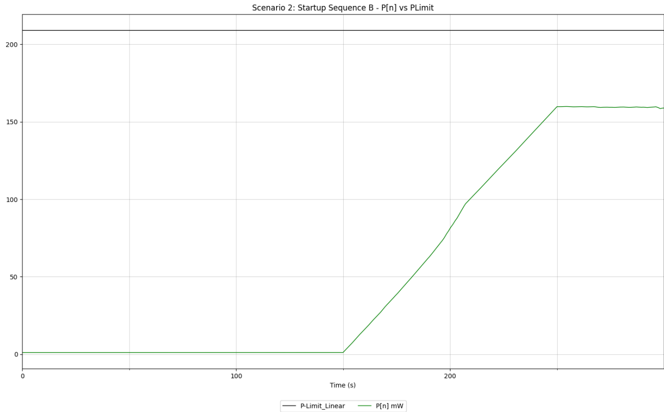
Figure 6-6: W-CDMA P[n] vs. P Limit Sequence B Validation (Conducted)
