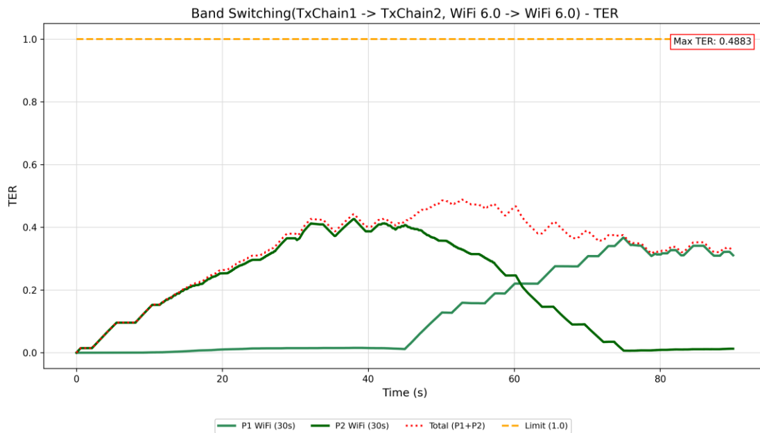
Figure 6-23: Change in Operating State and Antenna Switching (Conducted)
