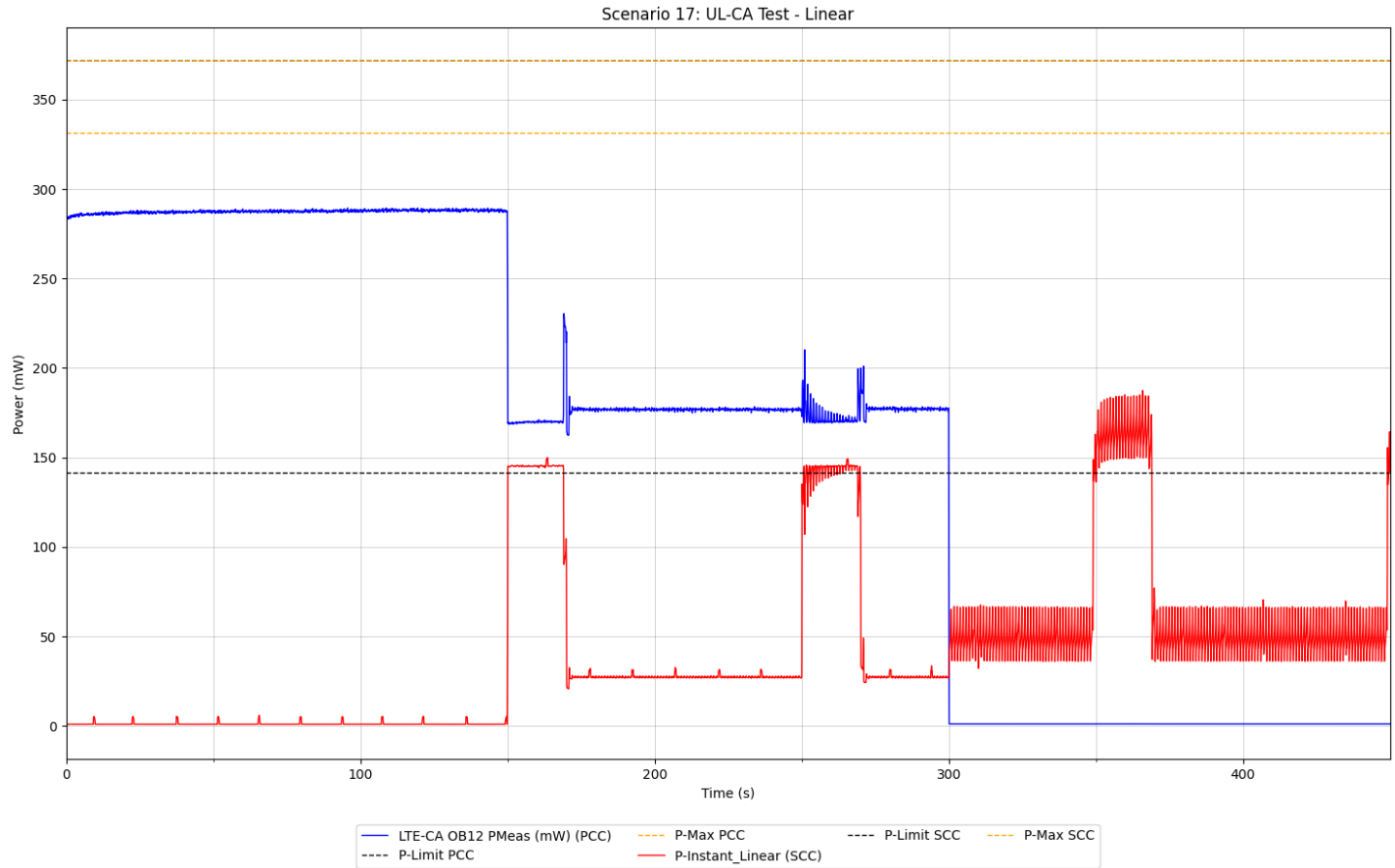
Figure 6-24: Technology Hand-off ULCA Test Case (Conducted)
