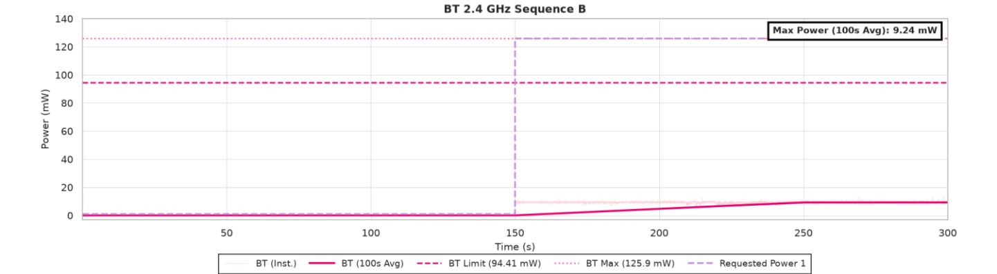
Figure 6-17: Bluetooth 2.4 GHz Start-up Sequence B and P[n] vs. P Limit (Conducted)
