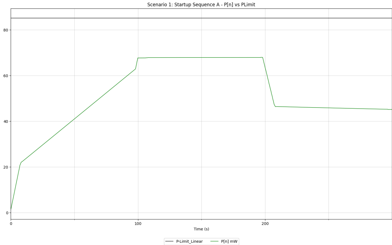
Figure 6-2: FR-1 TDD P[n] vs. P_{Limit} Sequence A Validation (Conducted)
