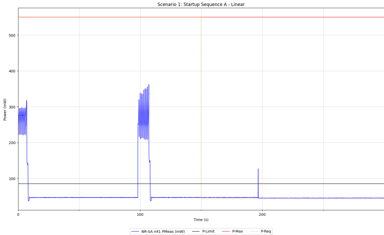
Figure 6-1: FR-1 TDD Start-up Sequence A (Conducted)
