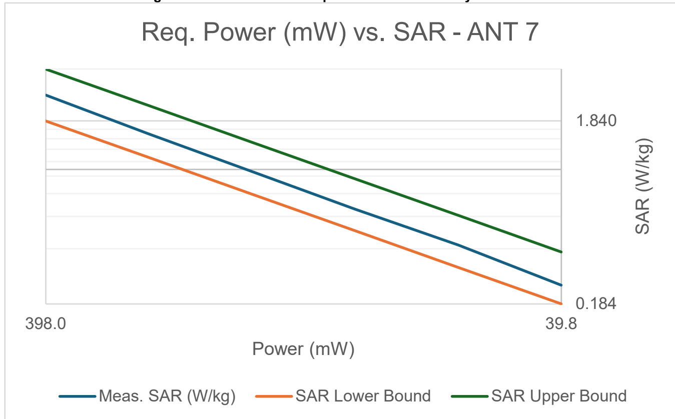
Figure 4-5: ANT 7 SAR v. Requested Power Linearity Validation
