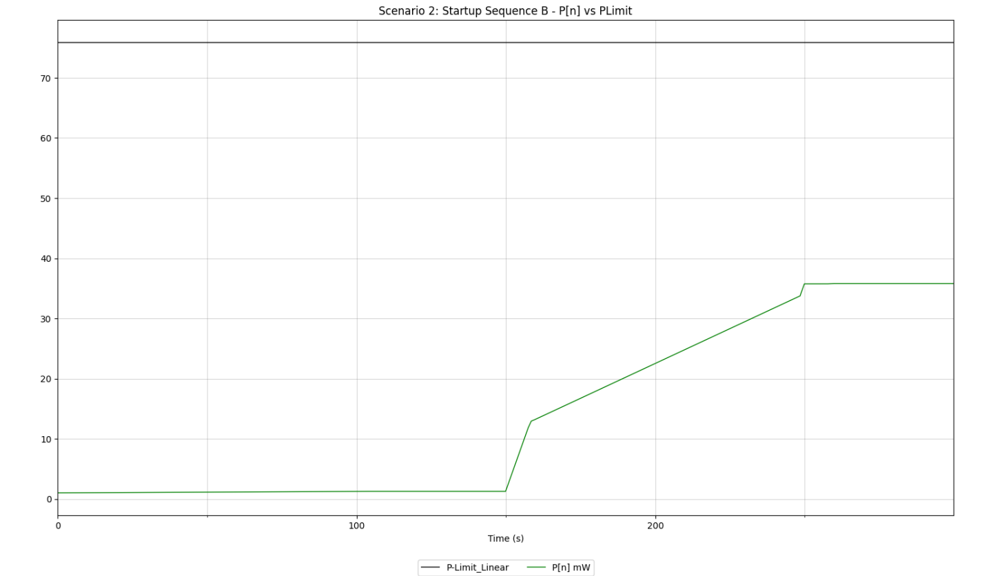
Figure 6-12: FR-1 FDD P[n] vs. P Limit Sequence B Validation (Conducted)
