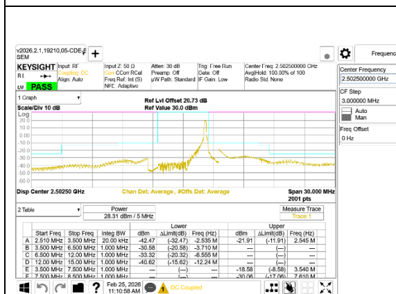
LTE B41 5MHz QPSK Low Channel RB1-24
