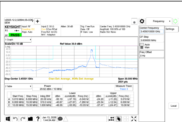
5G NR n77 10MHz BPSK Low Channel RB1-23 Ant7+Ant8
