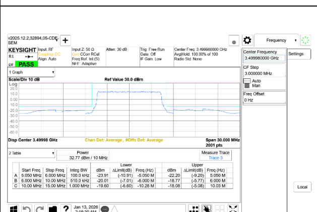
5G NR n77 10MHz BPSK Mid Channel RB24-0 Ant7+Ant8
