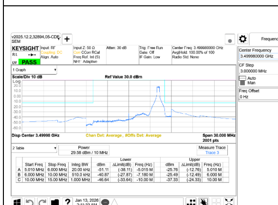
5G NR n77 10MHz BPSK Mid Channel RB1-23 Ant7+Ant8
