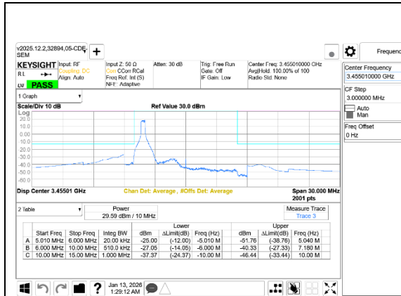
5G NR n77 10MHz BPSK Low Channel RB1-0 Ant7+Ant8
