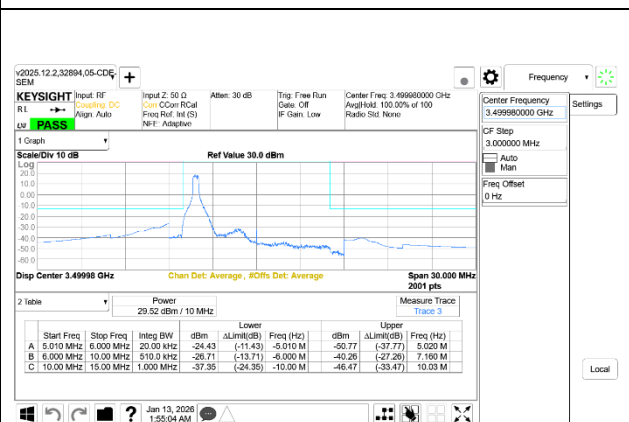
5G NR n77 10MHz BPSK Mid Channel RB1-0 Ant7+Ant8
