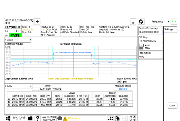
5G NR n77 40MHz BPSK Mid Channel RB100-0 Ant7+Ant8
