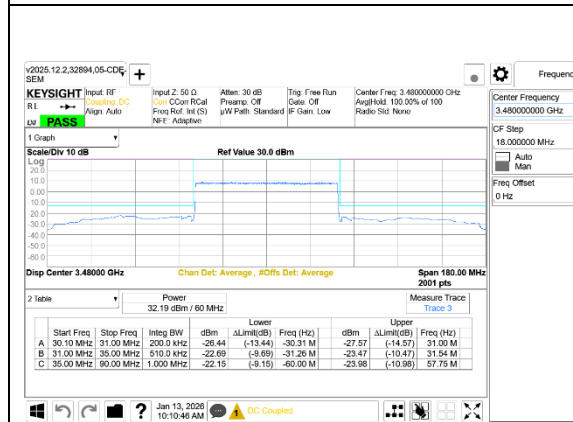
5G NR n77 60MHz BPSK Low Channel RB162-0 Ant7+Ant8
