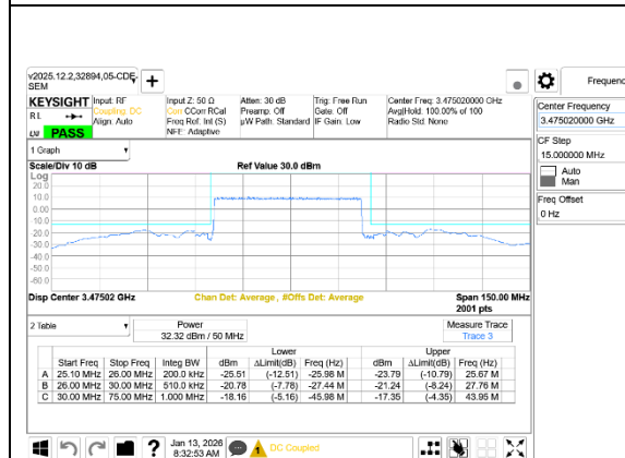
5G NR n77 50MHz BPSK Low Channel RB128-0 Ant7+Ant8
