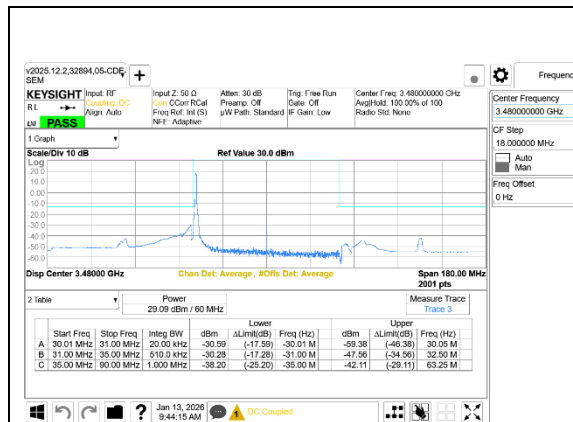
5G NR n77 60MHz BPSK Low Channel RB1-0 Ant7+Ant8
