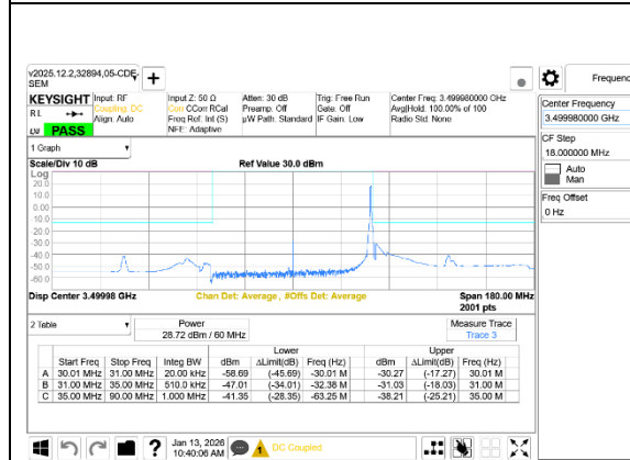
5G NR n77 60MHz BPSK Mid Channel RB1-161 Ant7+Ant8
