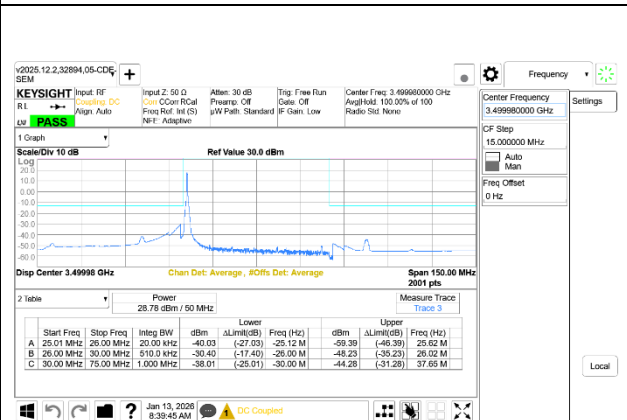
5G NR n77 50MHz BPSK Mid Channel RB1-0 Ant7+Ant8
