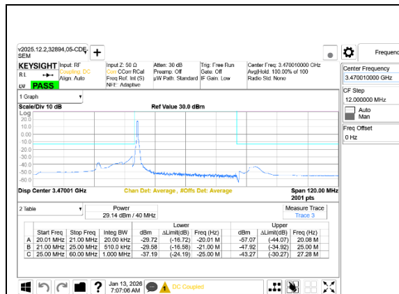
5G NR n77 40MHz BPSK Low Channel RB1-0 Ant7+Ant8
