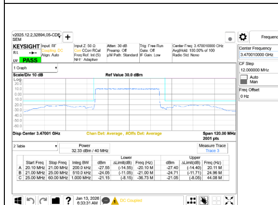
5G NR n77 40MHz BPSK Low Channel RB100-0 Ant7+Ant8
