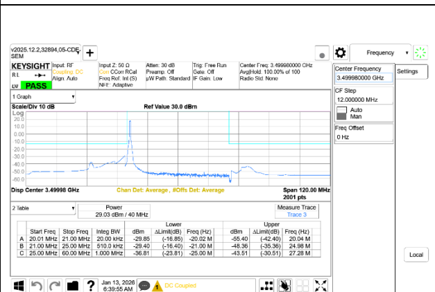
5G NR n77 40MHz BPSK Mid Channel RB1-0 Ant7+Ant8
