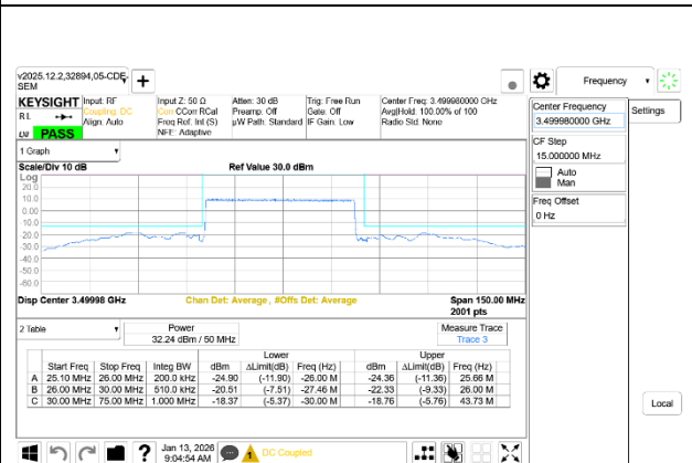
5G NR n77 50MHz BPSK Mid Channel RB128-0 Ant7+Ant8
