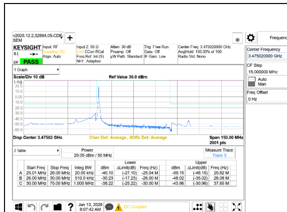
5G NR n77 50MHz BPSK Low Channel RB1-0 Ant7+Ant8
