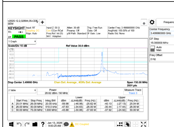
5G NR n77 50MHz BPSK Mid Channel RB1-132 Ant7+Ant8
