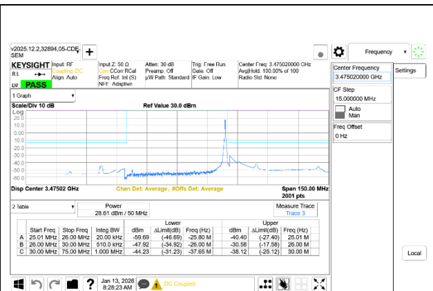
5G NR n77 50MHz BPSK Low Channel RB1-132 Ant7+Ant8
