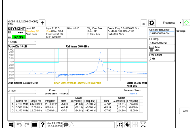
5G NR n77 15MHz BPSK Mid Channel RB1-37 Ant7+Ant8
