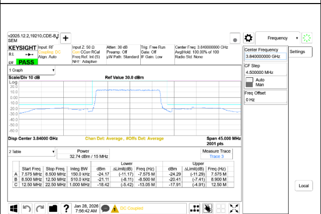
5G NR n77 15MHz BPSK Mid Channel RB36-0 Ant7+Ant8
