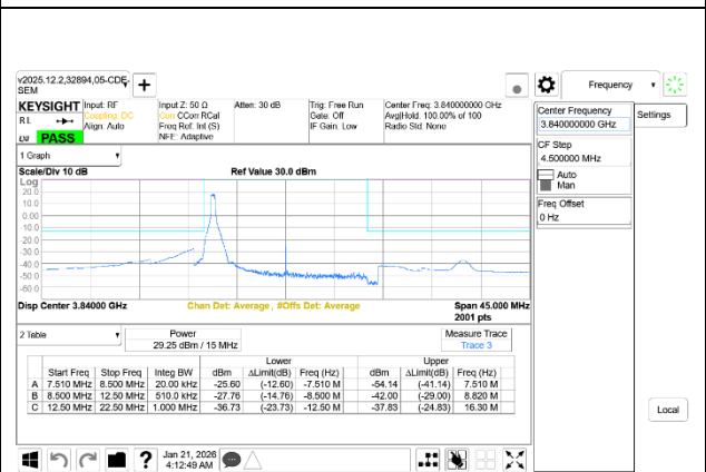
5G NR n77 15MHz BPSK Mid Channel RB1-0 Ant7+Ant8
