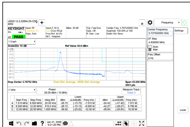
5G NR n77 15MHz BPSK Low Channel RB1-0 Ant7+Ant8
