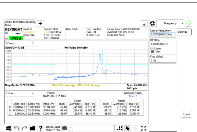
5G NR n77 15MHz BPSK Low Channel RB1-37 Ant7+Ant8
