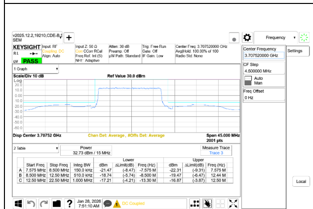
5G NR n77 15MHz BPSK Low Channel RB36-0 Ant7+Ant8
