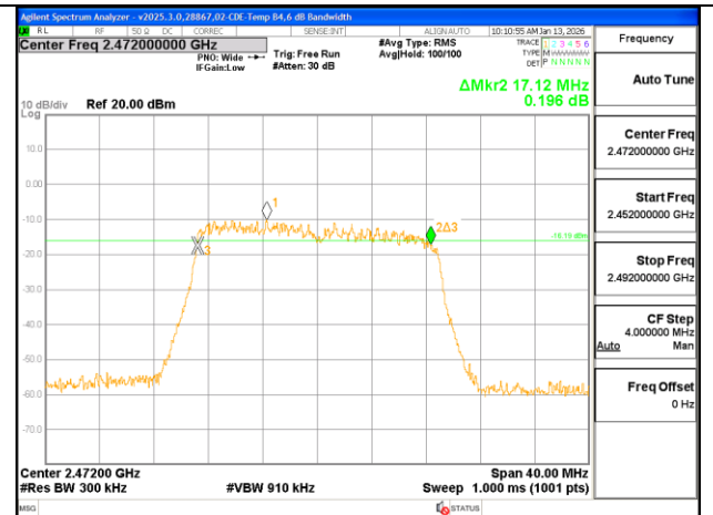
HT20-mode - 2472 Channel - ANT 3 SISO
