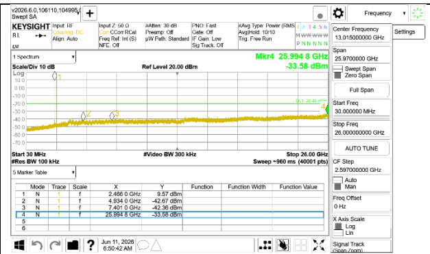
OUT-OF-BAND HIGH CHANNEL 12 ANT 4
