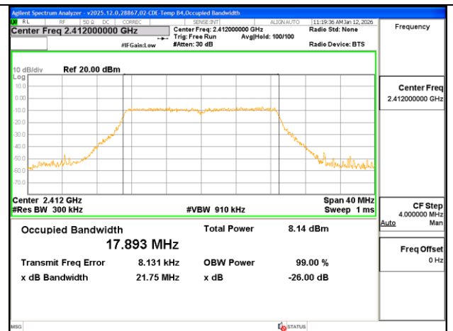
HT20-mode – 2412 Channel – ANT 3
