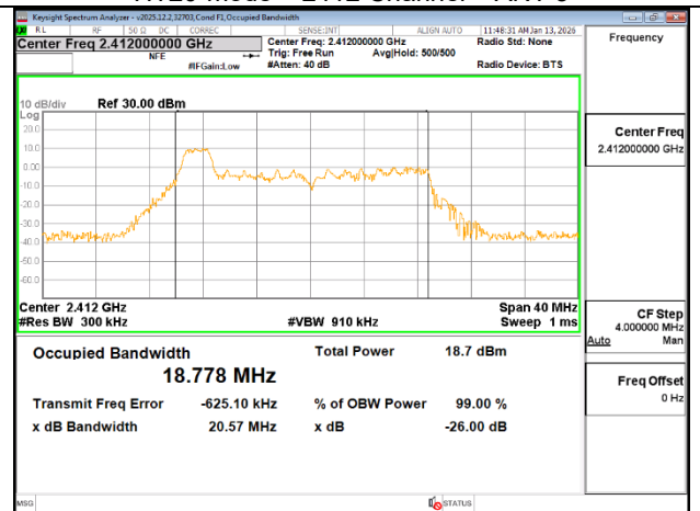
EHT20-mode – 2412 Channel – Partial RU0 – ANT 3
