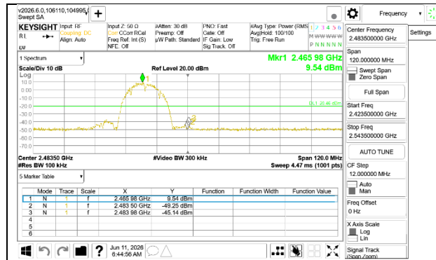
HIGH CHANNEL 12 BANDEGE ANT 4
