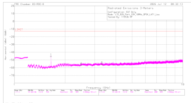
A3713 LTE B26 QPSK Low Channel Horizontal
