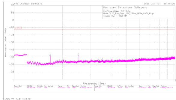
A3713 LTE B26 QPSK High Channel Horizontal
