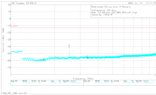
A3472 LTE B26 QPSK High Channel Vertical
