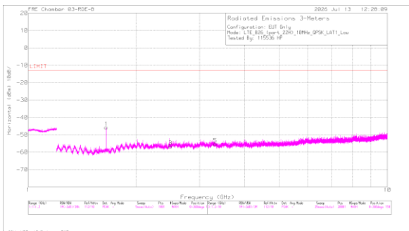
A3472 LTE B26 QPSK Low Channel Horizontal
