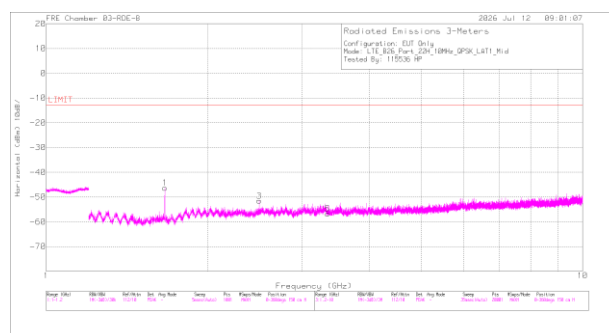
A3713 LTE B26 QPSK Middle Channel Horizontal
