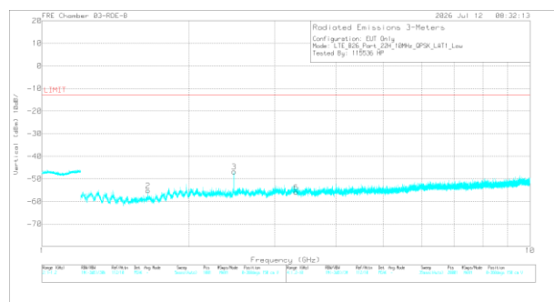
A3713 LTE B26 QPSK Low Channel Vertical
