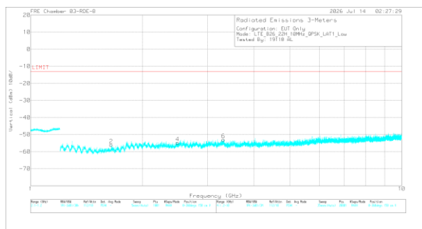
A3715 LTE B26 QPSK Low Channel Vertical
