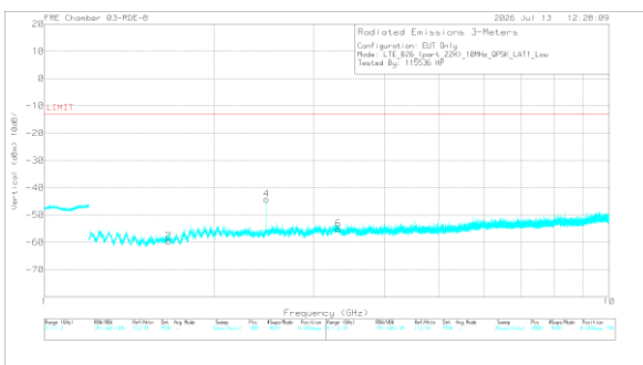
A3472 LTE B26 QPSK Low Channel Vertical
