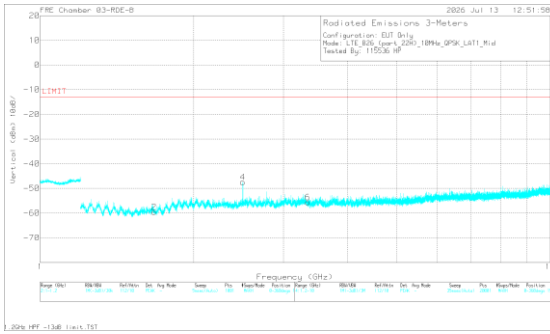
A3472 LTE B26 QPSK Mid Channel Vertical
