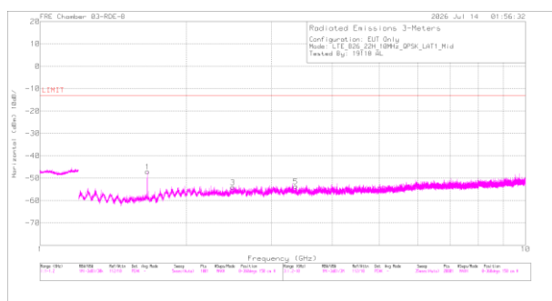
A3715 LTE B26 QPSK Middle Channel Horizontal
