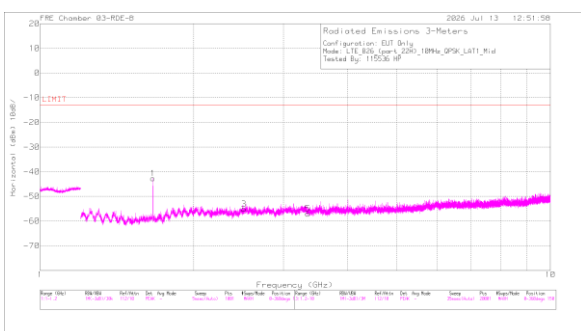
A3472 LTE B26 QPSK Mid Channel Horizontal
