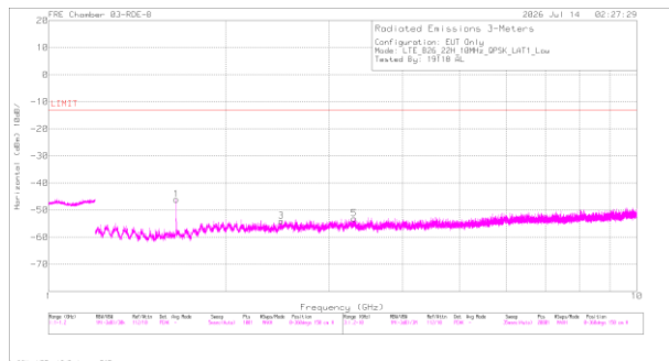
A3715 LTE B26 QPSK Low Channel Horizontal
