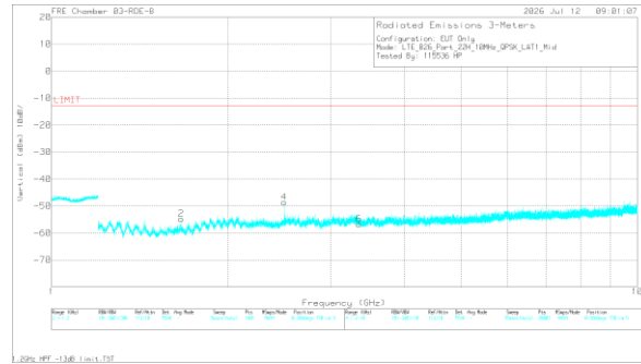
A3713 LTE B26 QPSK Middle Channel Vertical
