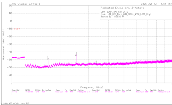
A3472 LTE B26 QPSK High Channel Horizontal
