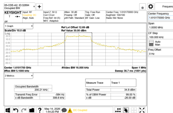
Occupied Bandwidth Low Channel Ant 4
