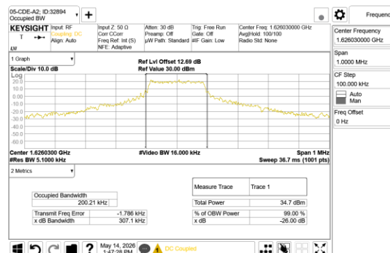
Occupied Bandwidth High Channel Ant 4
