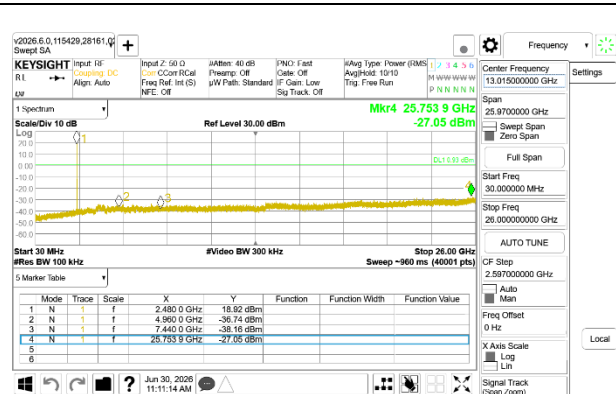
HIGH CHANNEL OUT-OF-BAND
