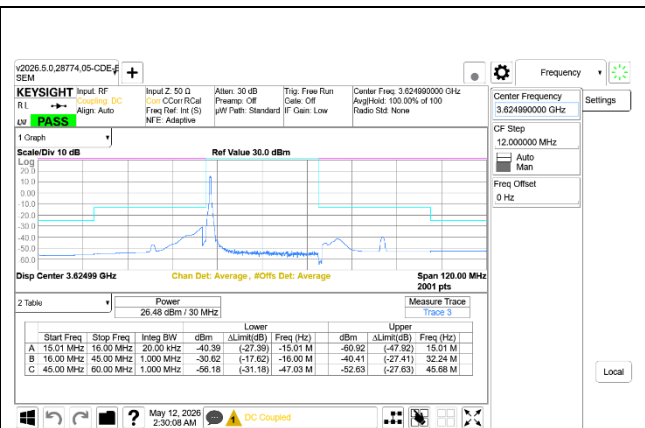
5G NR n48 30MHz BPSK Middle Channel RB1-0 Ant7 + Ant8
