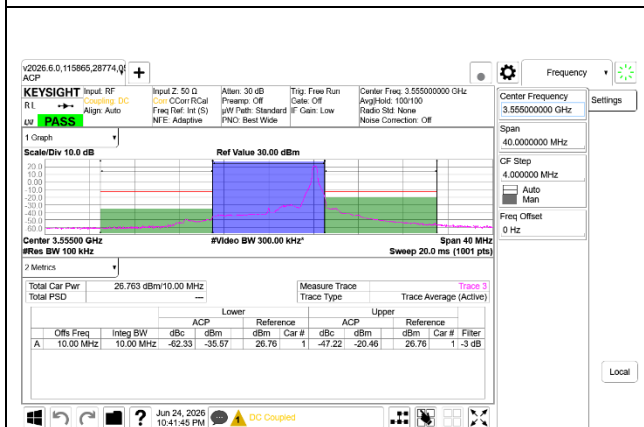
5G NR n48 10MHz BPSK Low Channel RB1-23 Ant7 + Ant8
