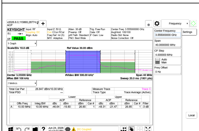
5G NR n48 10MHz BPSK Low Channel RB24-0 Ant7 + Ant8
