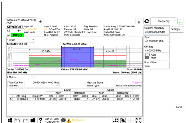
5G NR n48 10MHz BPSK Low Channel RB1-0 Ant7 + Ant8
