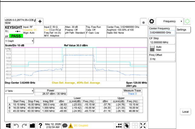
5G NR n48 30MHz BPSK Middle Channel RB75-0 Ant7 + Ant8
