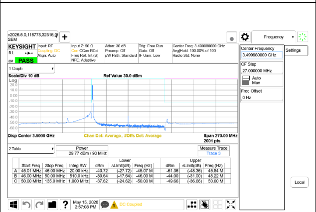
5G NR n77 90MHz BPSK Mid Channel RB1-0 Ant7+Ant8
