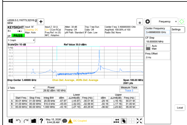
5G NR n77 60MHz BPSK Mid Channel RB1-161 Ant7+Ant8
