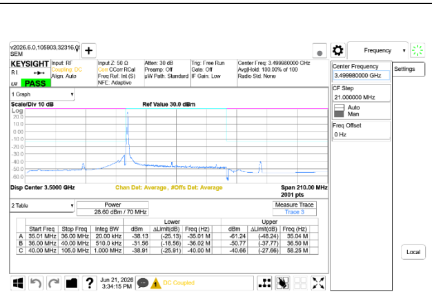
5G NR n77 70MHz BPSK Mid Channel RB1-0 Ant7+Ant8
