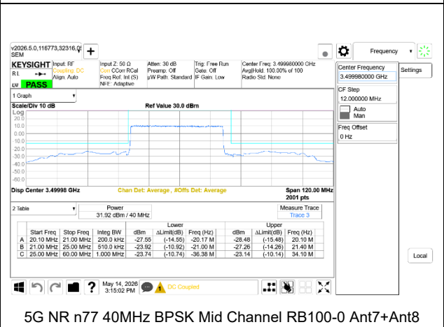
5G NR n77 40MHz BPSK Mid Channel RB100-0 Ant7+Ant8
