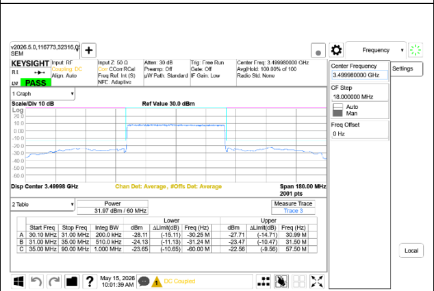
5G NR n77 60MHz BPSK Mid Channel RB162-0 Ant7+Ant8
