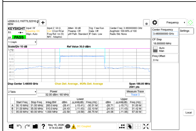
5G NR n77 60MHz BPSK Low Channel RB162-0 Ant7+Ant8
