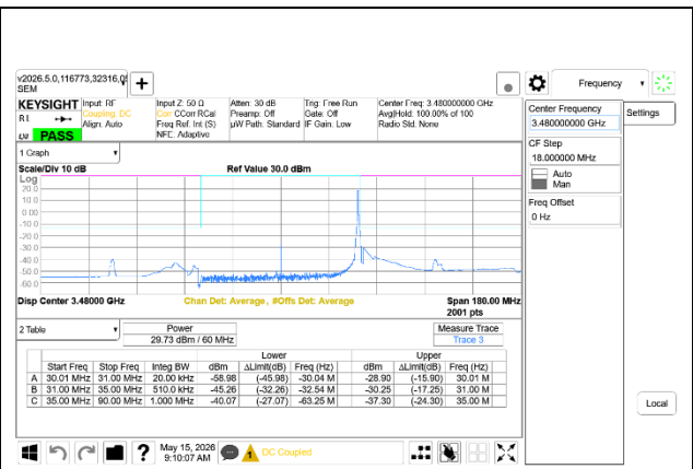
5G NR n77 60MHz BPSK Low Channel RB1-161 Ant7+Ant8
