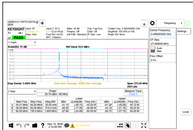
5G NR n77 90MHz BPSK Low Channel RB1-0 Ant7+Ant8
