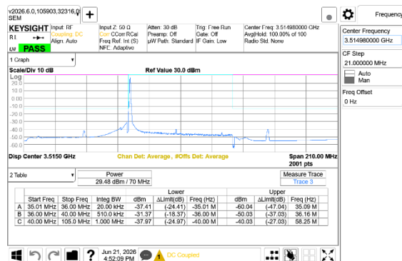
5G NR n77 70MHz BPSK High Channel RB1-0 Ant7+Ant8
