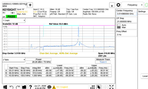
5G NR n77 70MHz BPSK High Channel RB1-188 Ant7+Ant8
