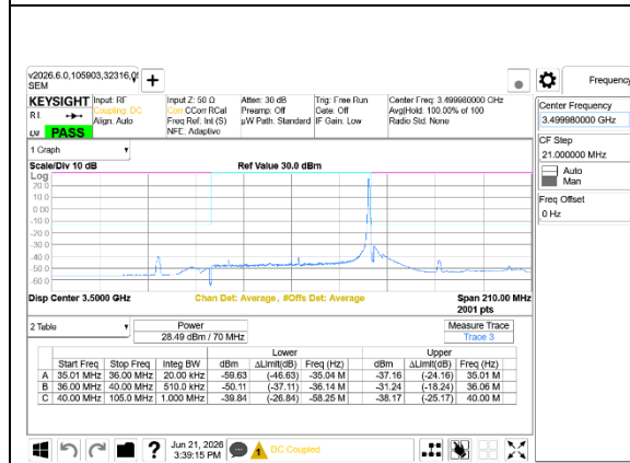
5G NR n77 70MHz BPSK Mid Channel RB1-188 Ant7+Ant8
