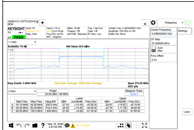
5G NR n77 90MHz BPSK Low Channel RB243-0 Ant7+Ant8
