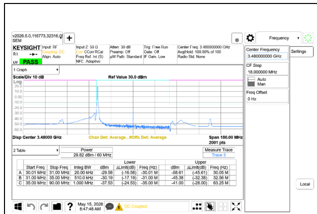
5G NR n77 60MHz BPSK Low Channel RB1-0 Ant7+Ant8
