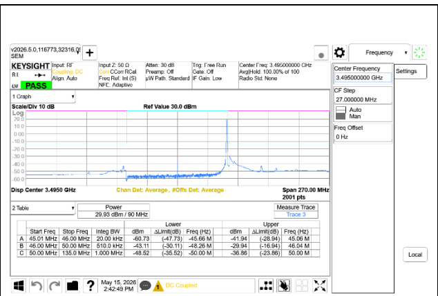
5G NR n77 90MHz BPSK Low Channel RB1-244 Ant7+Ant8
