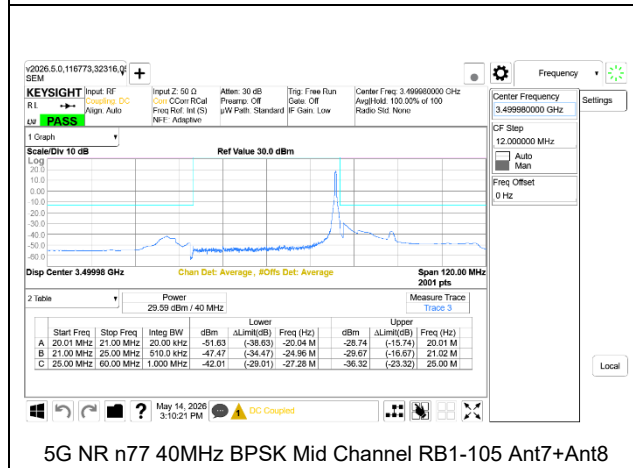
5G NR n77 40MHz BPSK Mid Channel RB1-105 Ant7+Ant8
