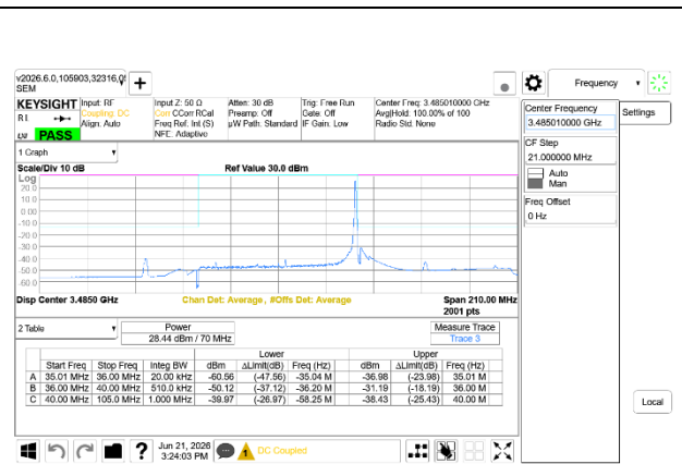
5G NR n77 70MHz BPSK Low Channel RB1-188 Ant7+Ant8
