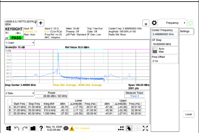
5G NR n77 60MHz BPSK Mid Channel RB1-0 Ant7+Ant8
