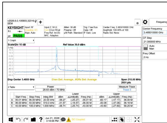
5G NR n77 70MHz BPSK Low Channel RB1-0 Ant7+Ant8
