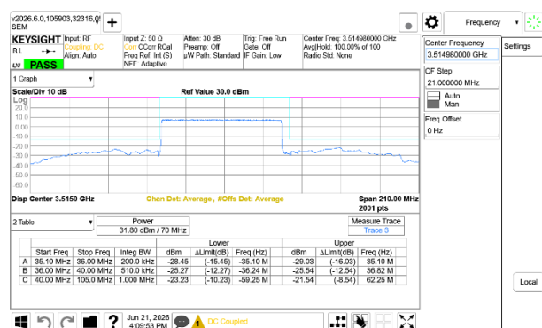
5G NR n77 70MHz BPSK High Channel RB180-0 Ant7+Ant8
