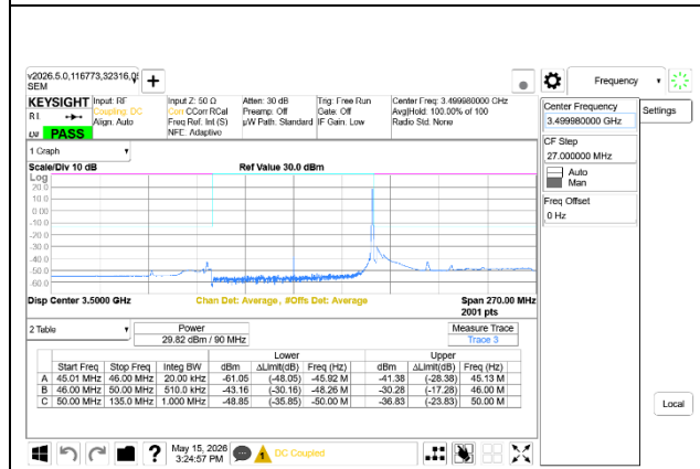
5G NR n77 90MHz BPSK Mid Channel RB1-244 Ant7+Ant8
