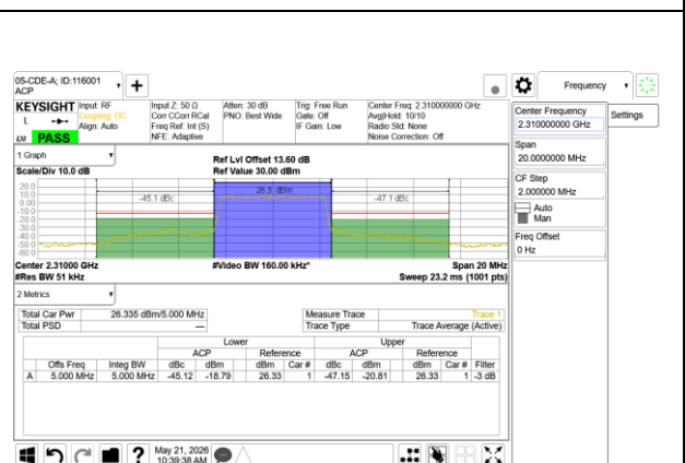
5G NR n30 5MHz BPSK Middle Channel RB25-0
