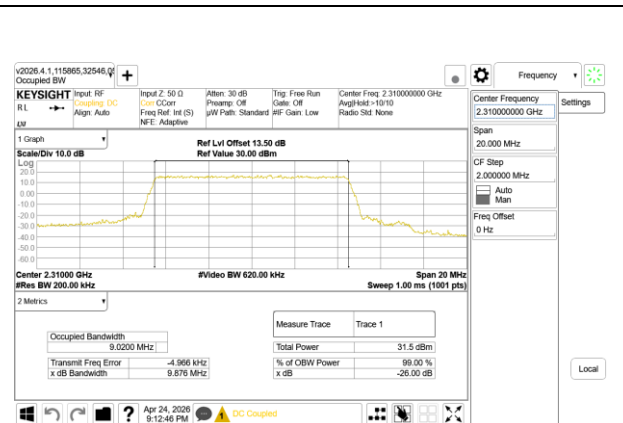
LTE B30 10MHz QPSK Middle Channel RB50-0
