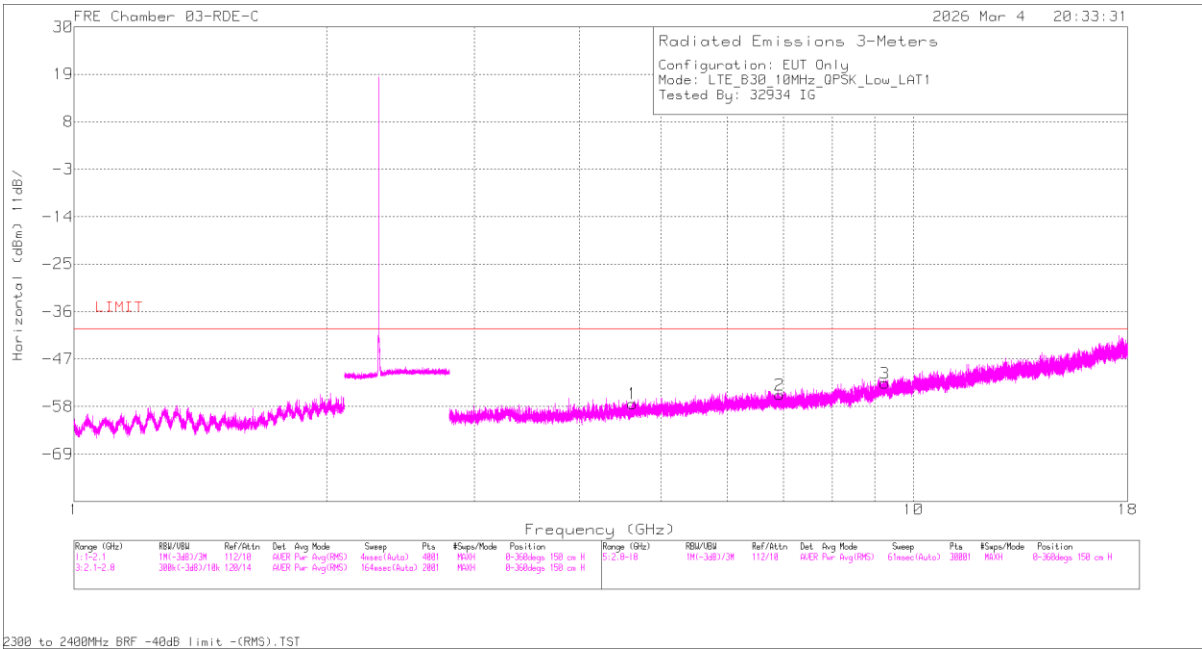
Horizontal Polarity
