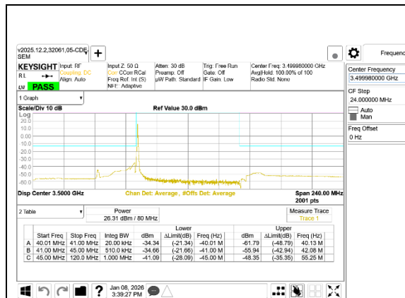
5G NR n77 80MHz BPSK Middle Channel RB1-0
