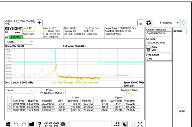
5G NR n77 100MHz BPSK Mid Channel RB1-0
