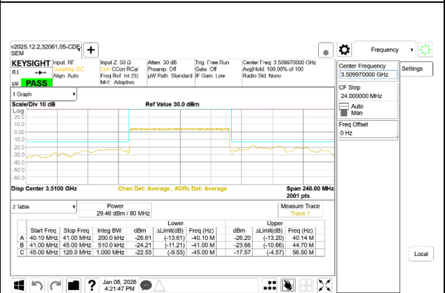
5G NR n77 80MHz BPSK High Channel RB216-0
