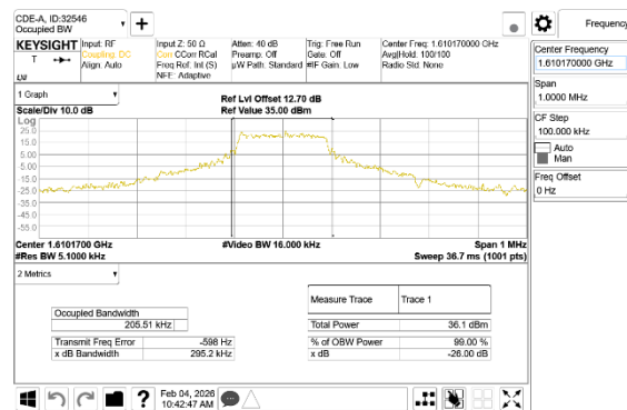
Occupied Bandwidth Low Channel
