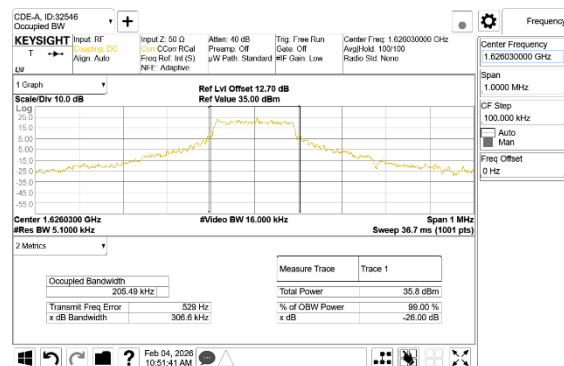
Occupied Bandwidth High Channel
