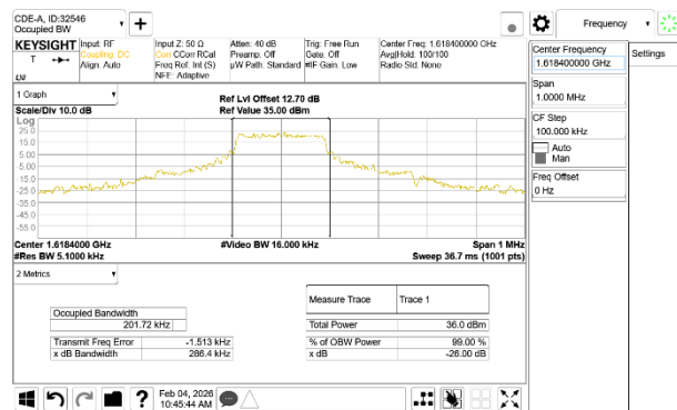
Occupied Bandwidth Mid Channel
