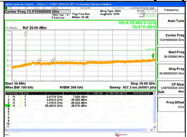
HIGH CHANNEL 13, OUT-OF-BAND [ANT 4]
