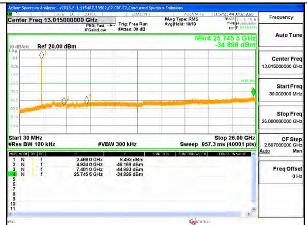
HIGH CHANNEL 12, OUT-OF-BAND [ANT 4]
