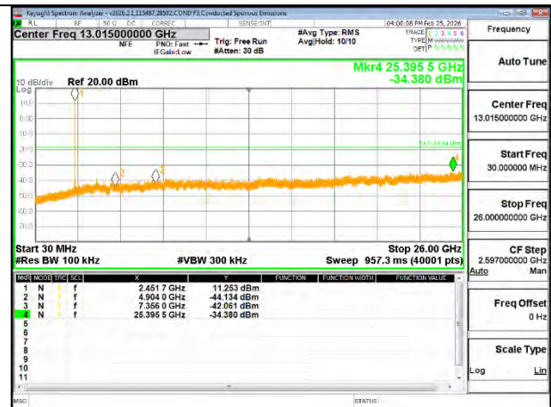
HIGH CHANNEL 9, OUT-OF-BAND [ANT 4]
