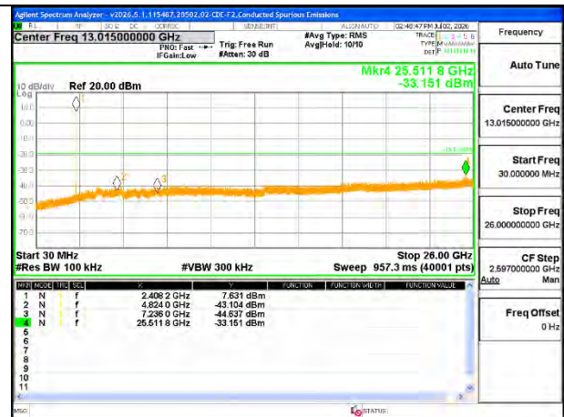
LOW CHANNEL 1, OUT-OF-BAND [ANT 3]
