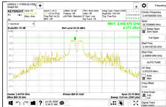
Channel 8 – 26 Tone Index 4 [ANT 4]
