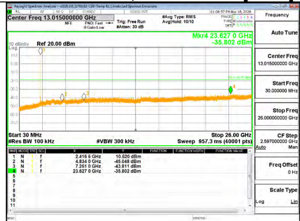
LOW CHANNEL 2, OUT-OF-BAND [ANT 3]
