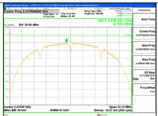
Worst Case Plot Channel 6 [ANT 3]
