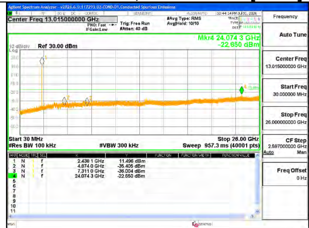
MID CHANNEL 6, OUT-OF-BAND [ANT 3]
