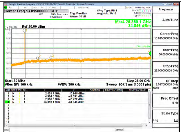
HIGH CHANNEL 9, OUT-OF-BAND [ANT 3]
