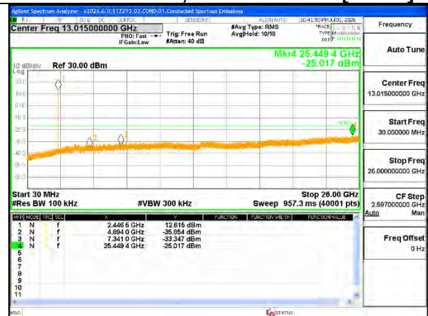
HIGH CHANNEL 8, OUT-OF-BAND [ANT 4]
