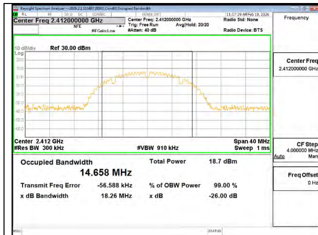
b-mode – Channel 1 – ANT 4
