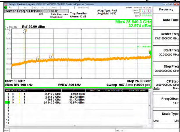
LOW CHANNEL 3, OUT-OF-BAND [ANT 3]
