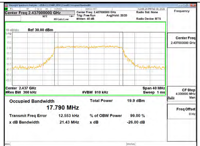
HT20-mode – Channel 6 – ANT 3
