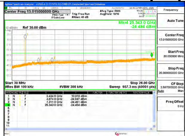
MID CHANNEL 6, OUT-OF-BAND [ANT 4]
