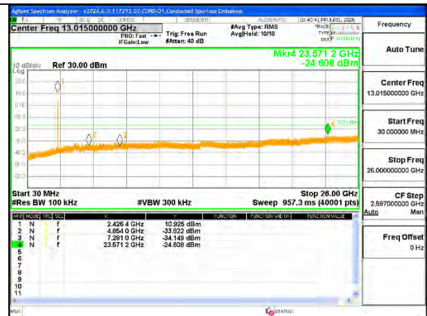
LOW CHANNEL 4, OUT-OF-BAND [ANT 4]
