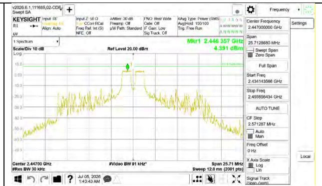
Channel 8 – 26 Tone Index 4 [ANT 3]
