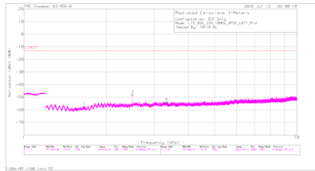
A3721 LTE B26 QPSK Middle Channel Horizontal
