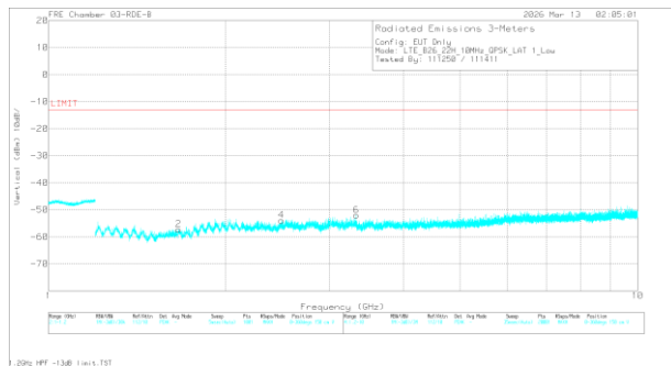
A3447 LTE B26 QPSK Low Channel Vertical
