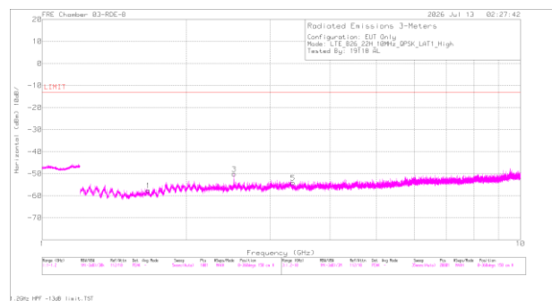
A3721 LTE B26 QPSK High Channel Horizontal
