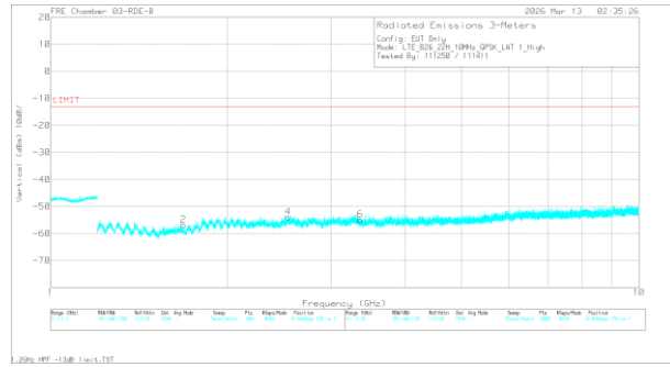
A3447 LTE B26 QPSK High Channel Vertical
