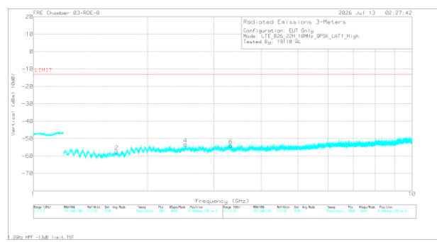
A3721 LTE B26 QPSK High Channel Vertical
