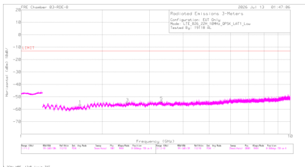
A3721 LTE B26 QPSK Low Channel Horizontal
