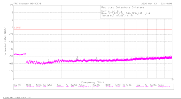
A3447 LTE B26 QPSK Mid Channel Horizontal
