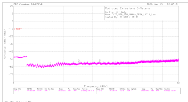
A3447 LTE B26 QPSK Low Channel Horizontal
