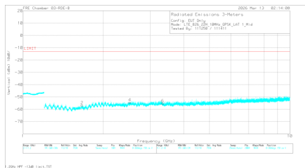
A3447 LTE B26 QPSK Mid Channel Vertical
