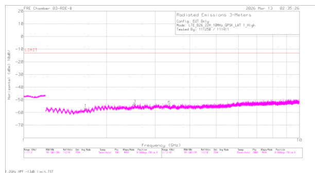
A3447 LTE B26 QPSK High Channel Horizontal
