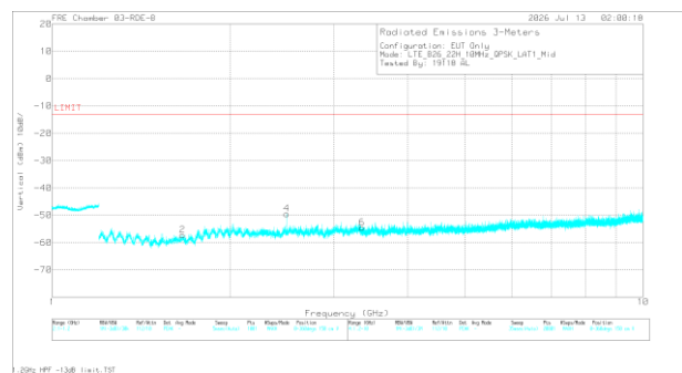
A3721 LTE B26 QPSK Middle Channel Vertical
