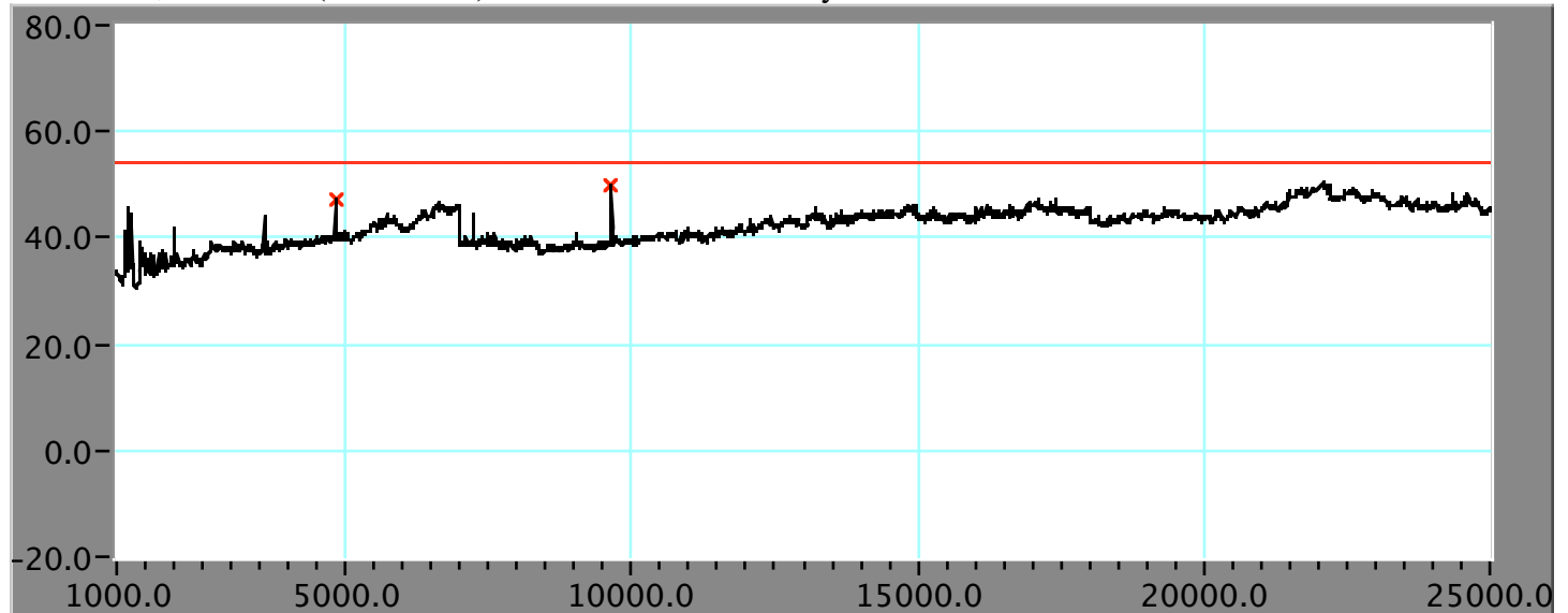
Horizontal, channel 1 (2.412 GHz) - 802.11b mode Host System #2
