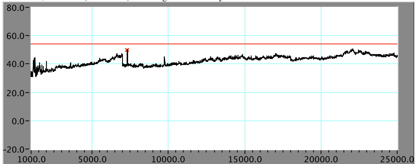
Horizontal, channel 6 (2.437 GHz) - 802.11g mode Host System #2
