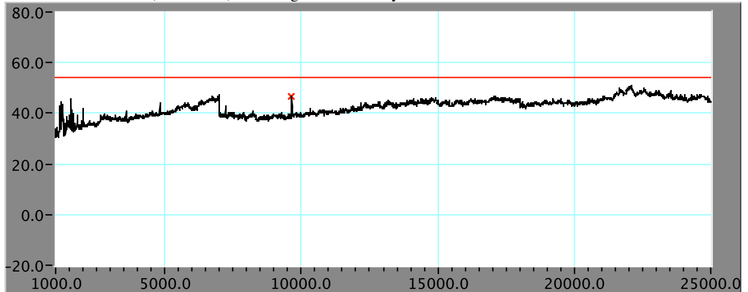
Horizontal, channel 1 (2.412 GHz) - 802.11g mode Host System #2
