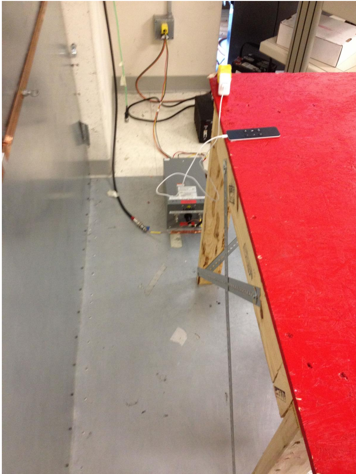
AC Line Conducted Emissions Setup Side:
