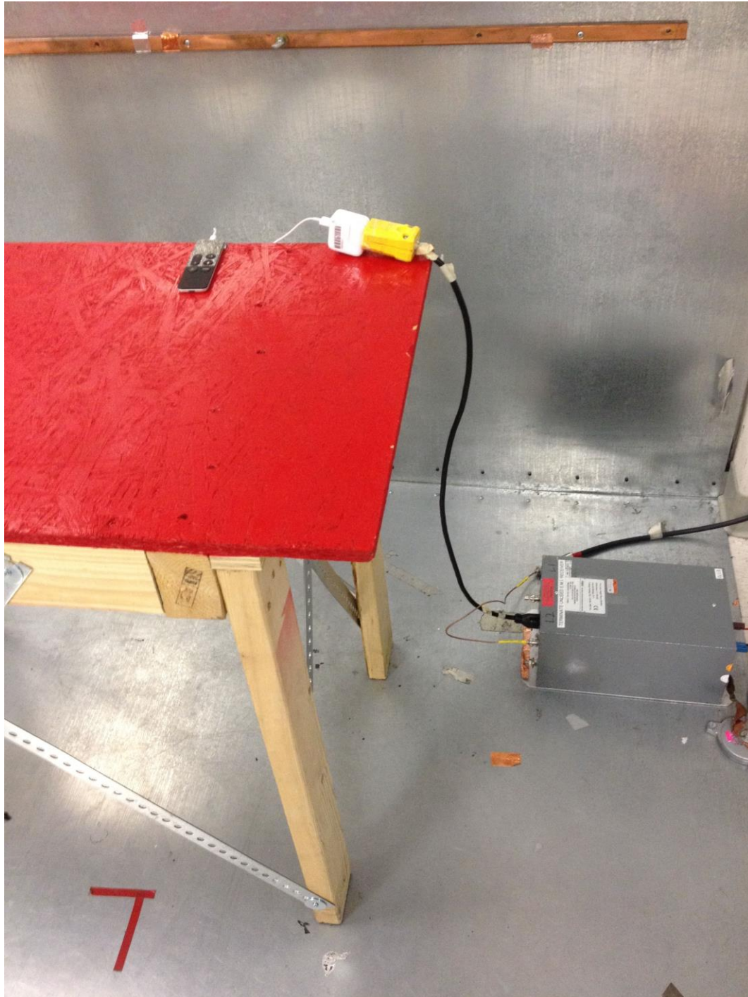
AC Line Conducted Emissions Setup Front:
