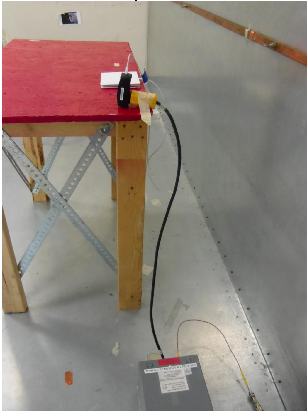
AC Line Conducted Emissions Setup 2
