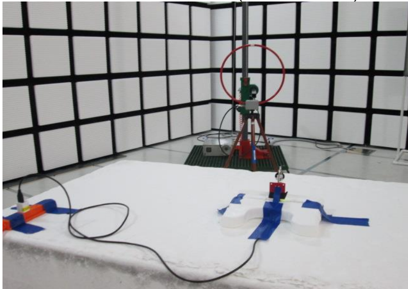
RADIATED EMISSIONS BELOW 30MHz (BACK - STANDBY)
