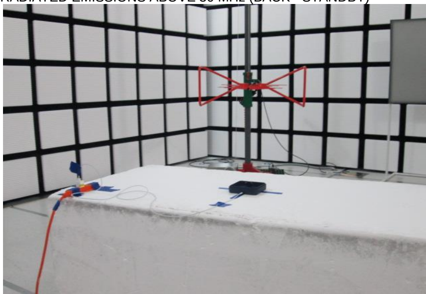
RADIATED EMISSIONS ABOVE 30 MHz (BACK - STANDBY)
