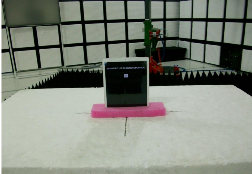
Z-AXIS PHOTO
