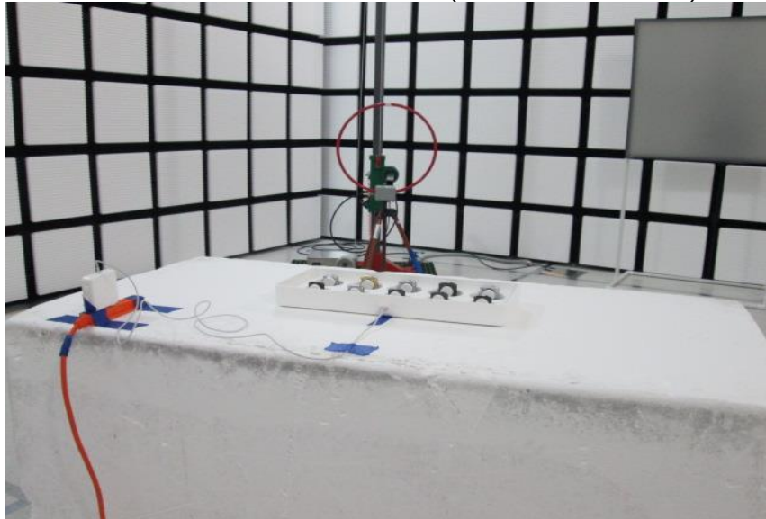
RADIATED EMISSIONS BELOW 30MHz (BACK – OPERATING)
