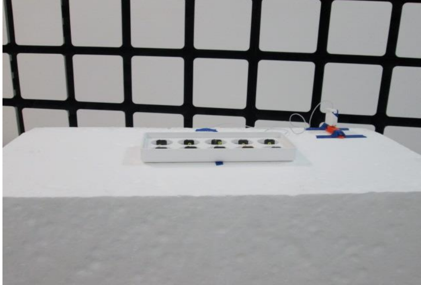
RADIATED EMISSIONS ABOVE 30 MHz (FRONT – OPERATING)
