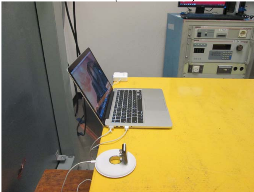
LINE CONDUCTED EMISSION (BACK - OPERATING)
