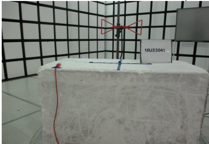
RADIATED EMISSIONS ABOVE 30 MHz (FRONT - STANDBY)
