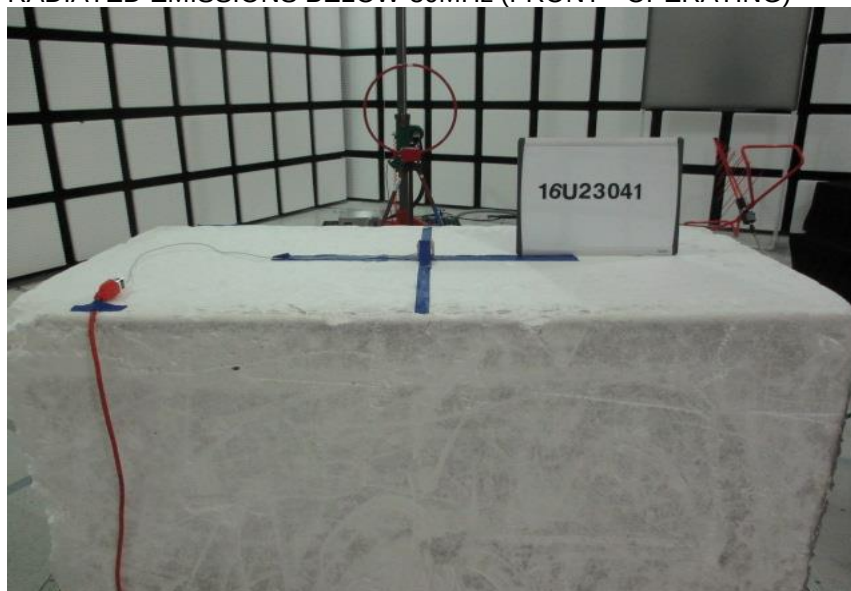
RADIATED EMISSIONS BELOW 30MHz (FRONT - OPERATING)
