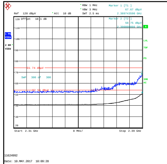
2310 MHz to 2390 MHz Restricted Band
