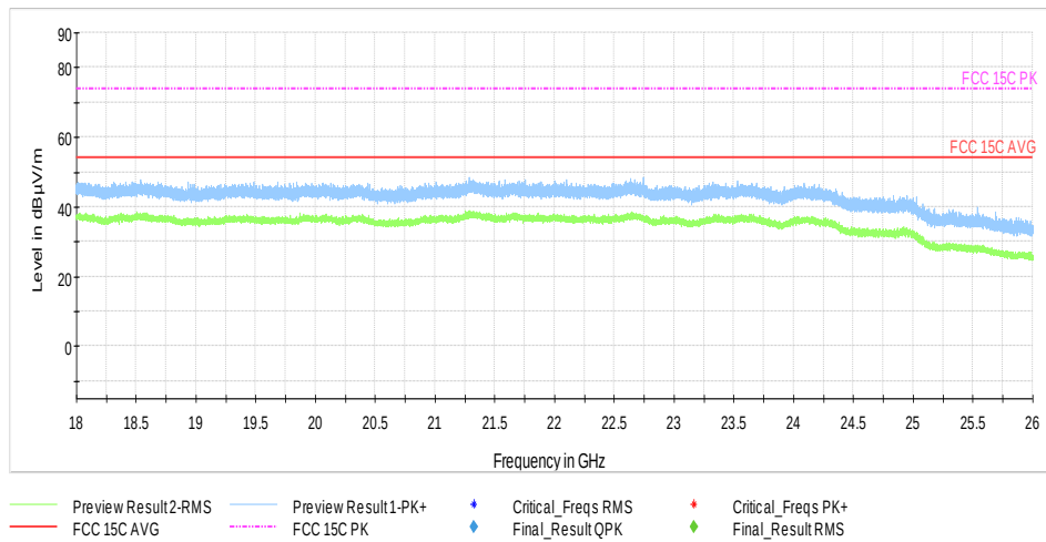
Plot #8 Radiated Emissions: 18-26 GHz
