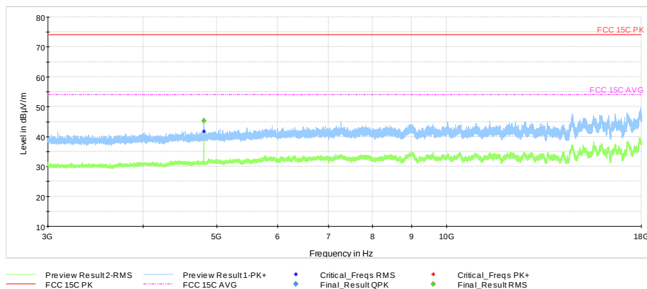
Plot # 3 Radiated Emissions: 3-18 GHz
