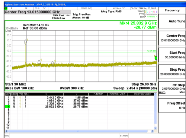
OUT-OF-BAND HIGH CHANNEL 7 WF4
