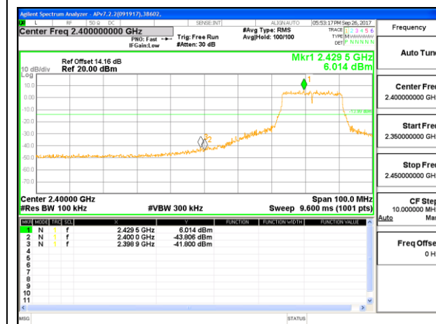
LOW CHANNEL 5 BANDEDGE WF4
