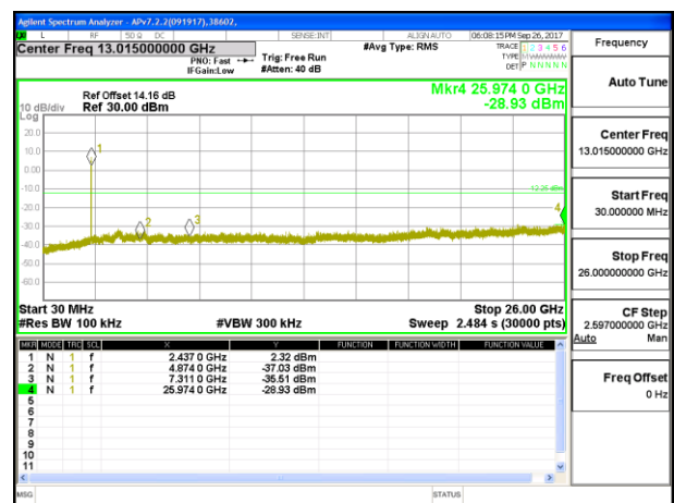
OUT-OF-BAND MID CHANNEL WF4
