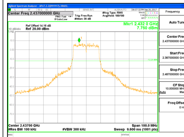
IN-BAND REFERENCE LEVEL WF4
