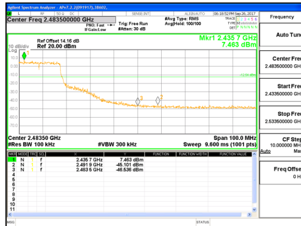
HIGH CHANNEL 7 BANDEDGE WF4
