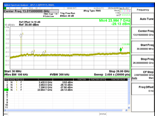
OUT-OF-BAND LOW CHANNEL 5 WF4
