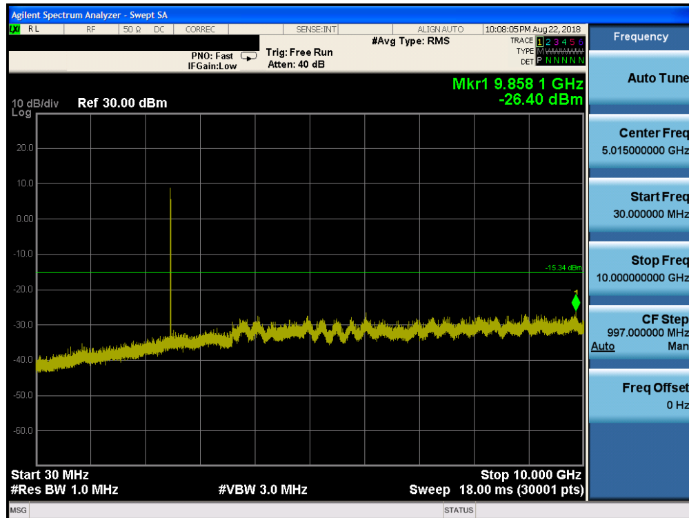
Plot 7-77. Conducted Spurious Plot ANT1 (Bluetooth (HDR4), 4Mbps, ePA – Ch. 75)
