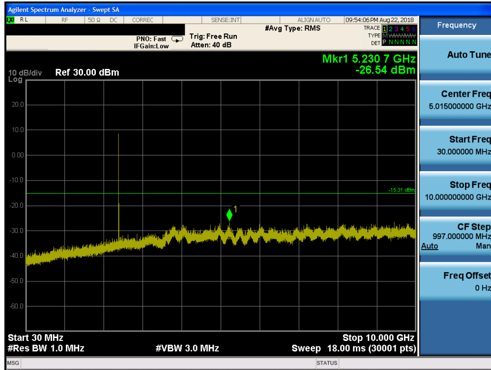
Plot 7-73. Conducted Spurious Plot ANT1 (Bluetooth (HDR4), 4Mbps, ePA – Ch. 1)
