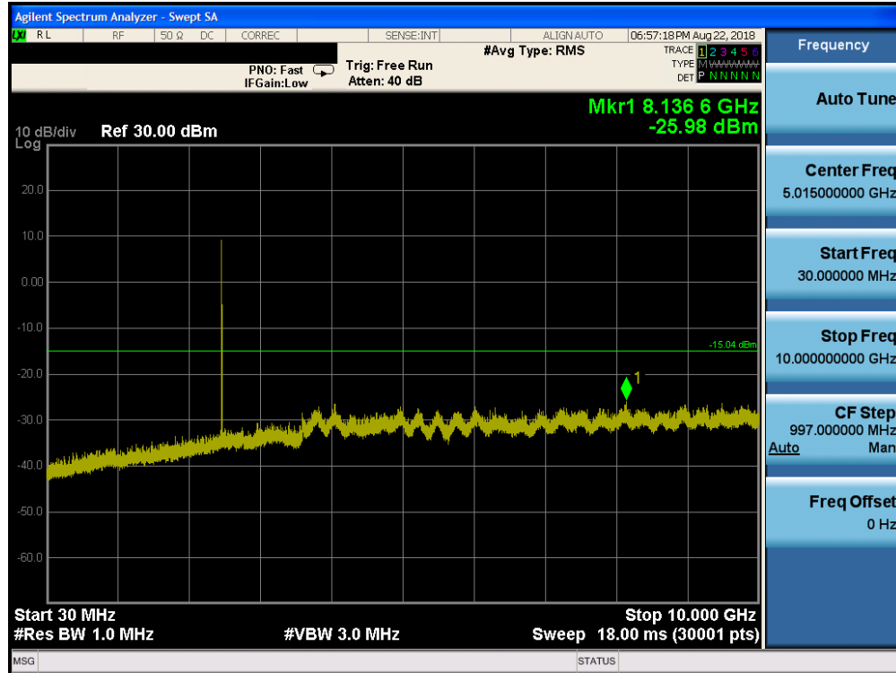
Plot 7-71. Conducted Spurious Plot ANT0 (Bluetooth (HDR4), 4Mbps, ePA – Ch. 75)
