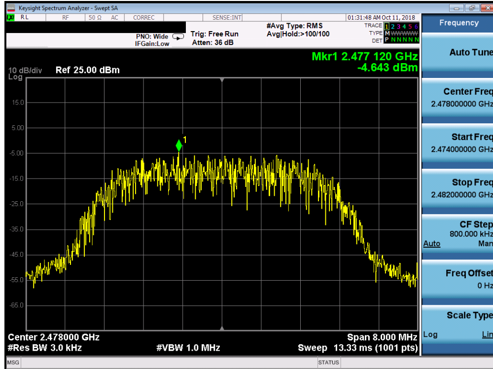
Plot 7-27. Power Spectral Density Plot ANT0 (Bluetooth (HDR8), 8Mbps, ePA – Ch. 75)
