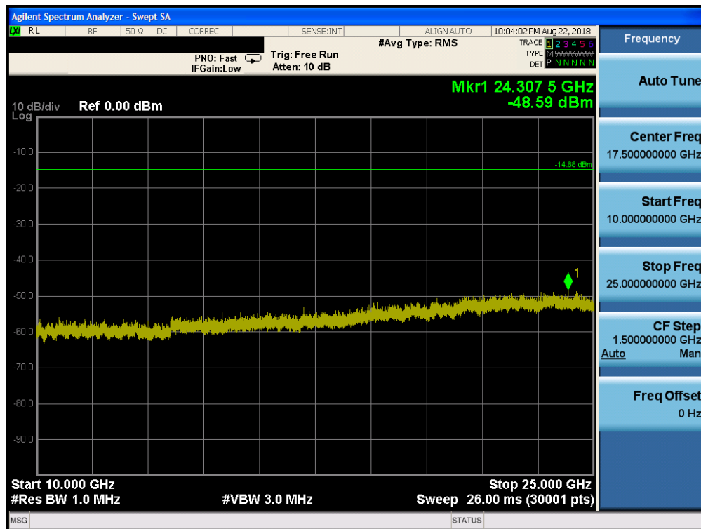
Plot 7-76. Conducted Spurious Plot ANT1 (Bluetooth (HDR4), 4Mbps, ePA – Ch. 38)
