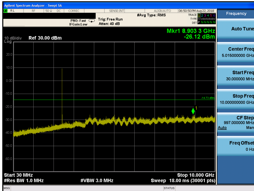
Plot 7-69. Conducted Spurious Plot ANT0 (Bluetooth (HDR4), 4Mbps, ePA – Ch. 38)
