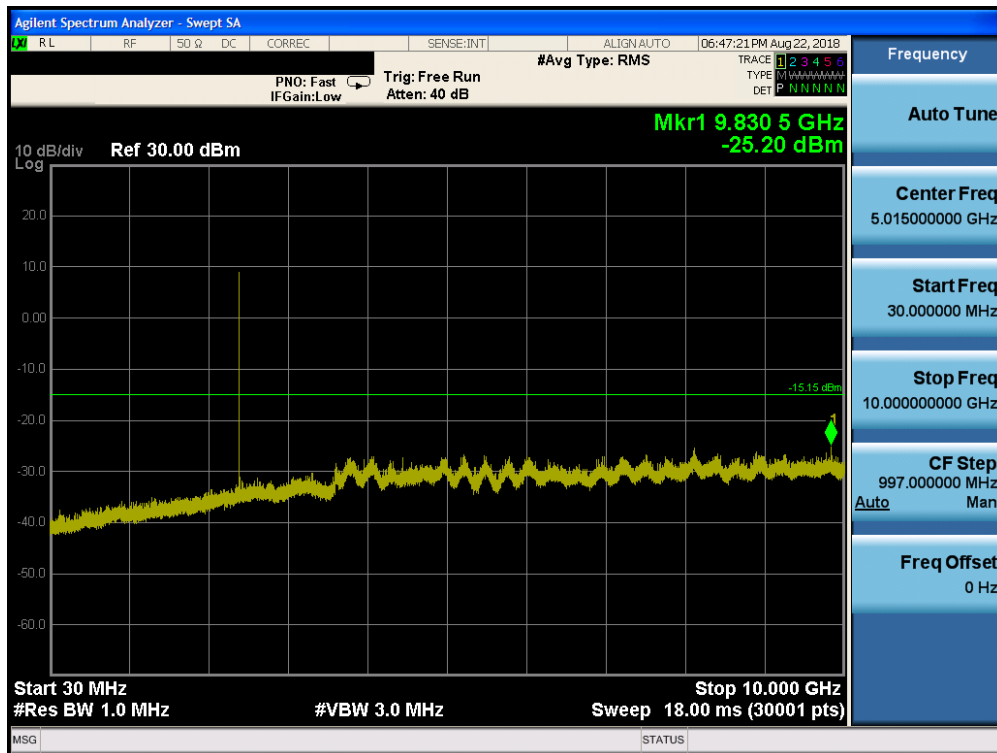
Plot 7-67. Conducted Spurious Plot ANT0 (Bluetooth (HDR4), 4Mbps, ePA – Ch. 1)
