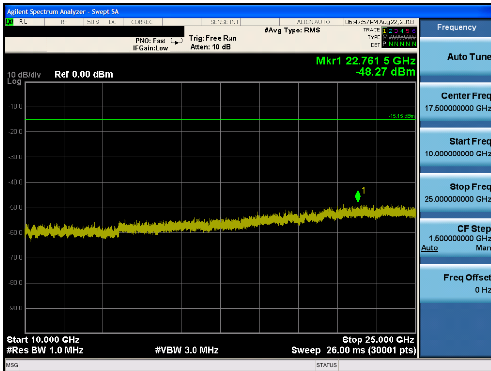
Plot 7-68. Conducted Spurious Plot ANT0 (Bluetooth (HDR4), 4Mbps, ePA – Ch. 1)
