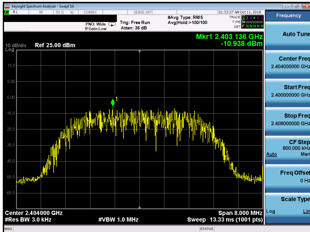
Plot 7-28. Power Spectral Density Plot ANT0 (Bluetooth (HDR8), 8Mbps, iPA – Ch. 1)
