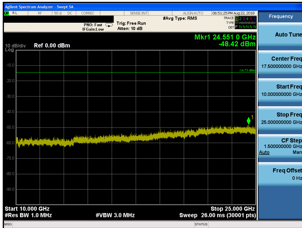
Plot 7-70. Conducted Spurious Plot ANT0 (Bluetooth (HDR4), 4Mbps, ePA – Ch. 38)
