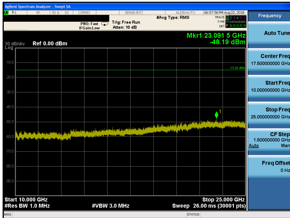
Plot 7-72. Conducted Spurious Plot ANT0 (Bluetooth (HDR4), 4Mbps, ePA – Ch. 75)
