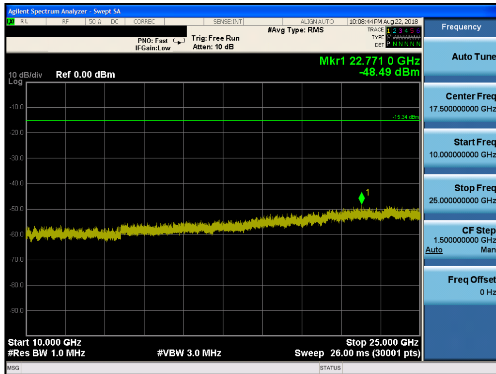
Plot 7-78. Conducted Spurious Plot ANT1 (Bluetooth (HDR4), 4Mbps, ePA – Ch. 75)
