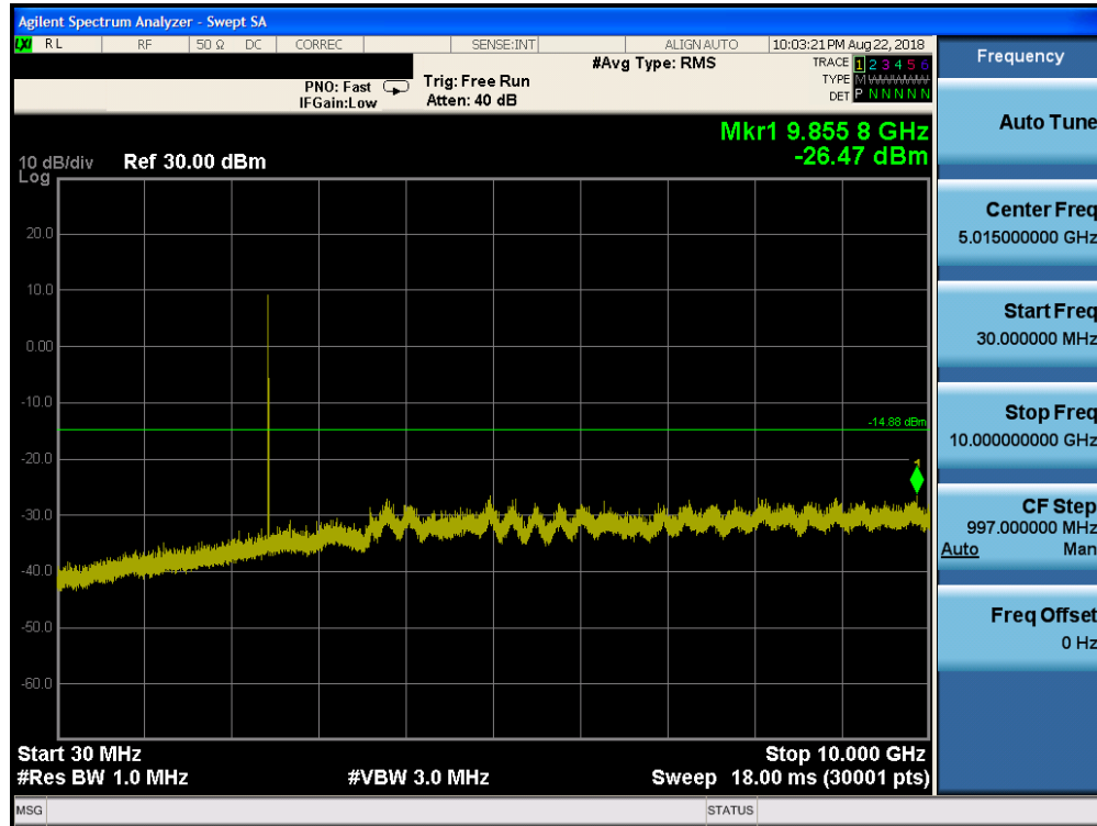
Plot 7-75. Conducted Spurious Plot ANT1 (Bluetooth (HDR4), 4Mbps, ePA – Ch. 38)
