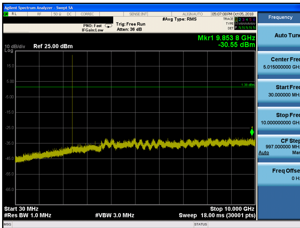
Plot 7-61. Conducted Spurious Plot (Bluetooth (LE), 1Mbps, ePA – Ch. 0, Antenna 0)
