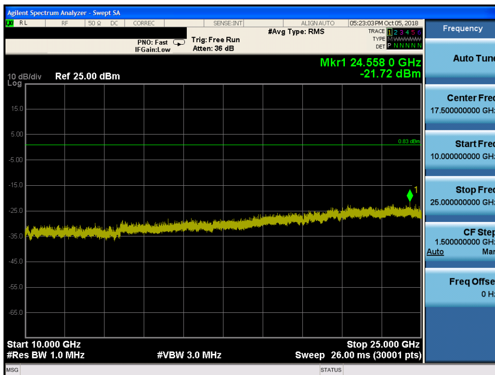
Plot 7-72. Conducted Spurious Plot (Bluetooth (LE), 1Mbps, ePA – Ch. 39, Antenna 1)
