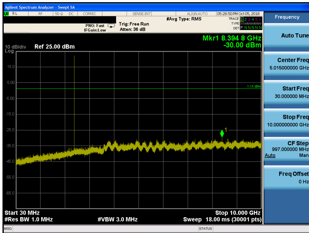
Plot 7-73. Conducted Spurious Plot (Bluetooth (LE), 1Mbps, ePA – Ch. 0, Antenna 2)
