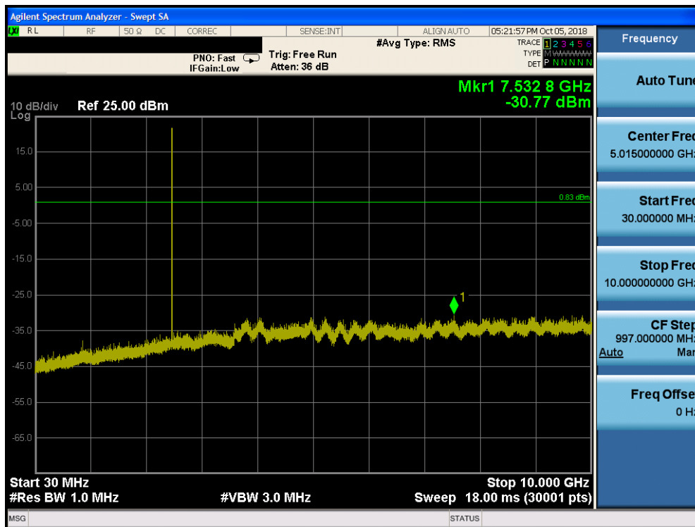
Plot 7-71. Conducted Spurious Plot (Bluetooth (LE), 1Mbps, ePA – Ch. 39, Antenna 1)
