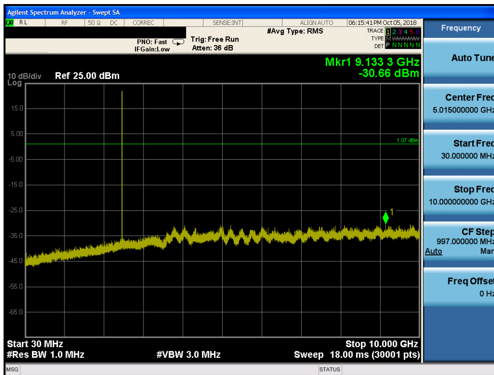
Plot 7-71. Conducted Spurious Plot ANT 0 (Bluetooth, GFSK, ePA – Ch. 78)
