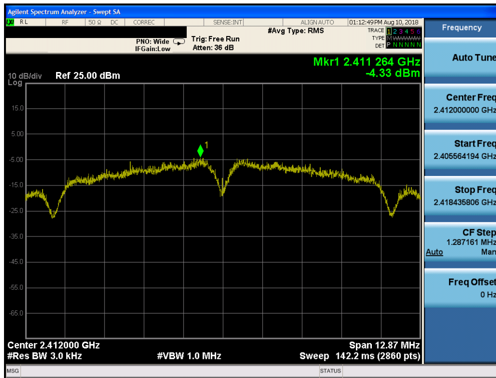
Plot 7-37. Power Spectral Density Plot SISO Core 1 Primary (802.11b – Ch. 1)
