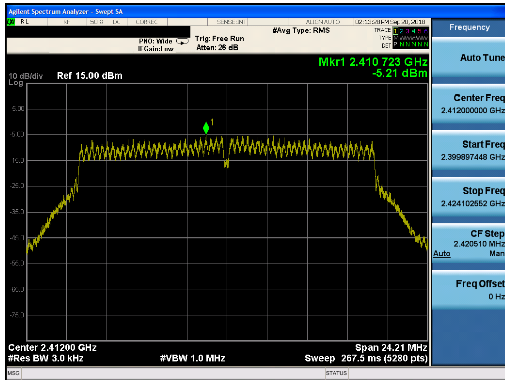
Plot 7-62. Power Spectral Density Plot CDD Core 1 Primary (802.11n – Ch. 1)
