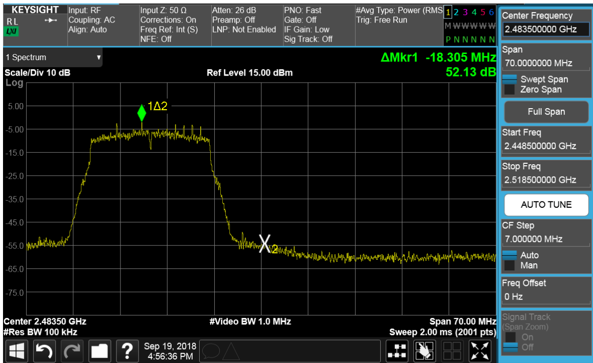
Plot 7-89. Band Edge Plot SISO Core 0 (11n (2.4GHz) – Ch. 12)
