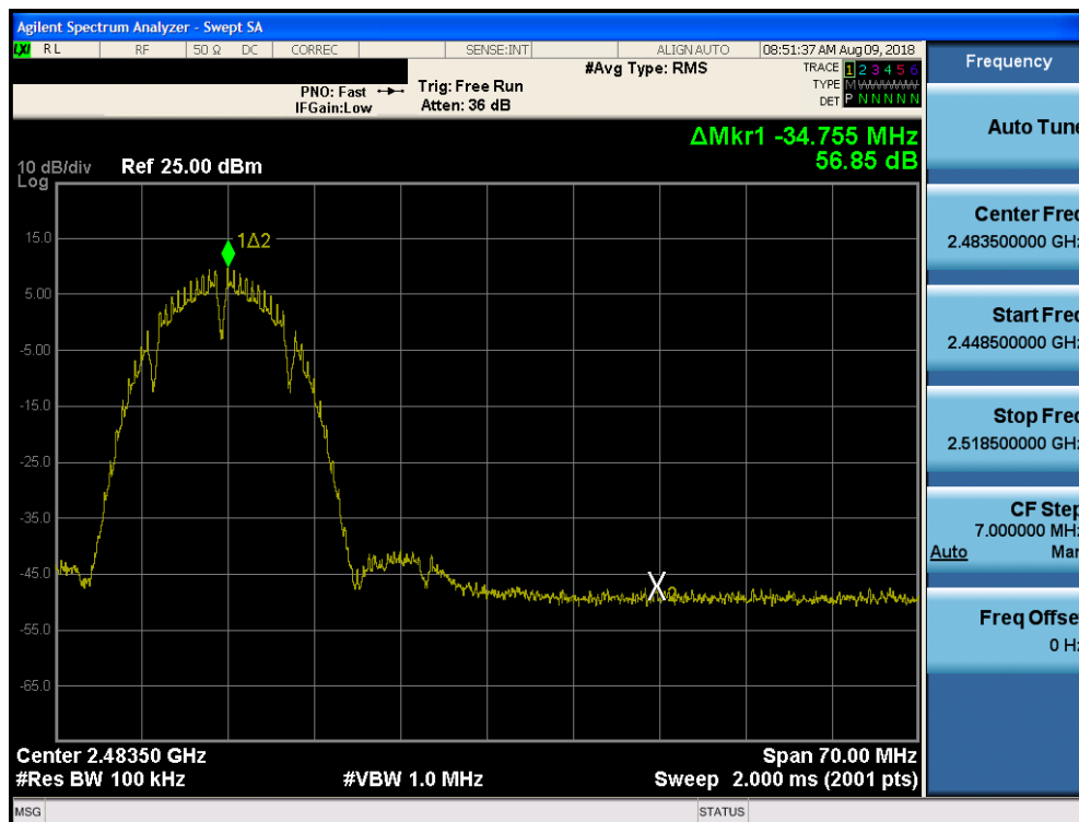
Plot 7-80. Band Edge Plot SISO Core 0 (802.11b – Ch. 11)
