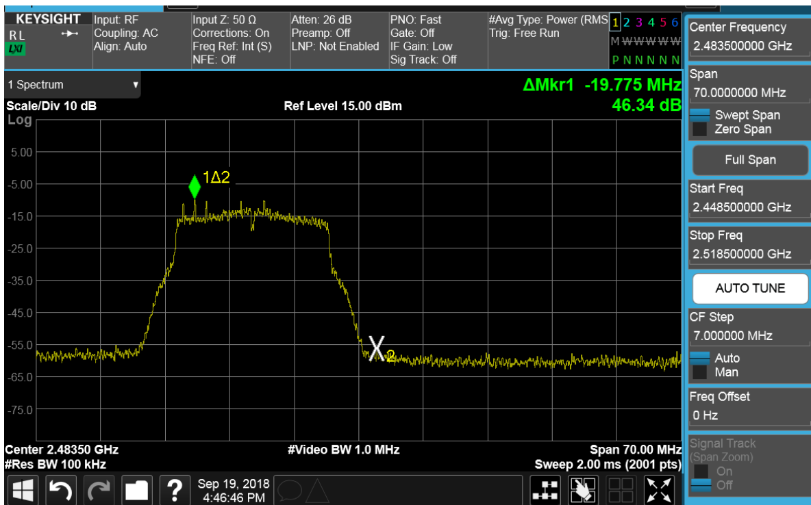
Plot 7-86. Band Edge Plot SISO Core 0 (802.11g – Ch. 13)
