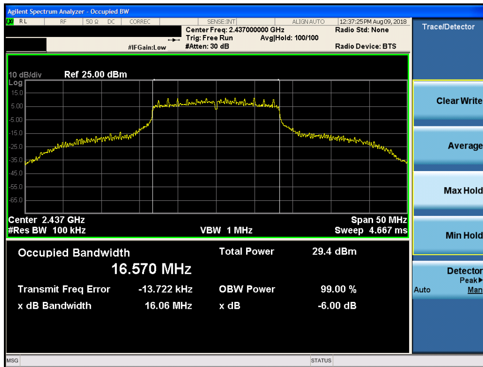
Plot 7-23. 6dB Bandwidth Plot SISO Core 1 Diversity (802.11g – Ch. 6)
