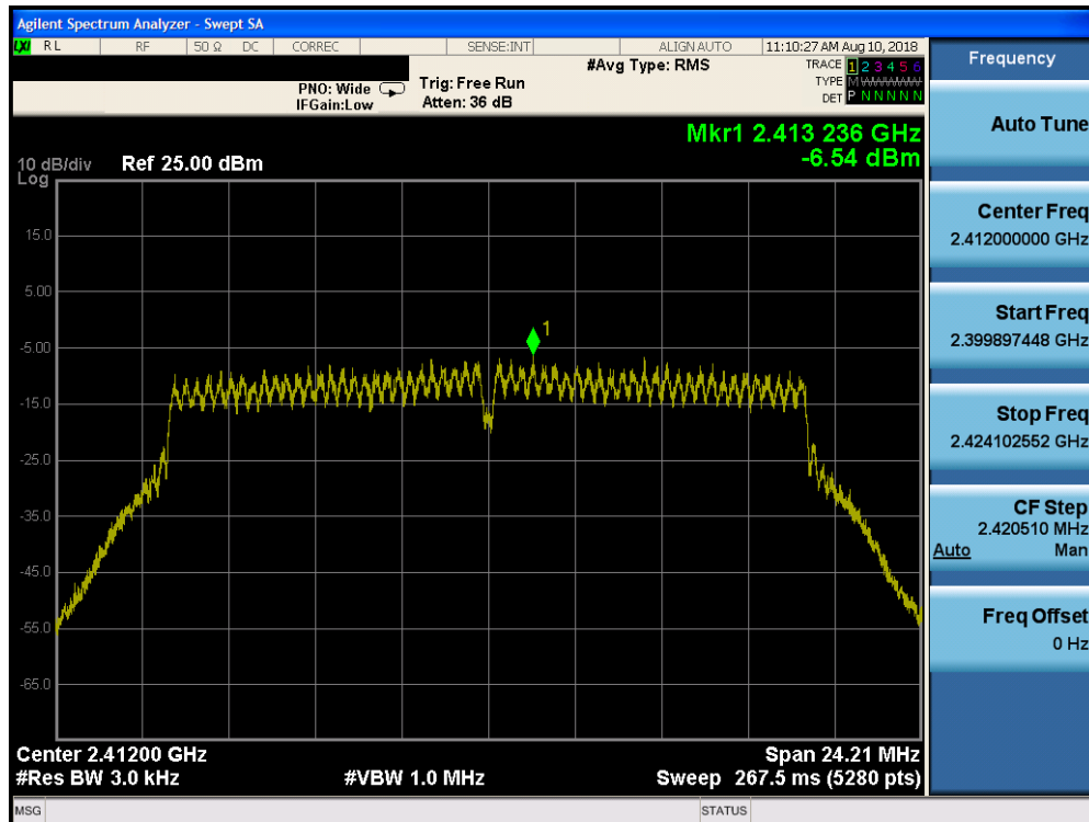
Plot 7-43. Power Spectral Density Plot SISO Core 1 Primary (802.11n (2.4GHz) – Ch. 1)
