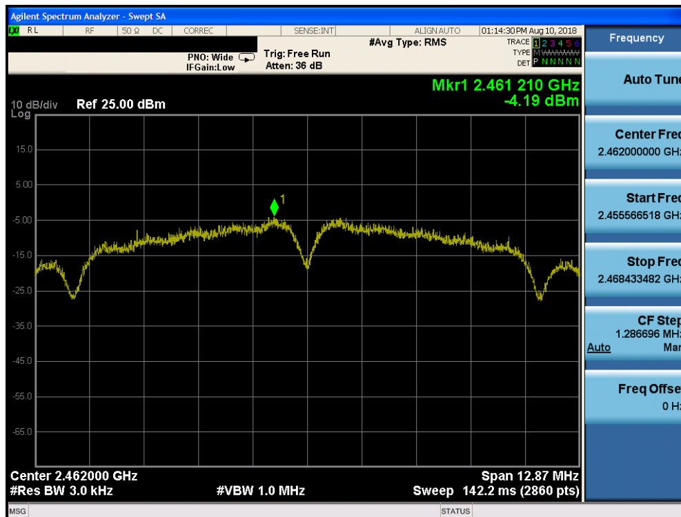
Plot 7-39. Power Spectral Density Plot SISO Core 1 Primary (802.11b – Ch. 11)
