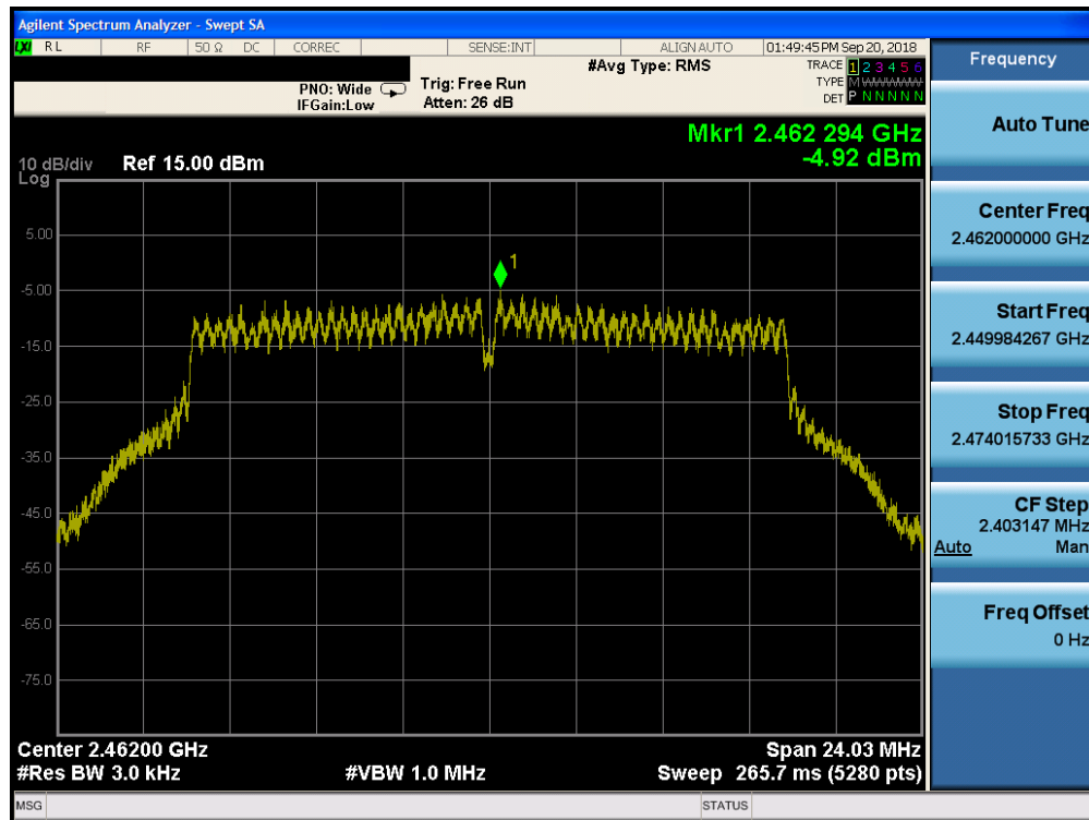
Plot 7-72. Power Spectral Density Plot CDD Core 1 Diversity (802.11g – Ch. 11)
