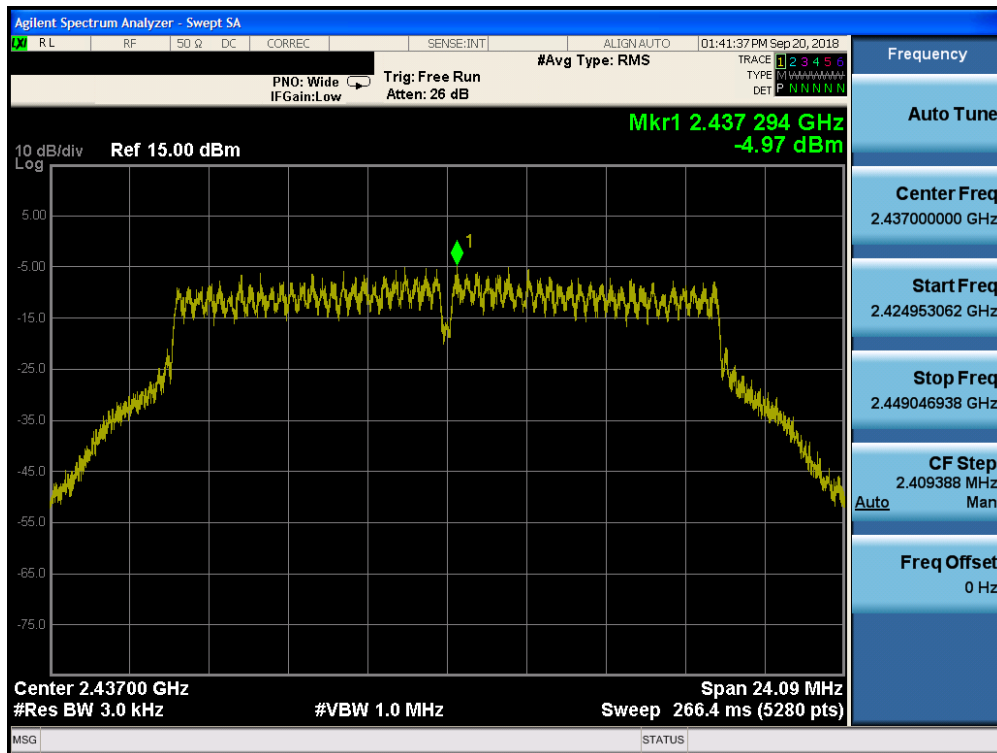
Plot 7-69. Power Spectral Density Plot CDD Core 0 (802.11g – Ch. 6)
