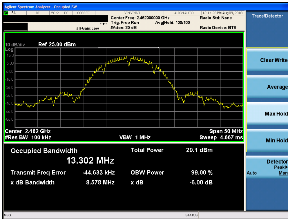
Plot 7-21. 6dB Bandwidth Plot SISO Core 1 Diversity (802.11b – Ch. 11)
