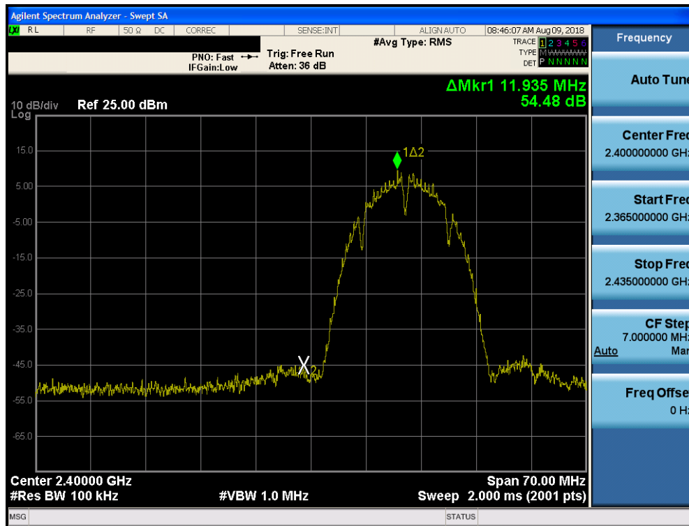
Plot 7-79. Band Edge Plot SISO Core 0 (802.11b – Ch. 1)
