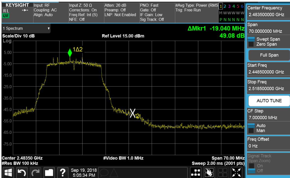
Plot 7-97. Band Edge Plot SISO Core 1 Primary (802.11g- Ch. 12)
