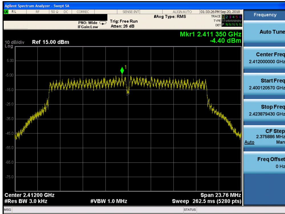
Plot 7-56. Power Spectral Density Plot CDD Core 1 Primary (802.11g – Ch. 1)
