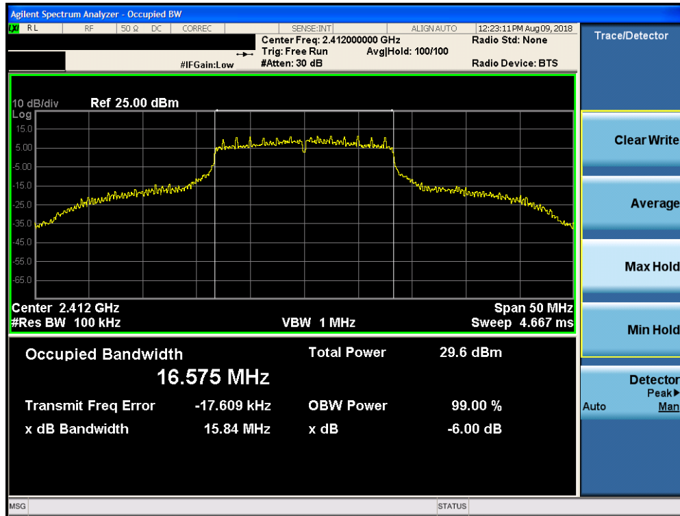
Plot 7-22. 6dB Bandwidth Plot Core 1 Diversity (802.11g – Ch. 1)
