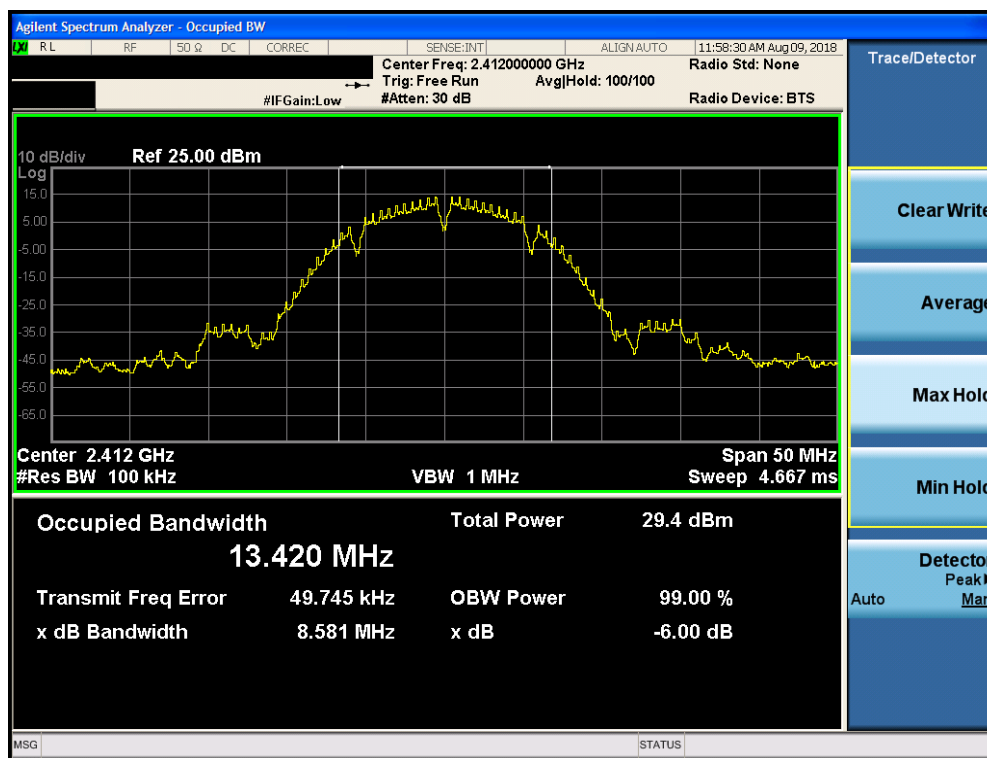
Plot 7-19. 6dB Bandwidth Plot SISO Core 1 Diversity (802.11b – Ch. 1)
