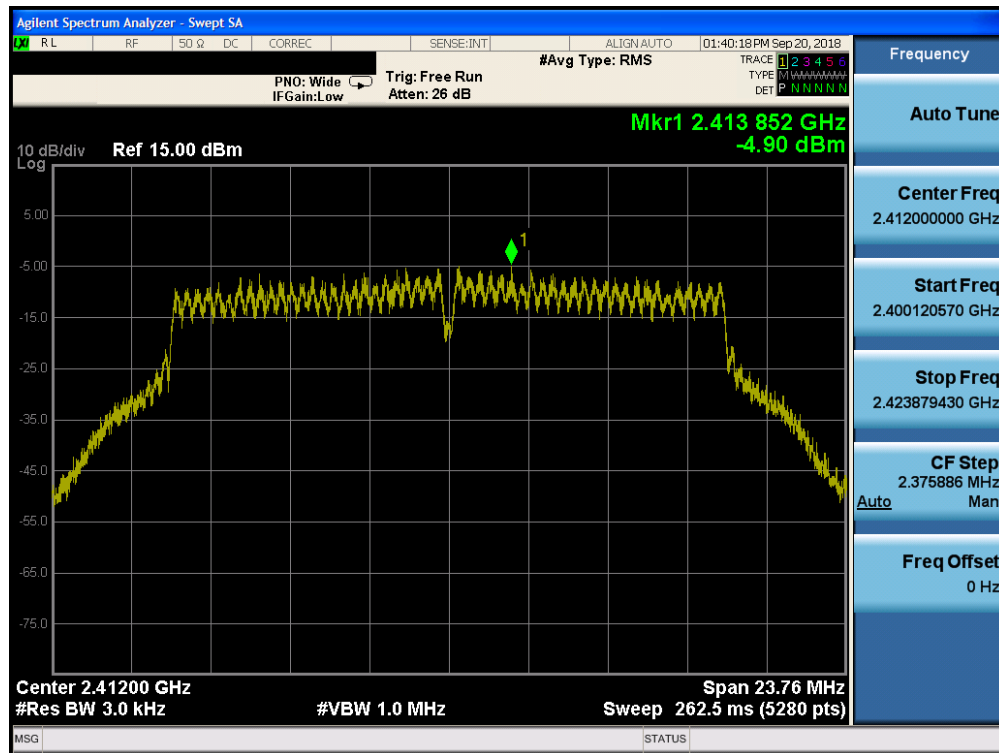
Plot 7-67. Power Spectral Density Plot CDD Core 0 (802.11g – Ch. 1)
