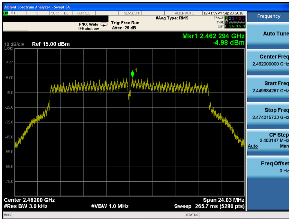
Plot 7-59. Power Spectral Density Plot CDD Core 0 (802.11g – Ch. 11)
