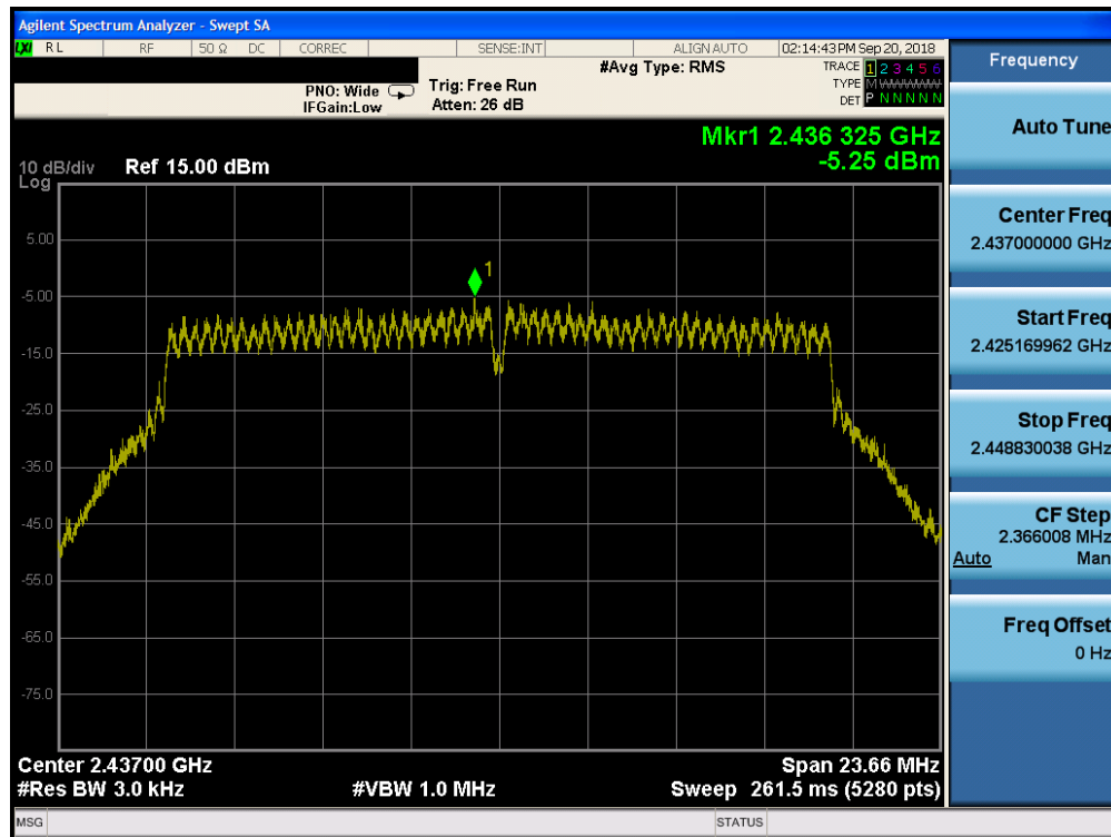
Plot 7-64. Power Spectral Density Plot CDD Core 1 Primary (802.11n – Ch. 6)
