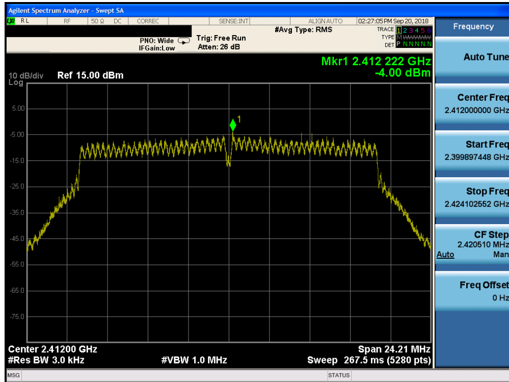
Plot 7-74. Power Spectral Density Plot CDD Core 1 Diversity (802.11n – Ch. 1)
