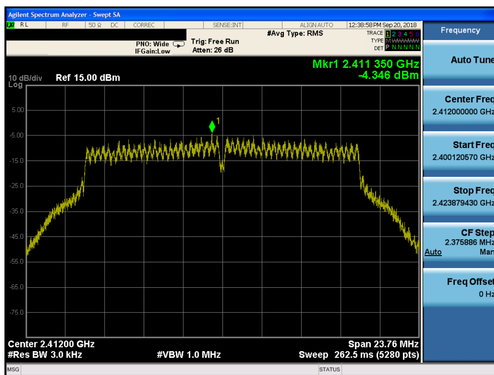
Plot 7-55. Power Spectral Density Plot CDD Core 0 (802.11g – Ch. 1)
