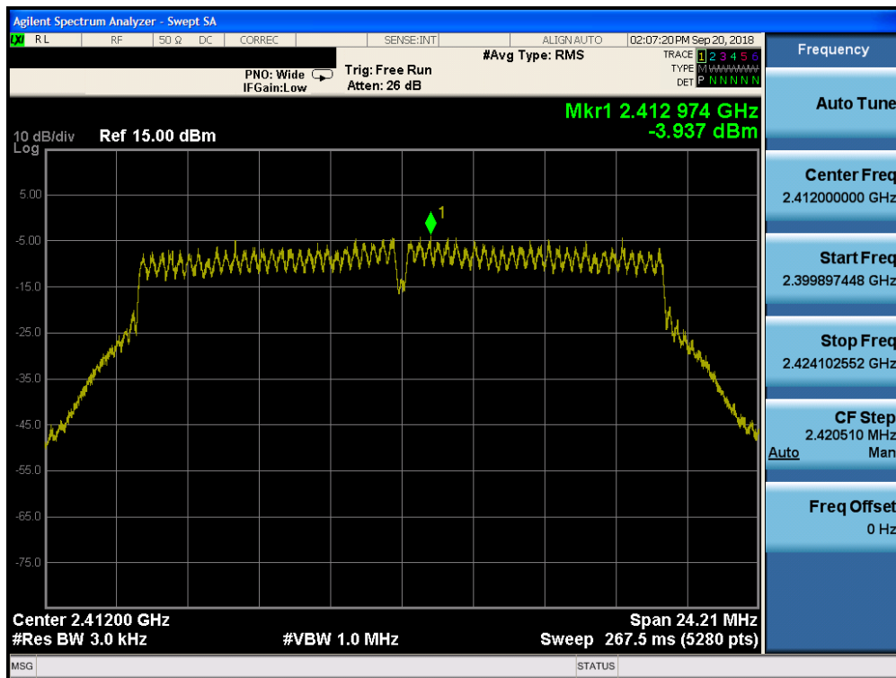
Plot 7-61. Power Spectral Density Plot CDD Core 0 (802.11n – Ch. 1)
