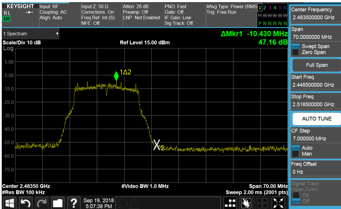
Plot 7-98. Band Edge Plot SISO Core 1 Primary (802.11g - Ch. 13)
