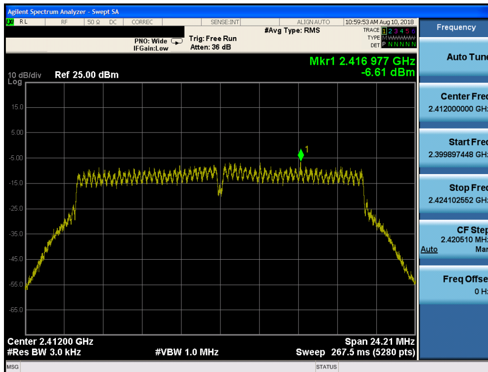
Plot 7-34. Power Spectral Density Plot SISO Core 0 (802.11n (2.4GHz) – Ch. 1)
