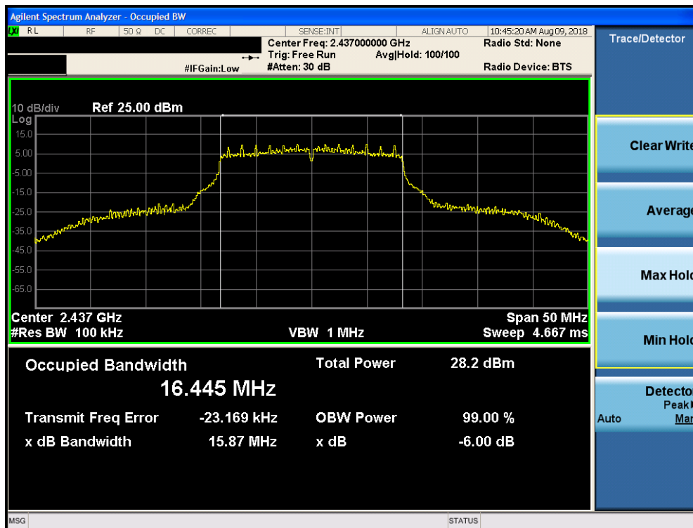
Plot 7-14. 6dB Bandwidth Plot SISO Core 1 Primary (802.11g – Ch. 6)
