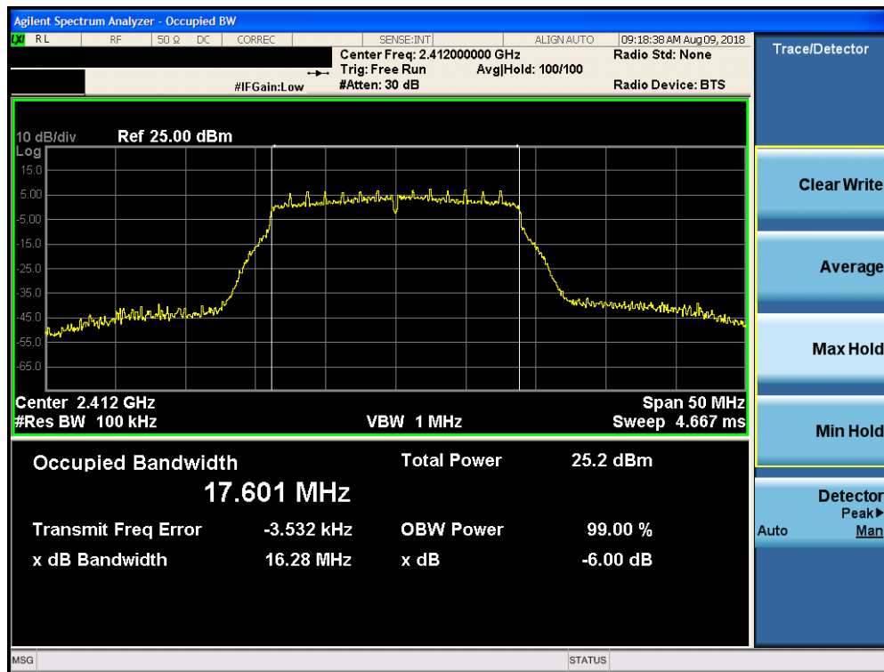
Plot 7-7. 6dB Bandwidth Plot SISO Core 0 (802.11n (2.4GHz) – Ch. 1)
