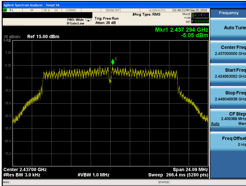
Plot 7-70. Power Spectral Density Plot CDD Core 1 Diversity (802.11g – Ch. 6)
