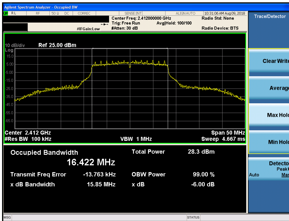
Plot 7-13. 6dB Bandwidth Plot Core 1 Primary (802.11g – Ch. 1)
