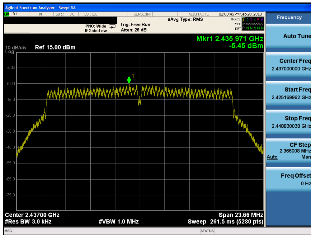
Plot 7-63. Power Spectral Density Plot CDD Core 0 (802.11n – Ch. 6)
