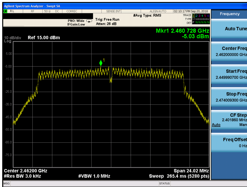
Plot 7-65. Power Spectral Density Plot CDD Core 0 (802.11n – Ch. 11)
