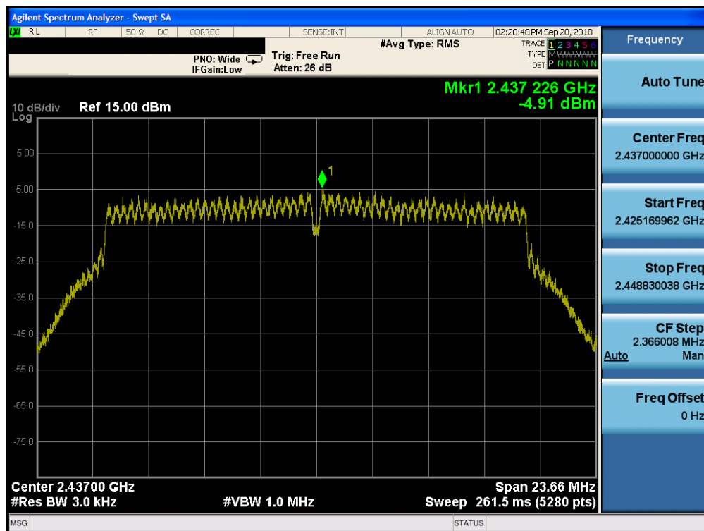
Plot 7-75. Power Spectral Density Plot CDD Core 0 (802.11n – Ch. 6)
