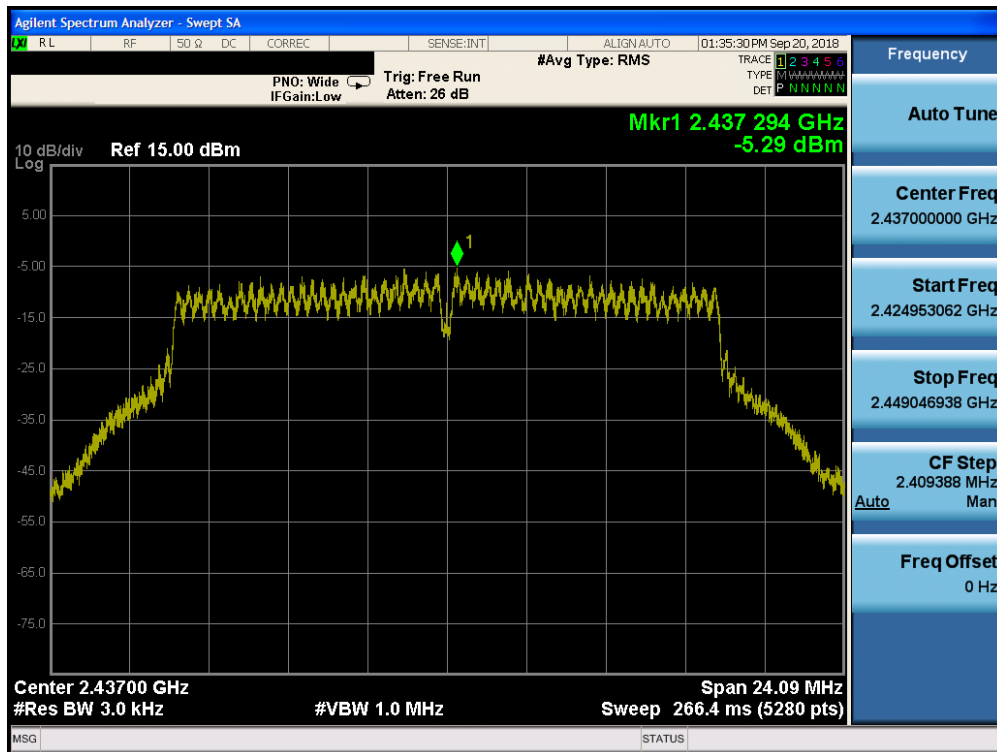
Plot 7-58. Power Spectral Density Plot CDD Core 1 Primary (802.11g – Ch. 6)
