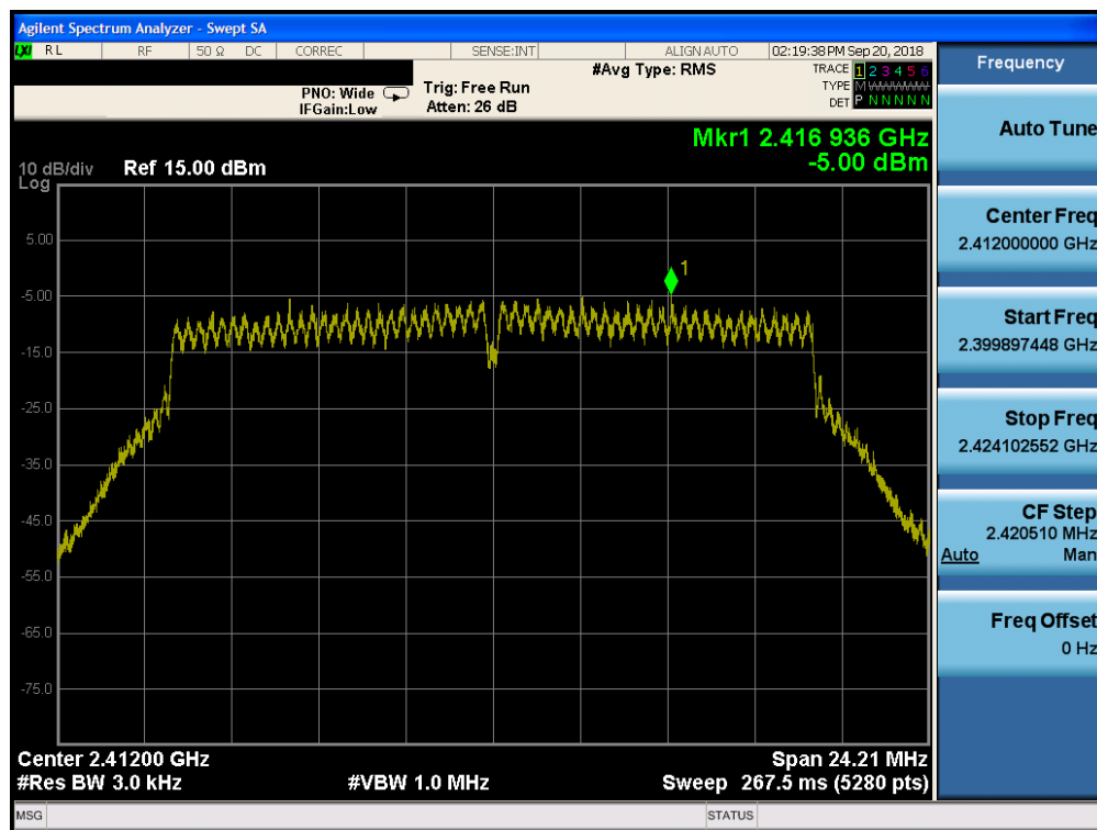
Plot 7-73. Power Spectral Density Plot CDD Core 0 (802.11n – Ch. 1)
