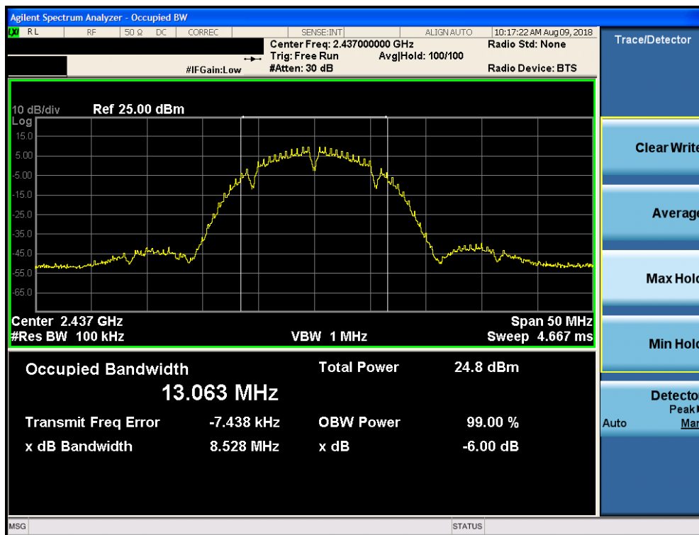
Plot 7-11. 6dB Bandwidth Plot SISO Core 1 Primary (802.11b – Ch. 6)
