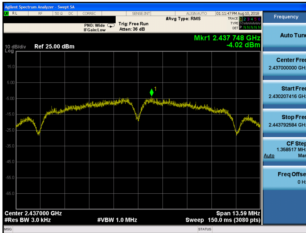
Plot 7-38. Power Spectral Density Plot SISO Core 1 Primary (802.11b – Ch. 6)
