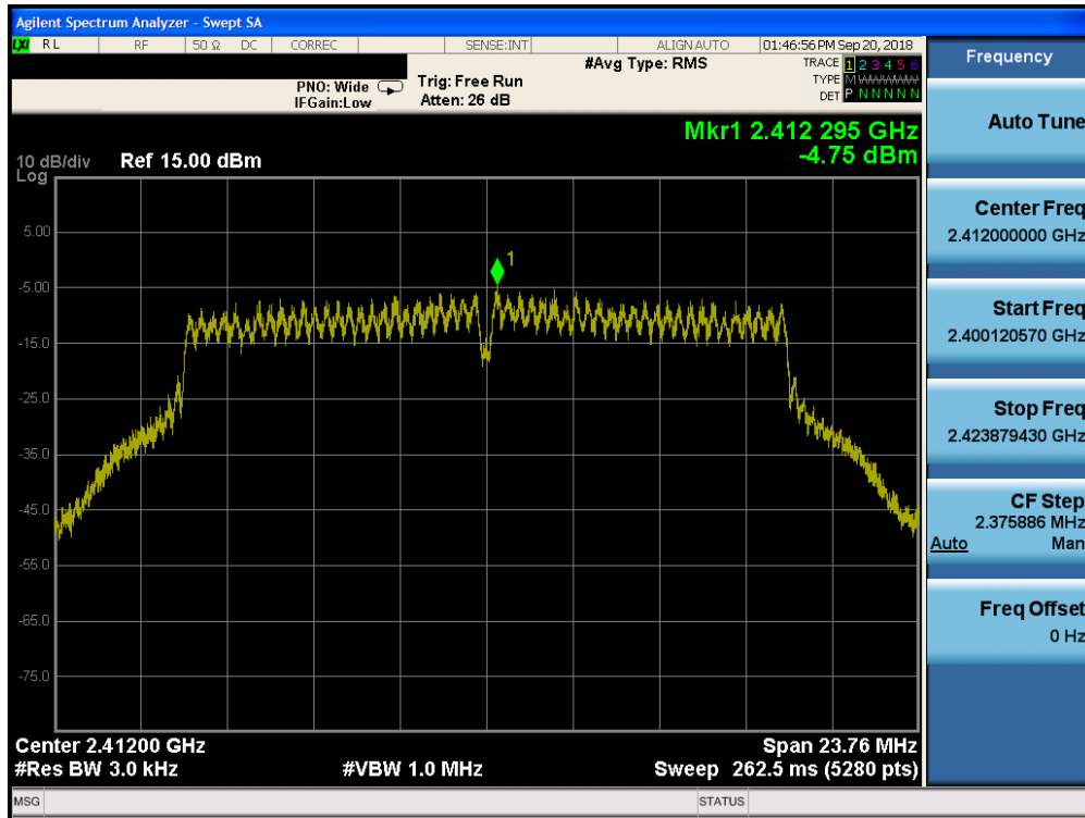
Plot 7-68. Power Spectral Density Plot CDD Core 1 Diversity (802.11g – Ch. 1)
