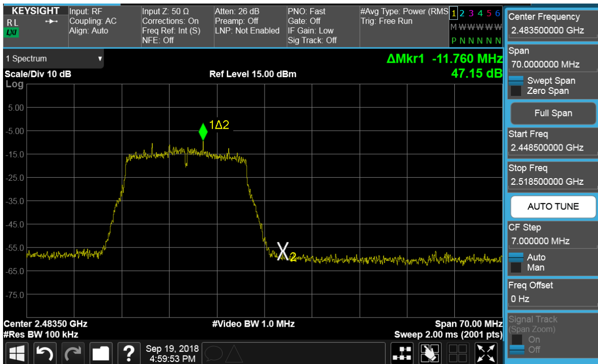
Plot 7-90. Band Edge Plot SISO Core 0 (11n (2.4GHz) – Ch. 13)
