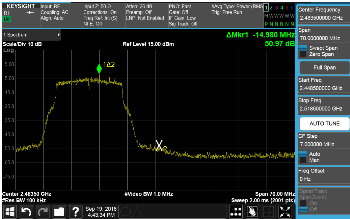
Plot 7-85. Band Edge Plot SISO Core 0 (802.11g – Ch. 12)
