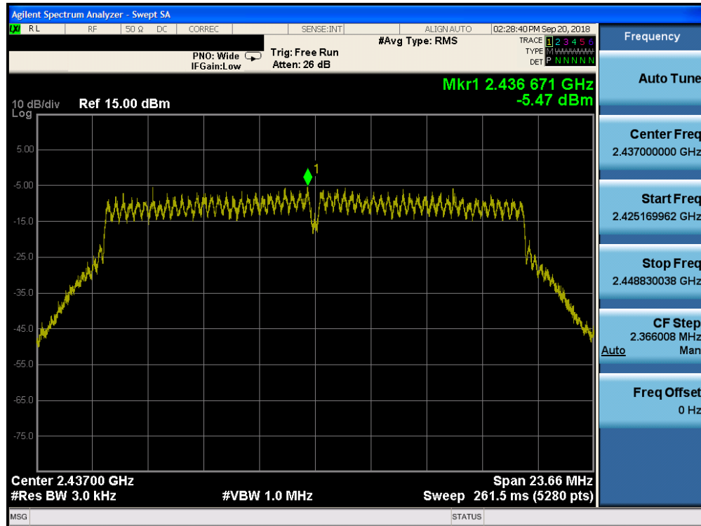
Plot 7-76. Power Spectral Density Plot CDD Core 1 Diversity (802.11n – Ch. 6)
