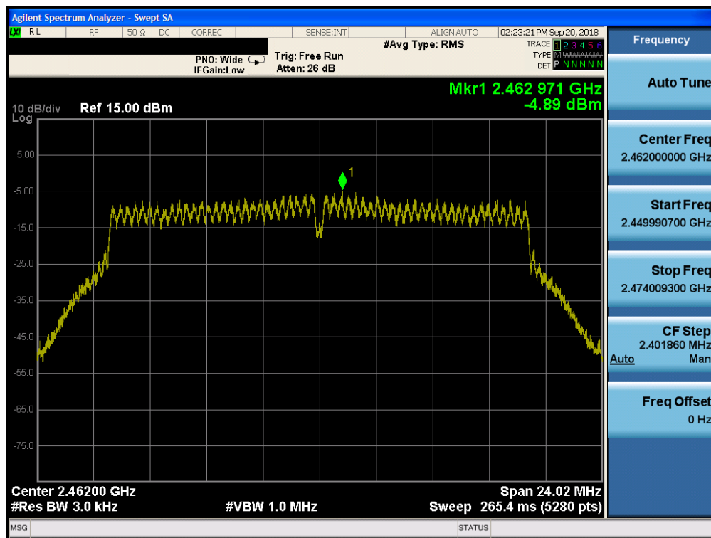
Plot 7-77. Power Spectral Density Plot CDD Core 0 (802.11n – Ch. 11)
