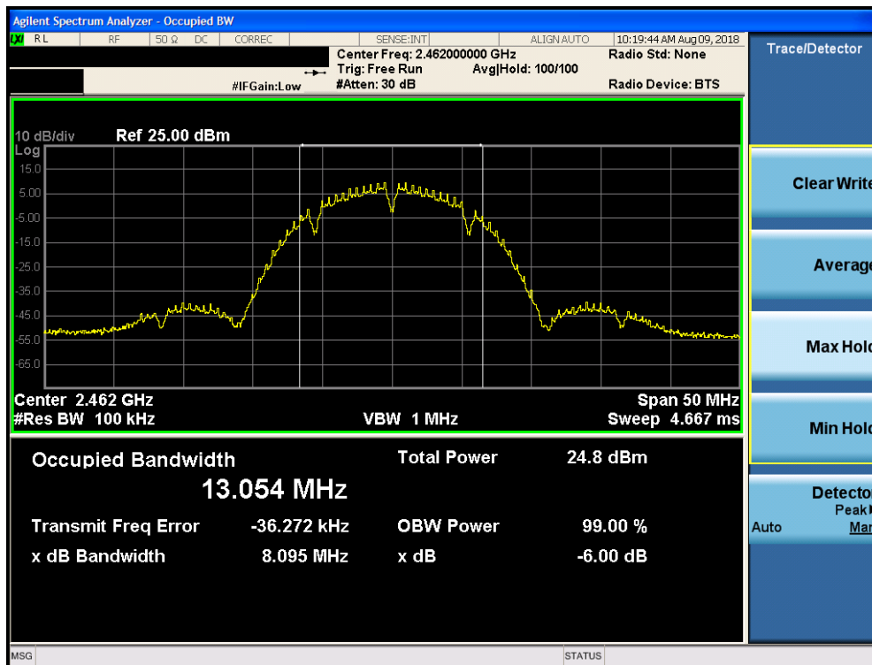
Plot 7-12. 6dB Bandwidth Plot SISO Core 1 Primary (802.11b – Ch. 11)
