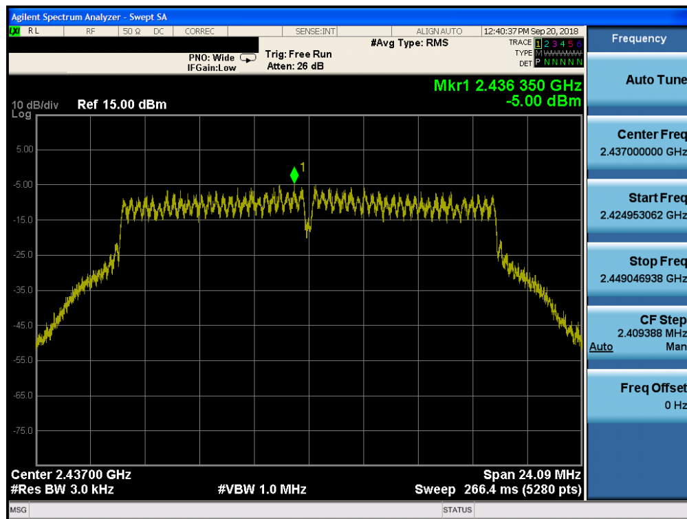
Plot 7-57. Power Spectral Density Plot CDD Core 0 (802.11g – Ch. 6)
