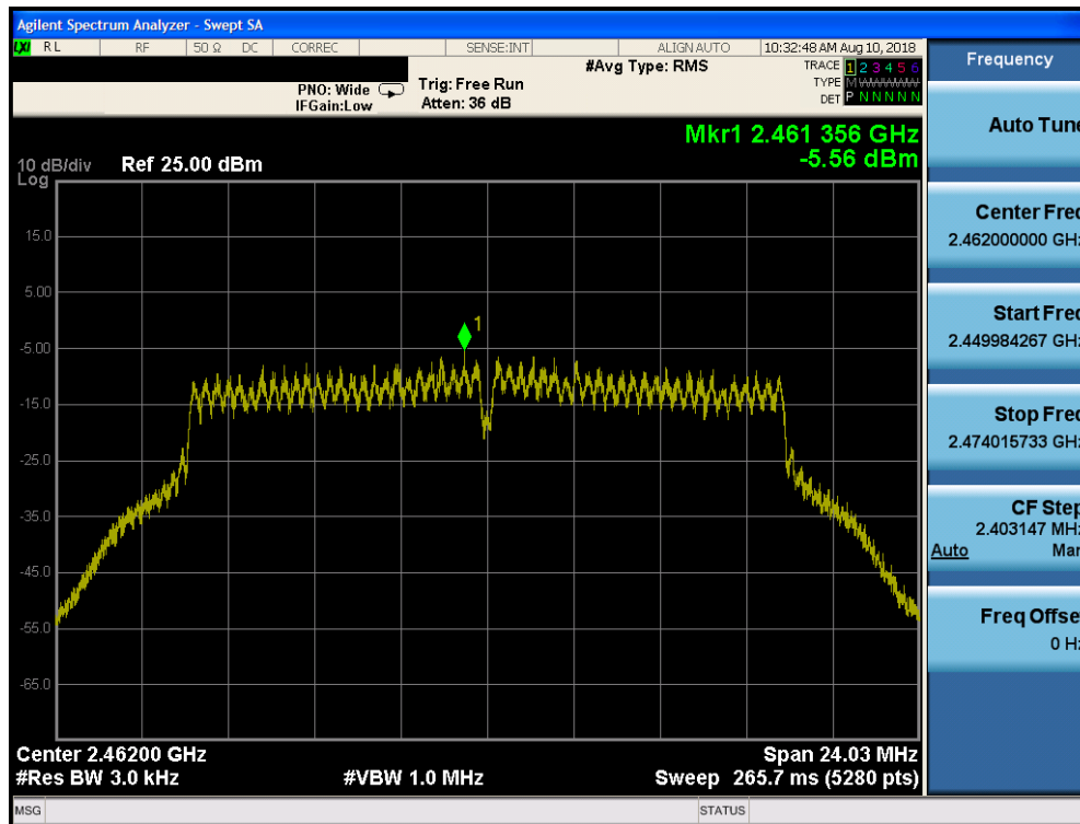
Plot 7-33. Power Spectral Density Plot SISO Core 0 (802.11g – Ch. 11)
