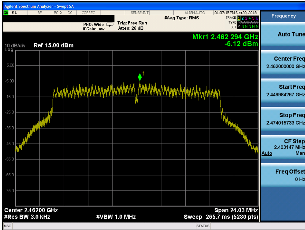
Plot 7-60. Power Spectral Density Plot CDD Core 1 Primary (802.11g – Ch. 11)
