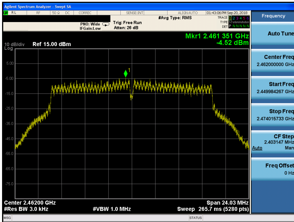
Plot 7-71. Power Spectral Density Plot CDD Core 0 (802.11g – Ch. 11)
