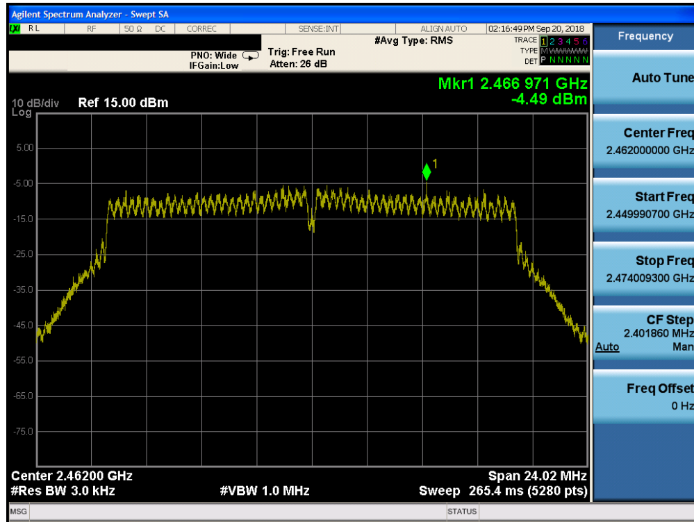
Plot 7-66. Power Spectral Density Plot CDD Core 1 Primary (802.11n – Ch. 11)
