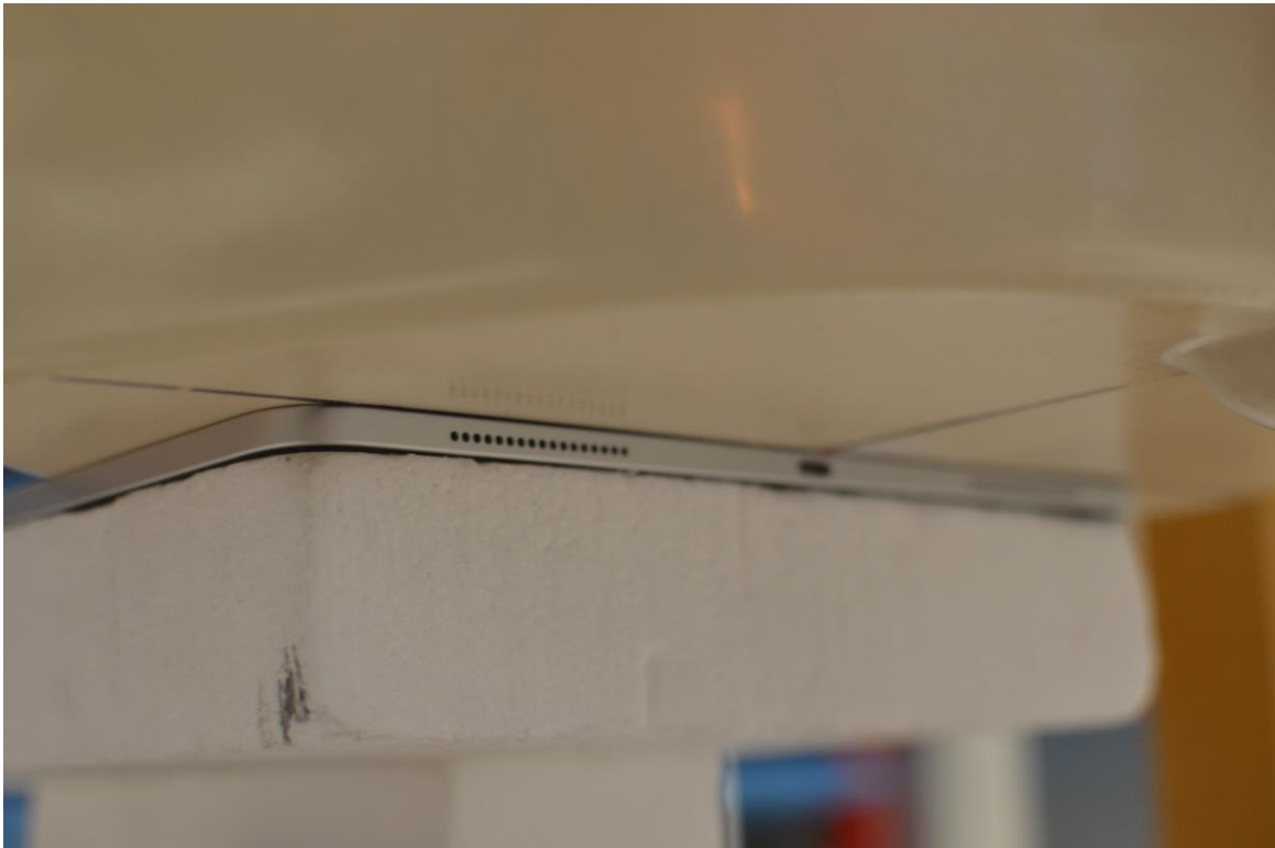
SAR Test Setup Photo 1: Back Side at 0 mm (for Antenna Lower testing)
