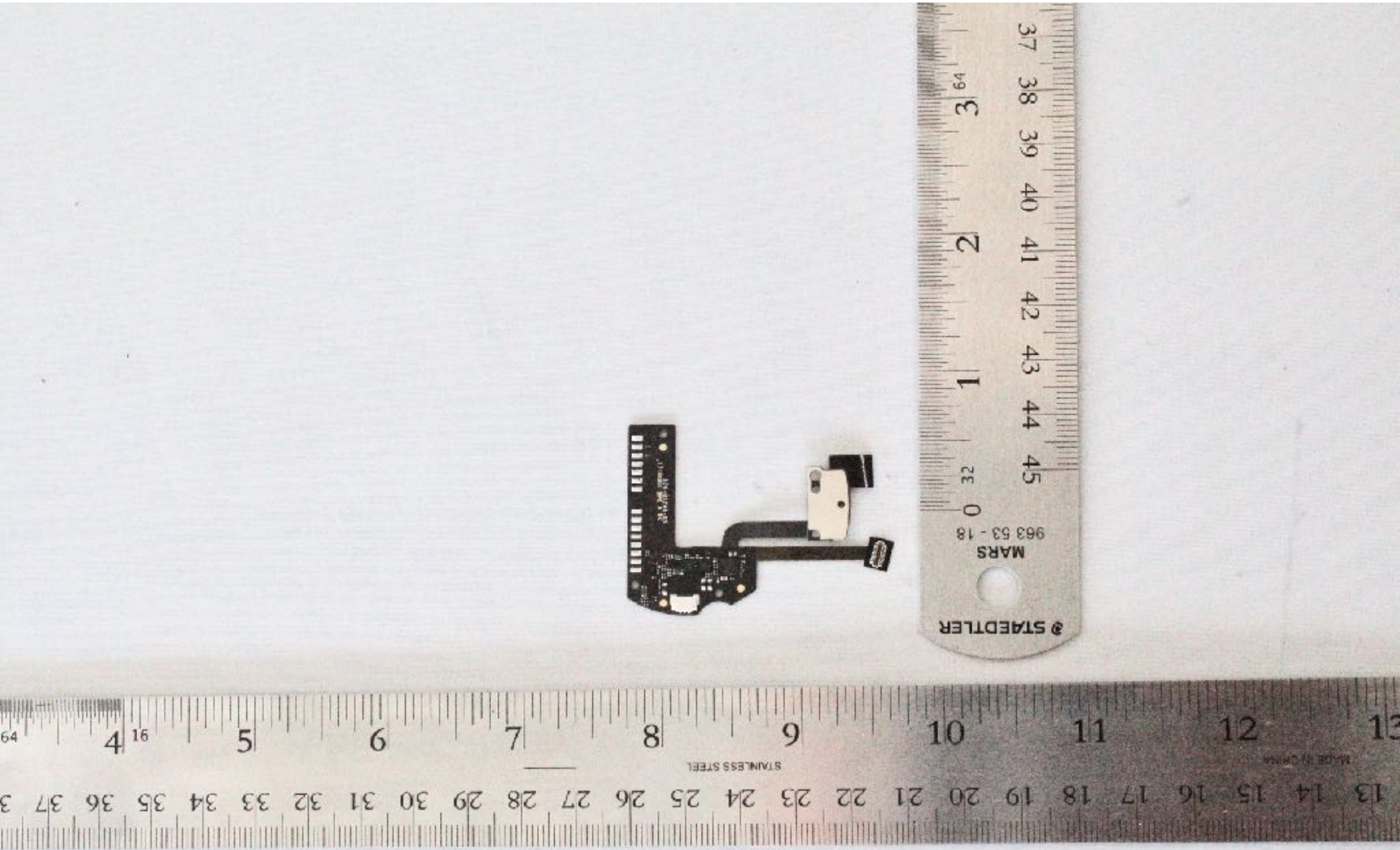
Front View of the Flex Cable
