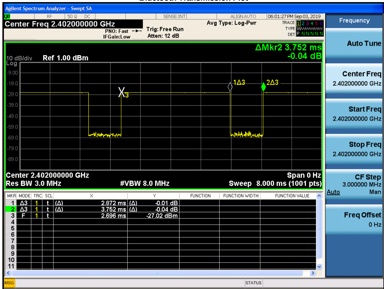
Equation 7-1 Bluetooth Duty Cycle Calculation
