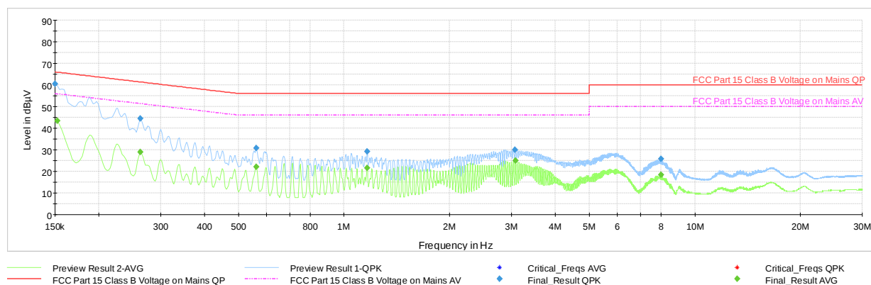
Plot 7-45. AC Line-Conducted Test Plot – GFSK Ch.39 (L1, with Laptop)
