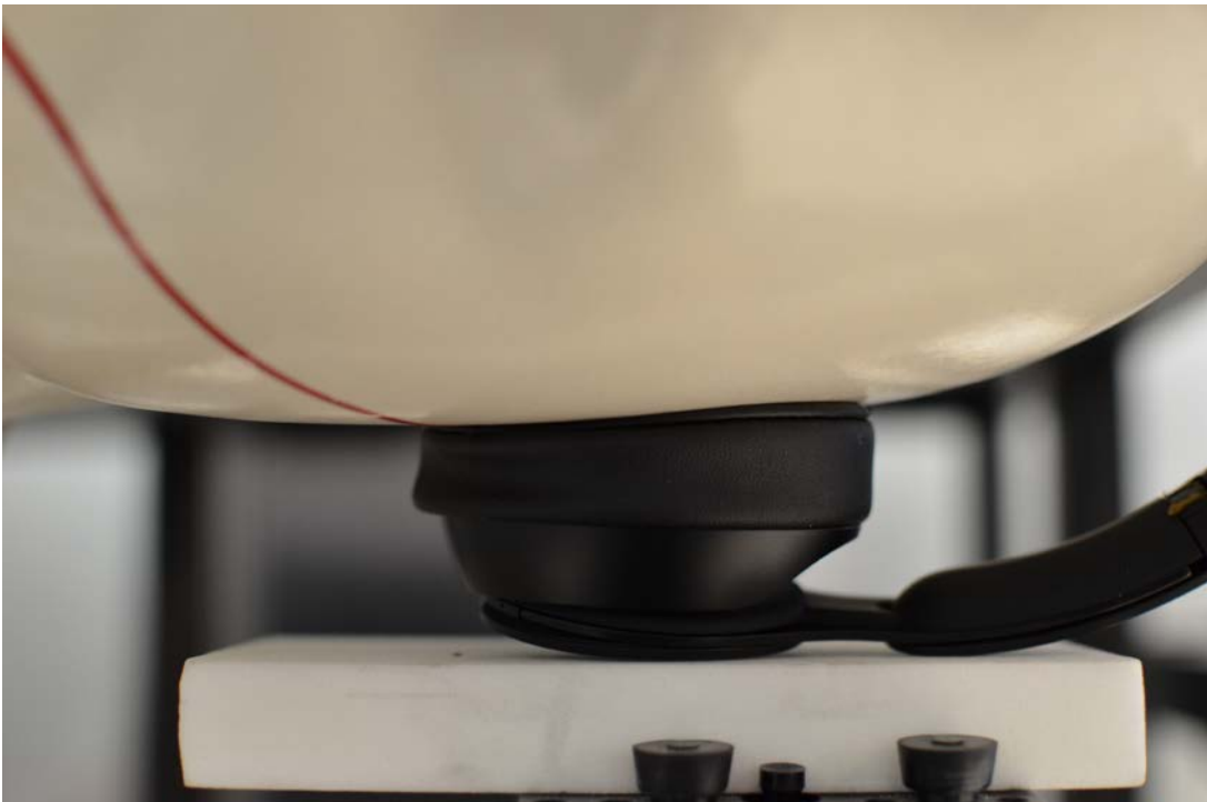
SAR Test Setup Photo 2: Left Head SAR Cushion Side at 0.0 cm
