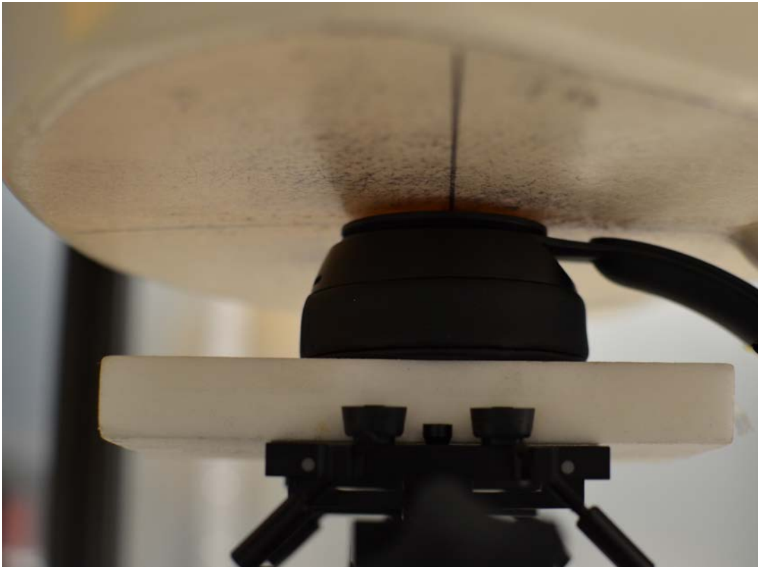
SAR Test Setup Photo 3: Extremity SAR Logo side at 0.0 cm
