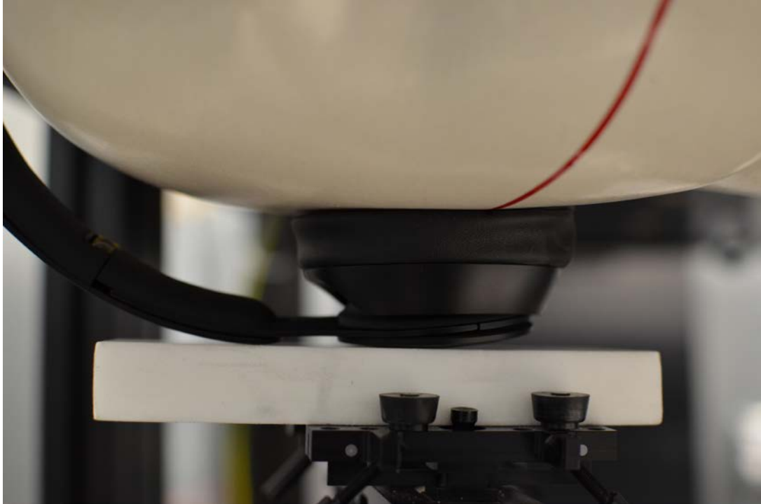
SAR Test Setup Photo 1: Right Head SAR Cushion Side at 0.0 cm
