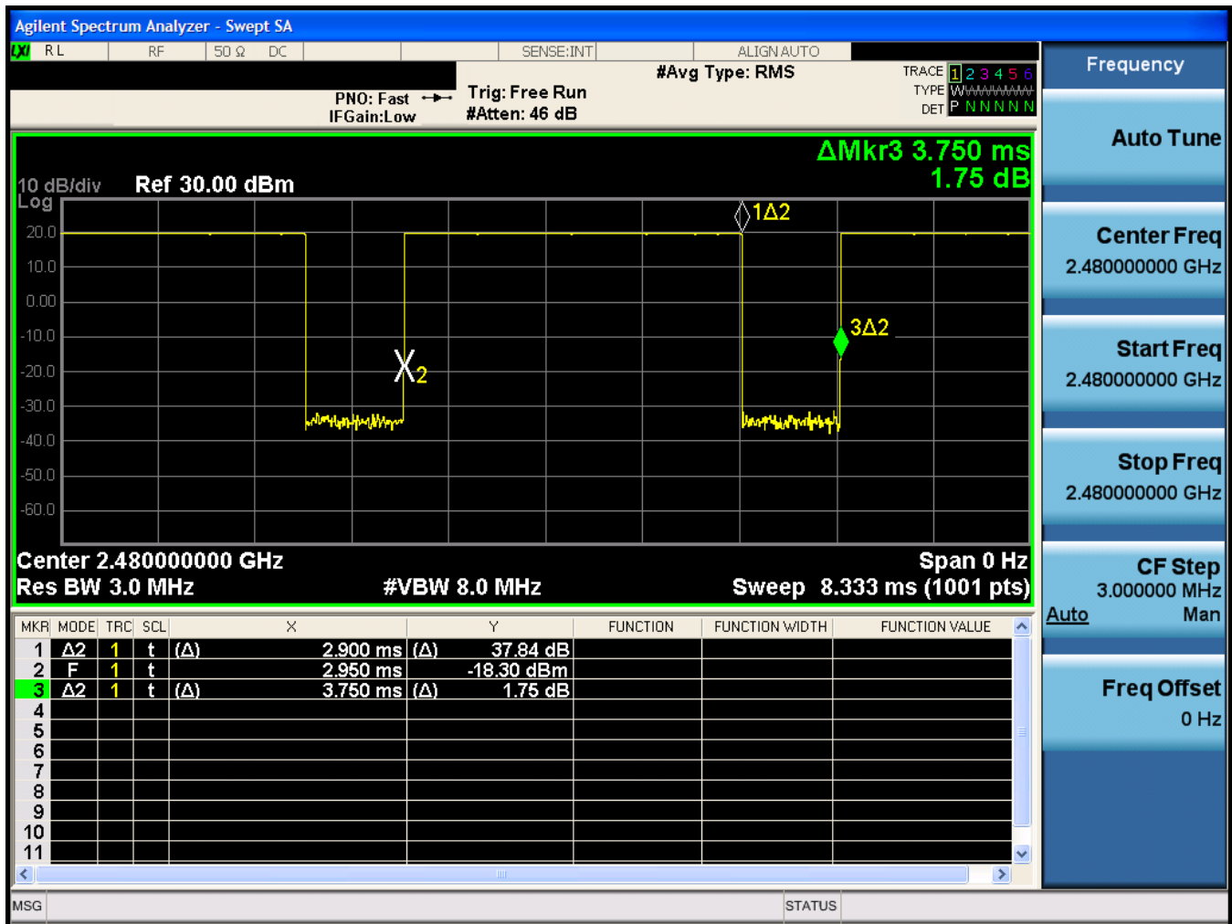
Figure 7-2 Bluetooth P High Transmission Plot & Duty Cycle Calculation – Variant 1
