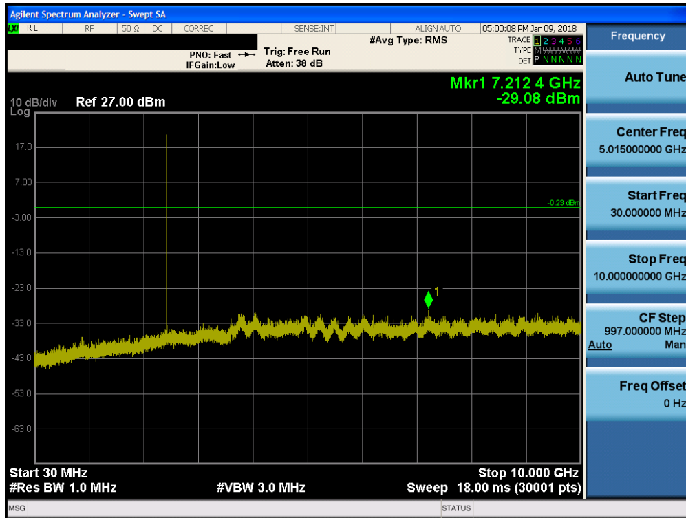
Plot 7-19. Conducted Spurious Plot (Bluetooth (LE), ePA – Ch. 19)
