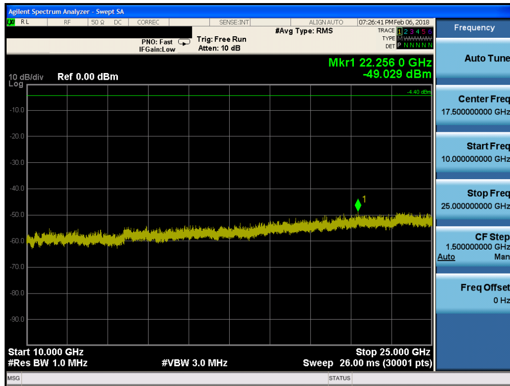
Plot 7-18. Conducted Spurious Plot (Bluetooth (LE), ePA – Ch. 0)
