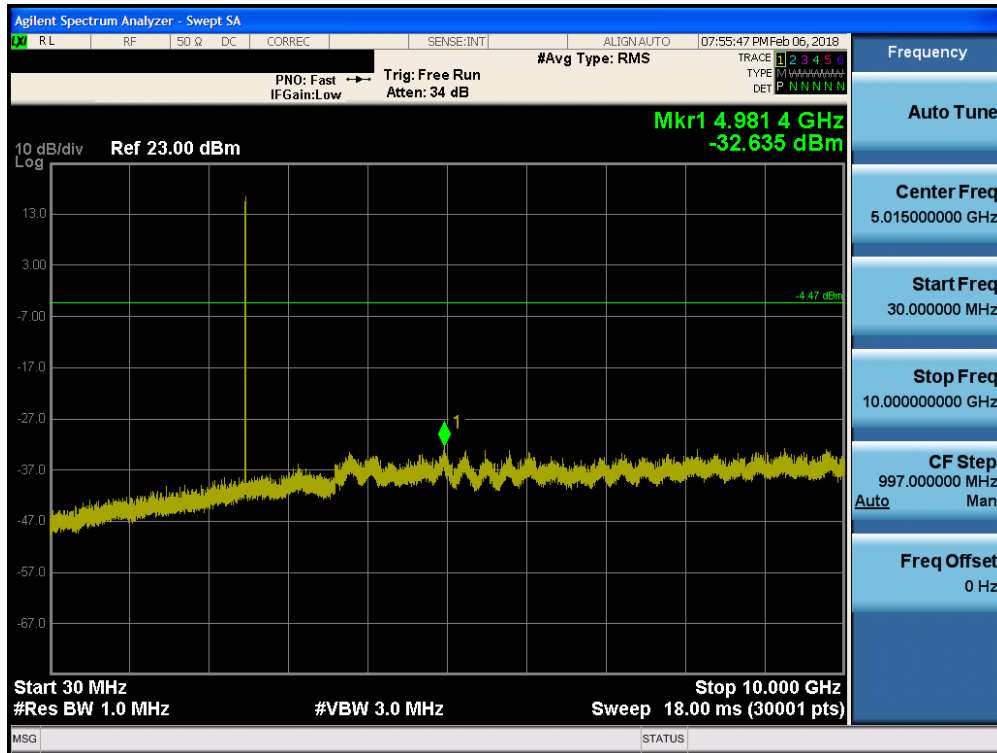
Plot 7-21. Conducted Spurious Plot (Bluetooth (LE), ePA – Ch. 39)
