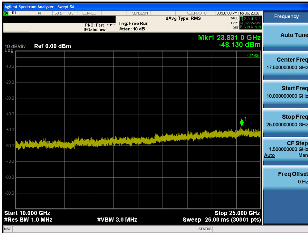
Plot 7-22. Conducted Spurious Plot (Bluetooth (LE), ePA – Ch. 39)
