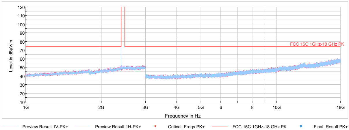
Plot 7-23. Radiated Spurious Plot above 1GHz (GFSK ePA – Ch. 0, Ant. Pol. H & V)
