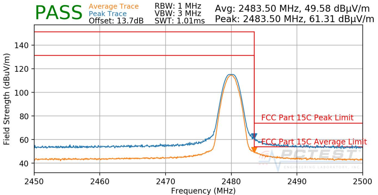
Plot 7-31. Radiated Restricted Upper Band Edge Measurement (Average & Peak)
