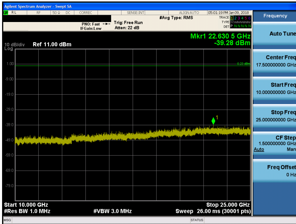
Plot 7-20. Conducted Spurious Plot (Bluetooth (LE), ePA – Ch. 19)
