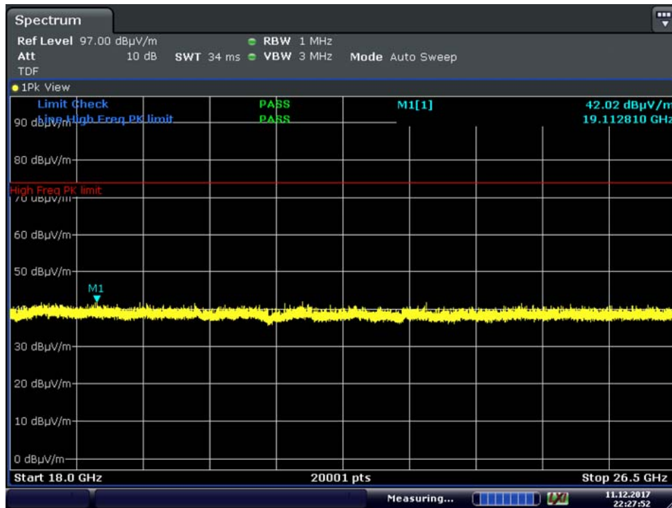
Plot 7-26. Radiated Spurious Plot above 18GHz (GFSK ePA, Pol. H)
