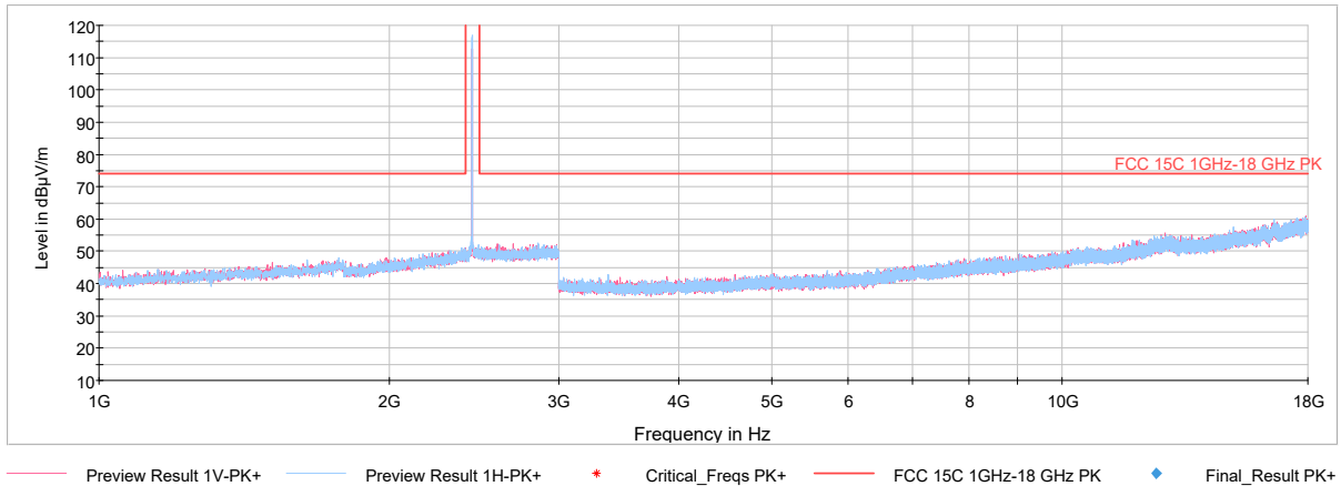
Plot 7-24. Radiated Spurious Plot above 1GHz (GFSK ePA – Ch. 19, Ant. Pol. H & V)
