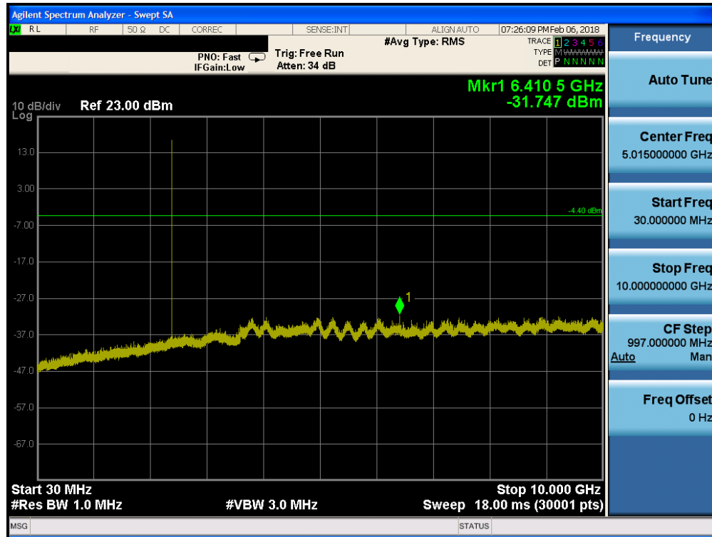
Plot 7-17. Conducted Spurious Plot (Bluetooth (LE), ePA – Ch. 0)
