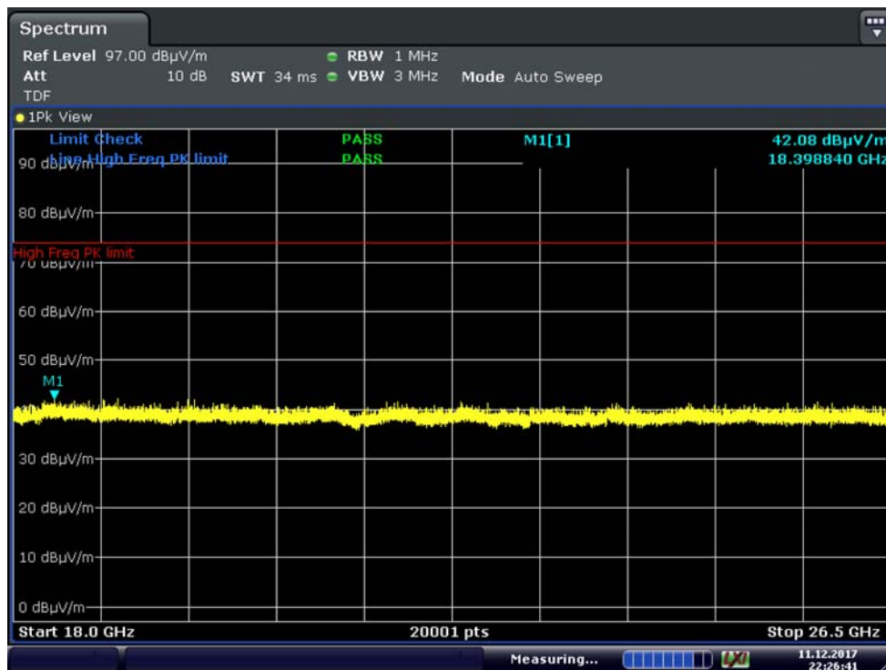
Plot 7-27. Radiated Spurious Plot above 18GHz (GFSK ePA, Pol. V)
