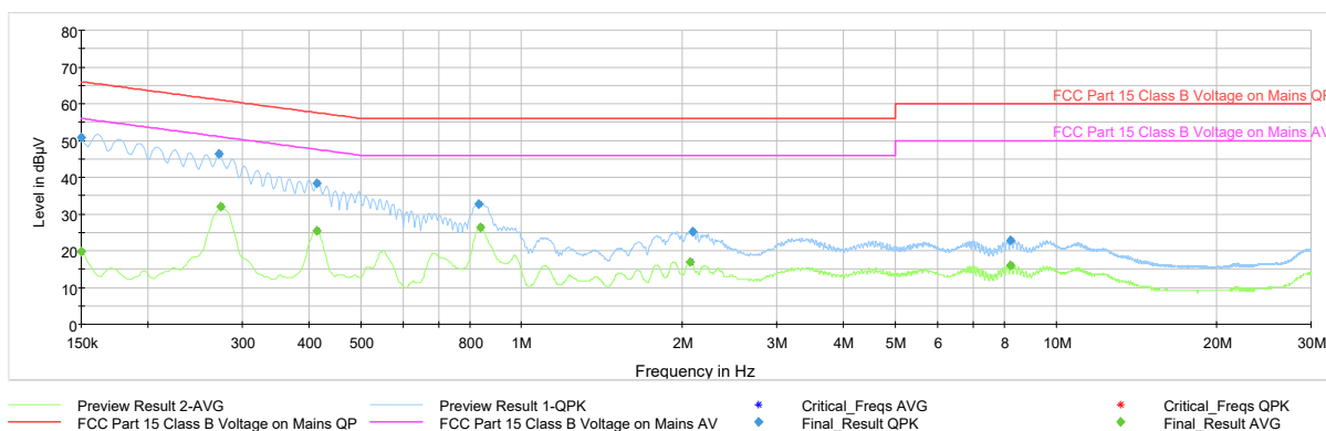
Plot 7-33. Line Conducted Plot with Bluetooth LE (GFSK ePA, L1)
