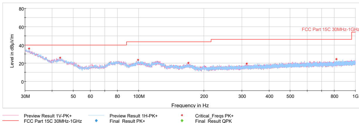
Plot 7-32. Radiated Spurious Plot below 1GHz (GFSK ePA, Pol. H & V)
