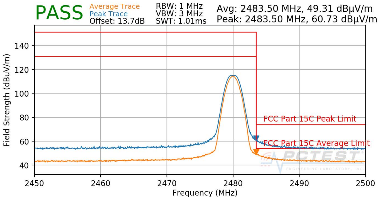
Plot 7-30. Radiated Restricted Upper Band Edge Measurement (Average & Peak)
