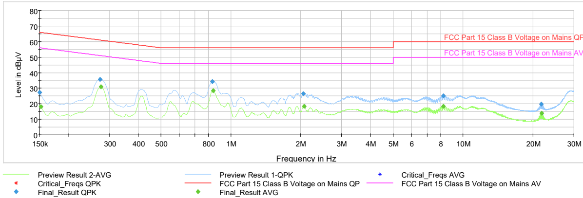
Plot 7-34. Line Conducted Plot with Bluetooth LE (GFSK ePA, N)
