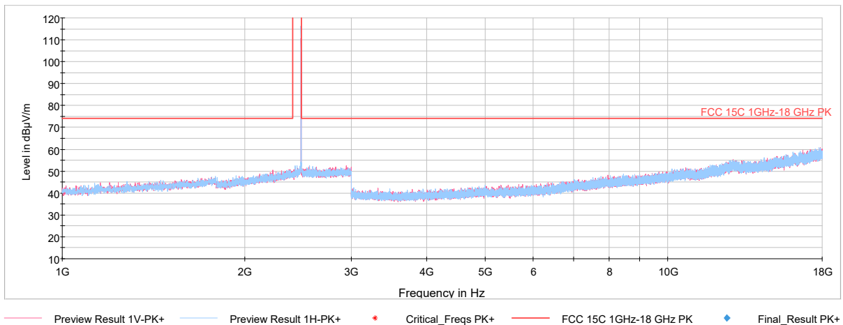
Plot 7-25. Radiated Spurious Plot above 1GHz (GFSK ePA – Ch. 39, Ant. Pol. H & V)
