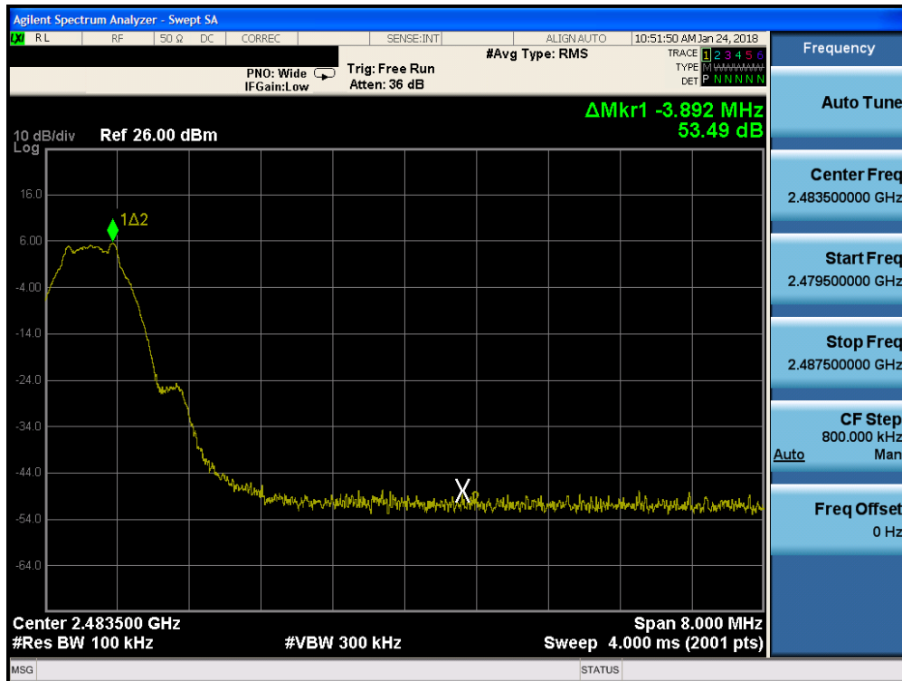
Plot 7-16. Band Edge Plot (Bluetooth (LE), iPa – Ch. 39)
