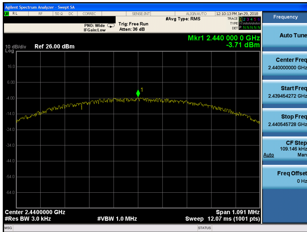
Plot 7-8. Power Spectral Density Plot (Bluetooth (LE), ePA – Ch. 19)
