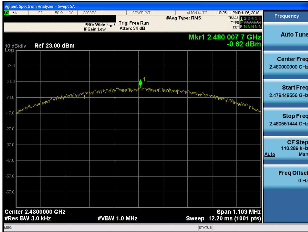
Plot 7-9. Power Spectral Density Plot (Bluetooth (LE), ePA – Ch. 39)
