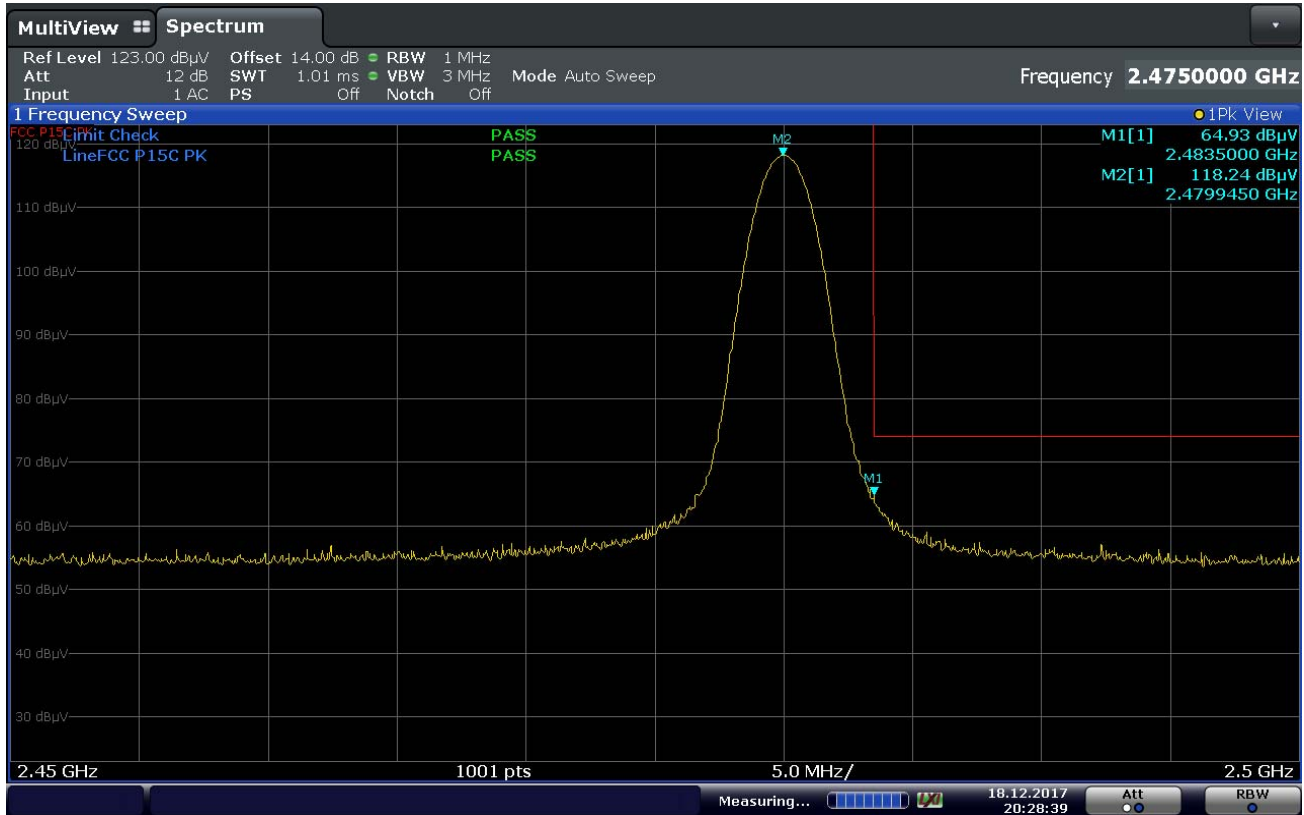
Plot 7-78. Radiated Restricted Upper Band Edge Measurement (Peak)
