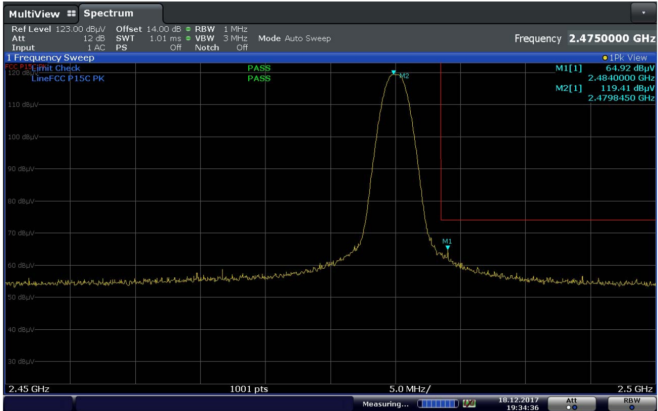
Plot 7-76. Radiated Restricted Upper Band Edge Measurement (Peak)
