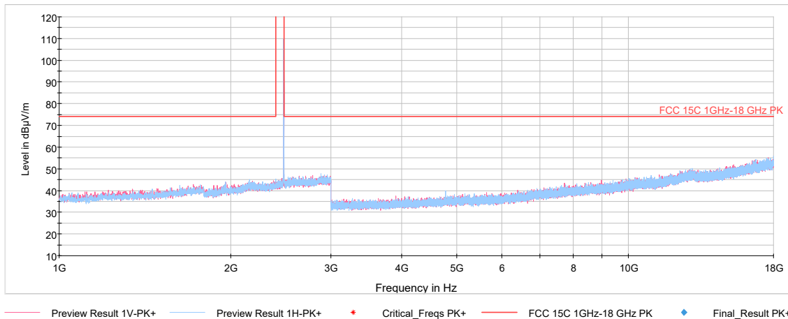
Plot 7-63. Radiated Spurious Plot above 1GHz (BT GFSK ePA – Ch. 78, Ant. Pol. H & V)
