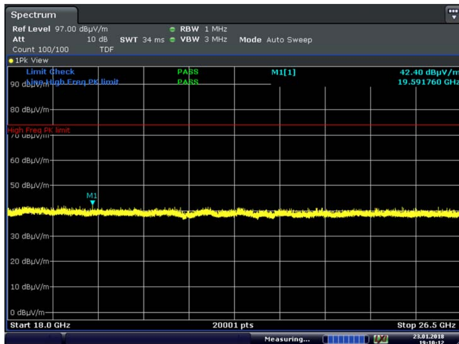
Plot 7-68. Radiated Spurious Plot 18GHz – 26.5GHz (2.4GHz – 5GHz, Ant. Pol. V)
