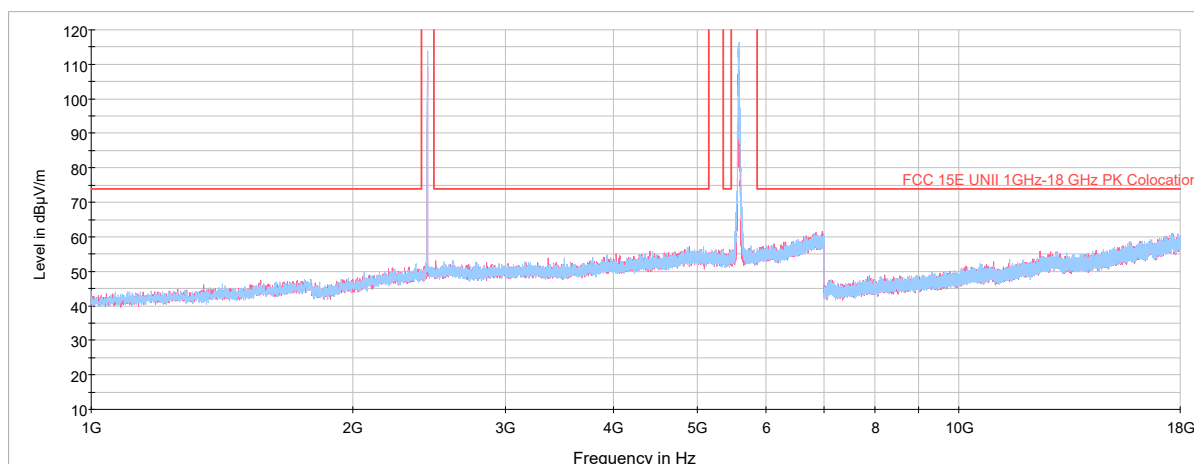
Plot 7-66. Radiated Spurious Plot above 1GHz (2.4GHz – 5GHz, Ant. Pol. H & V)
