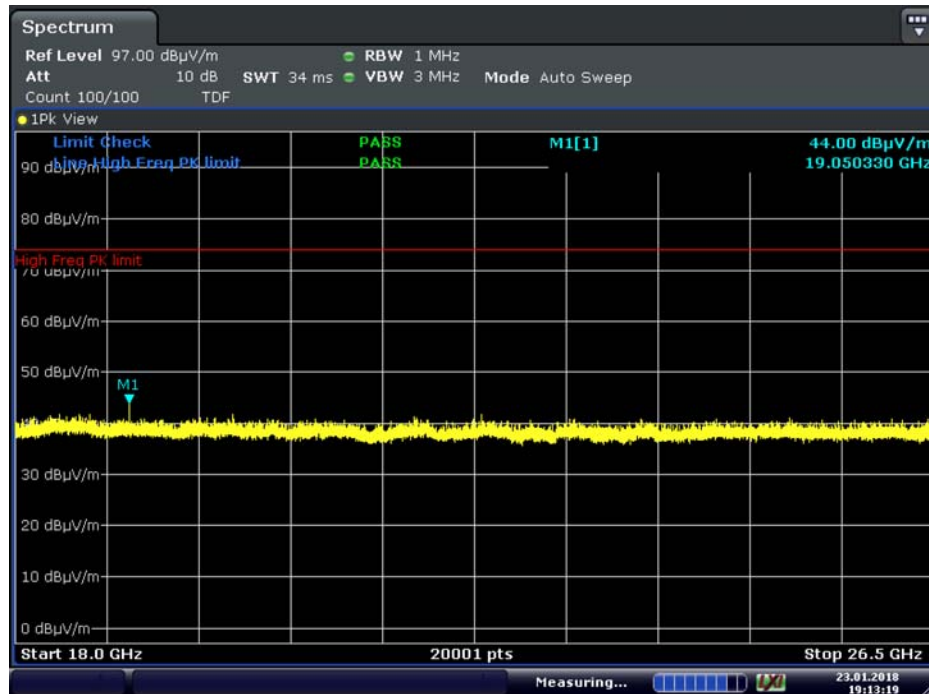
Plot 7-67. Radiated Spurious Plot 18GHz – 26.5GHz (2.4GHz – 5GHz, Ant. Pol. H)
