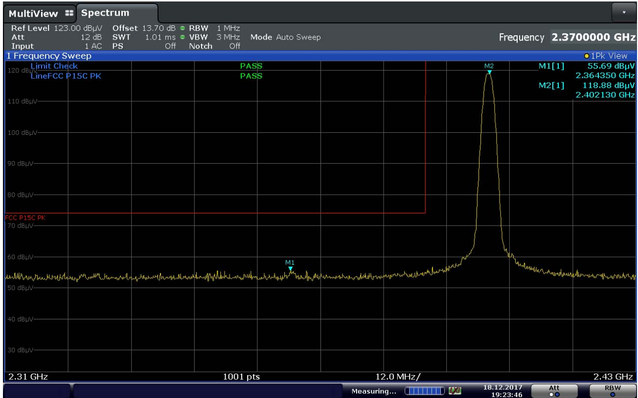
Plot 7-72. Radiated Restricted Lower Band Edge Measurement (Peak)
