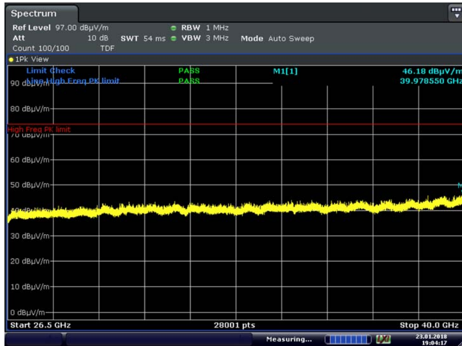
Plot 7-69. Radiated Spurious Plot above 26.5GHz (2.4GHz – 5GHz, Ant. Pol. H)
