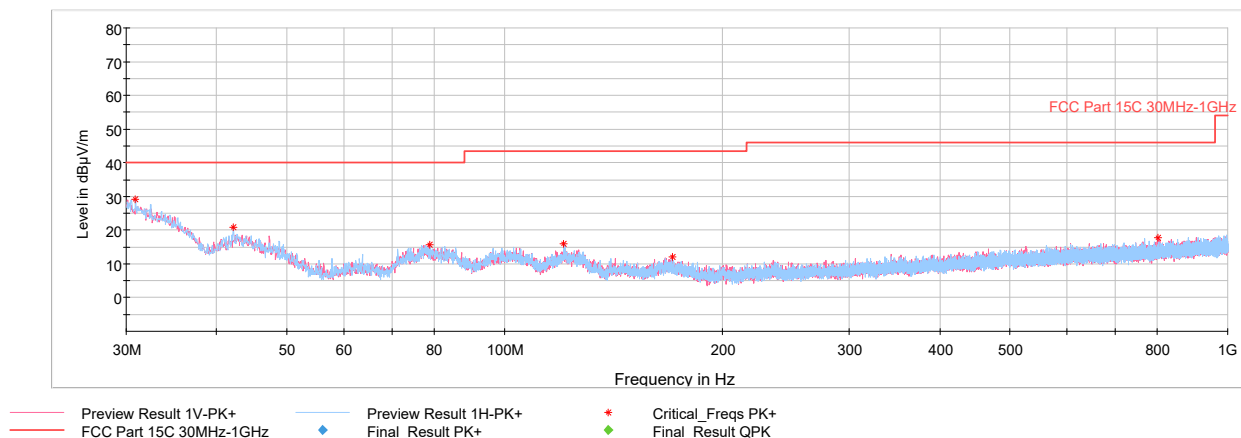
Plot 7-79. Radiated Spurious Plot below 1GHz (GFSK ePA, Pol. H & V)
