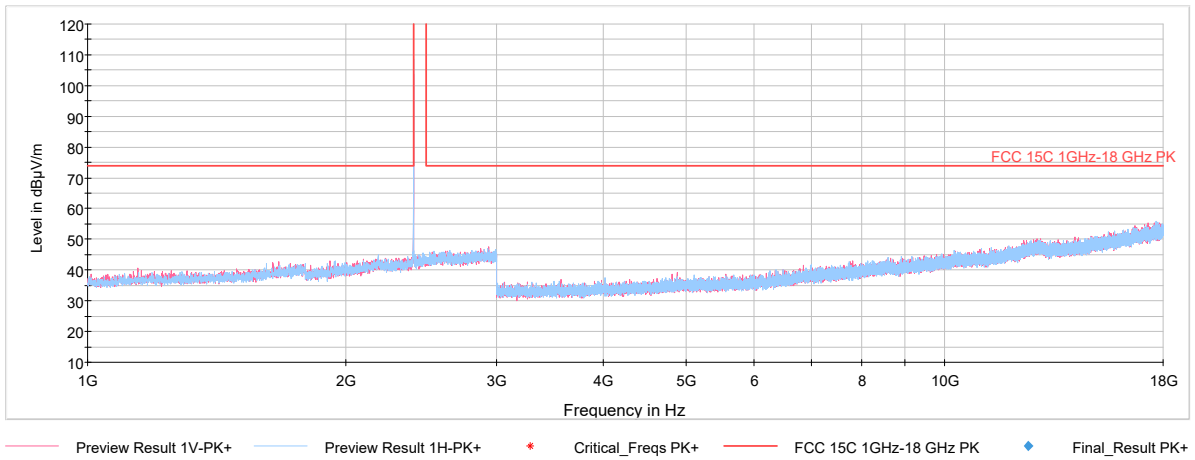
Plot 7-61. Radiated Spurious Plot above 1GHz (BT GFSK ePA – Ch. 0, Ant. Pol. H & V)
