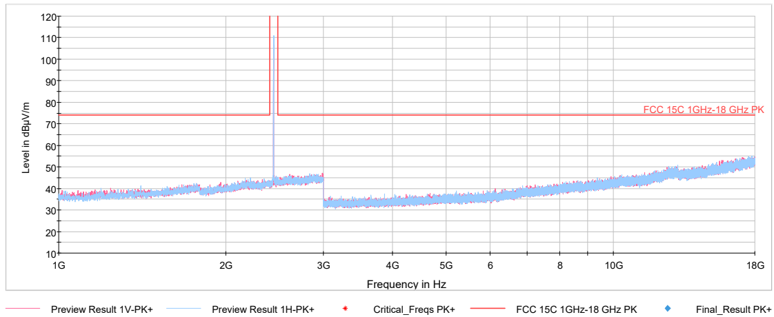
Plot 7-62. Radiated Spurious Plot above 1GHz (BT GFSK ePA – Ch. 39, Ant. Pol. H & V)
