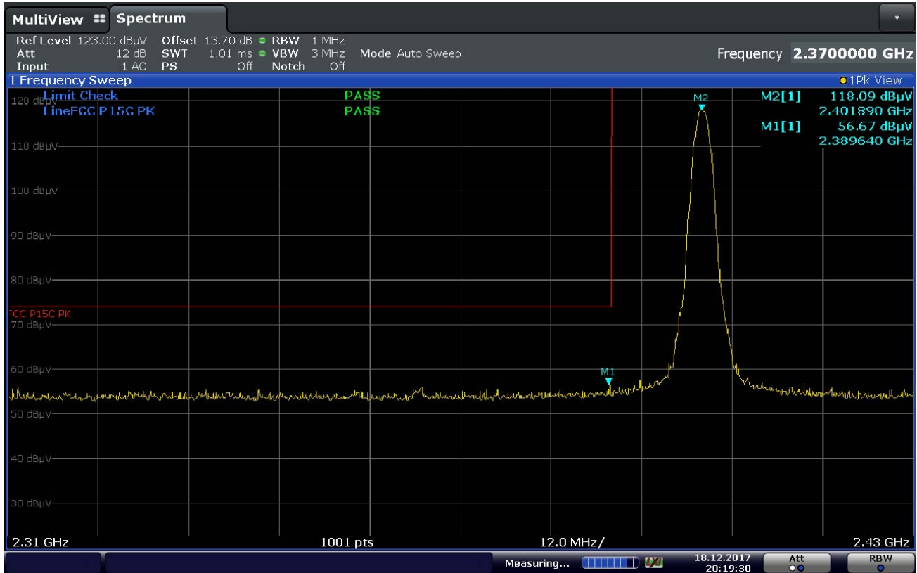
Plot 7-74. Radiated Restricted Lower Band Edge Measurement (Peak)
