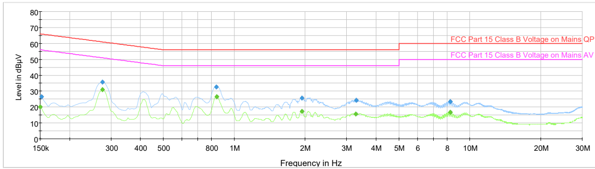
Plot 7-80. Line-Conducted Test Plot (L1)
