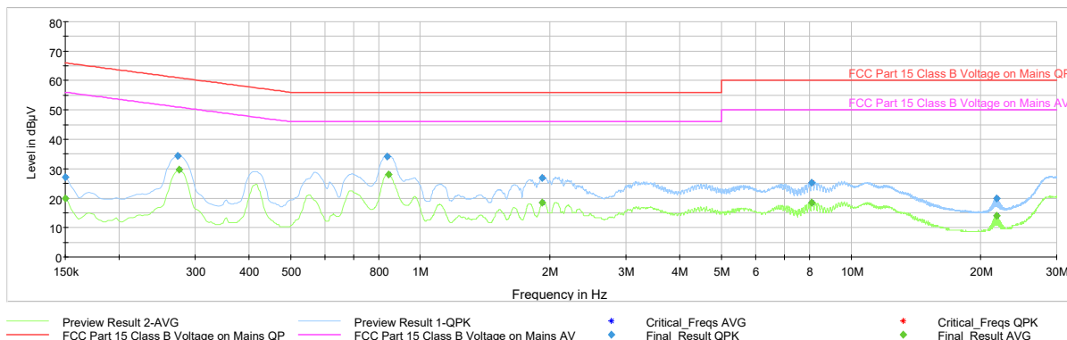
Plot 7-81. Line-Conducted Test Plot (N)
