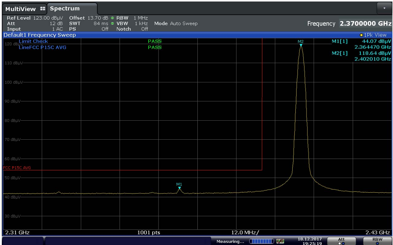
Plot 7-71. Radiated Restricted Lower Band Edge Measurement (Average)
