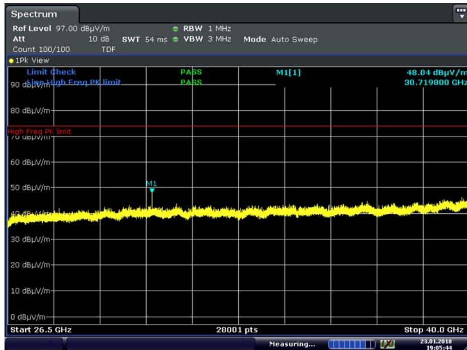
Plot 7-70. Radiated Spurious Plot above 26.5GHz (2.4GHz – 5GHz, Ant. Pol. V)
