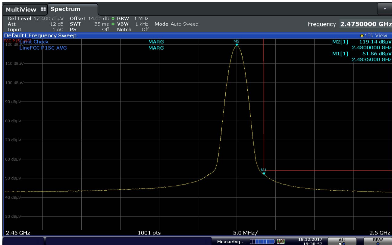
Plot 7-75. Radiated Restricted Upper Band Edge Measurement (Average)
