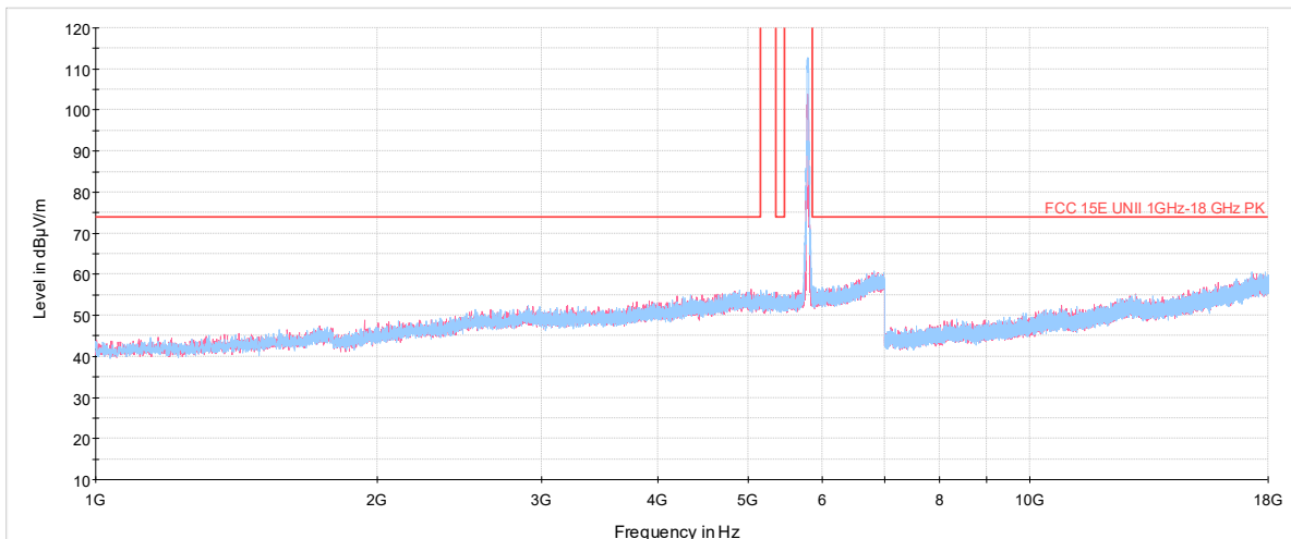
Plot 7-288. Radiated Spurious Plot above 1GHz SISO ANT2 (802.11a – U3 Ch. 157, Ant. Pol. H & V)
