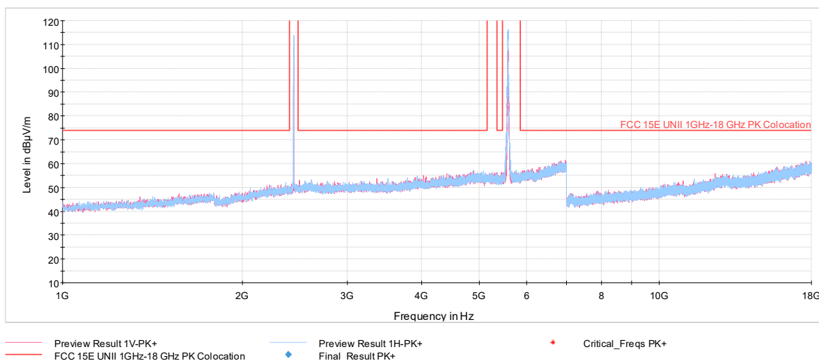
Plot 7-293. Radiated Spurious Plot above 1GHz Simultaneous Tx (2.4GHz – 5GHz, Ant. Pol. H & V)
